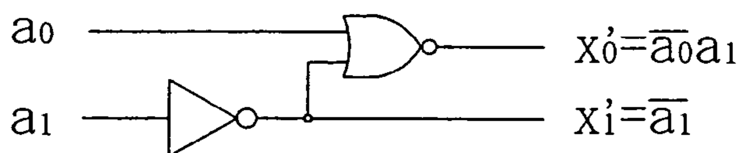
FIG. 5B DUMMY CIRCUIT f 1
