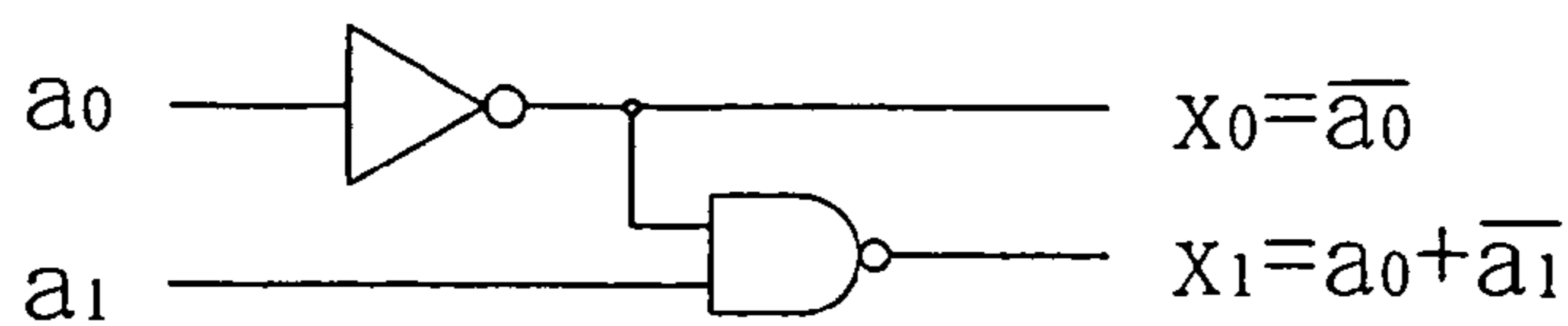
FIG. 5A ORIGINAL CIRCUIT f 0
