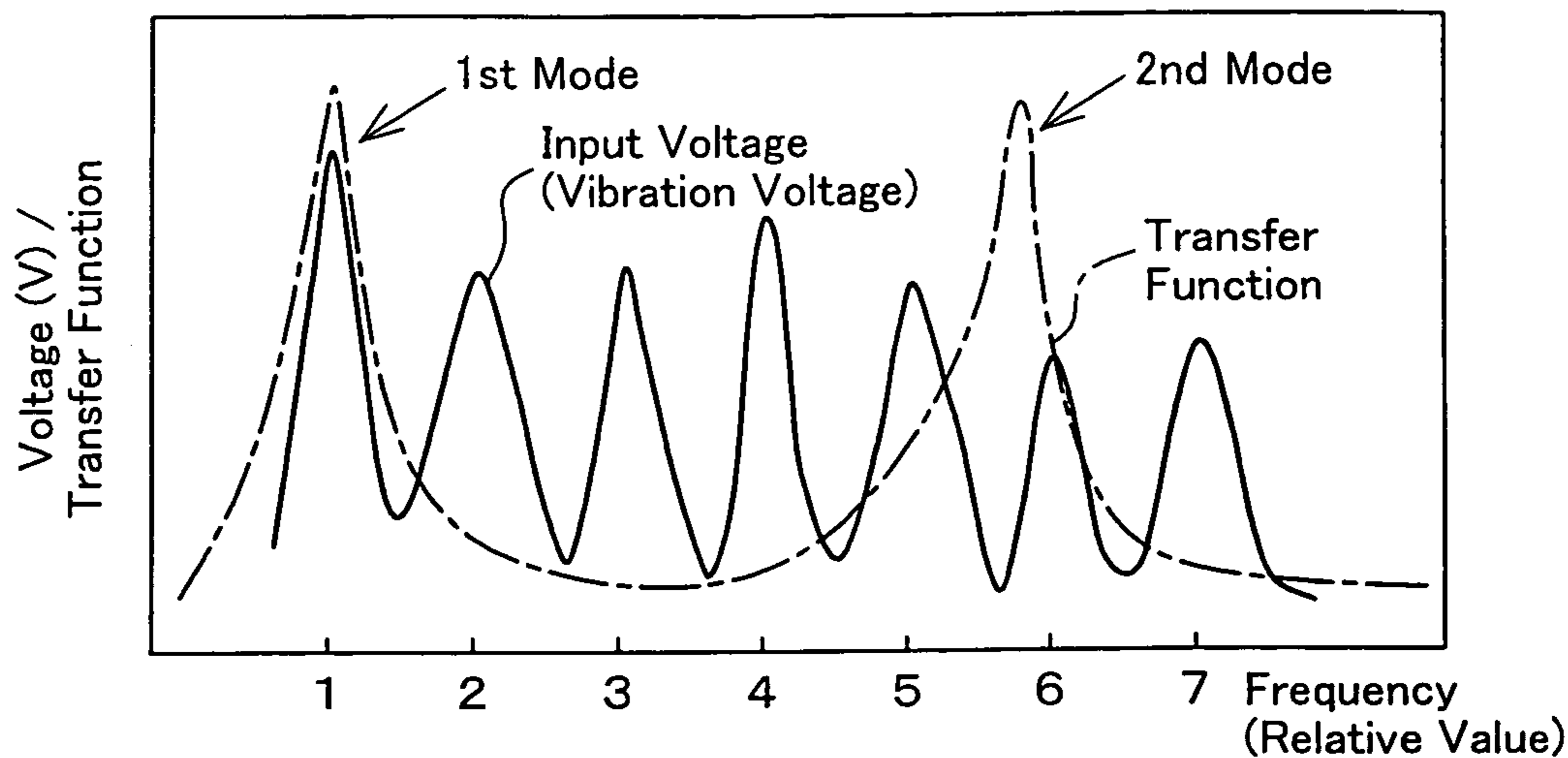
Vibration Voltage and Transfer Function of Sensor in Frequency Domain
