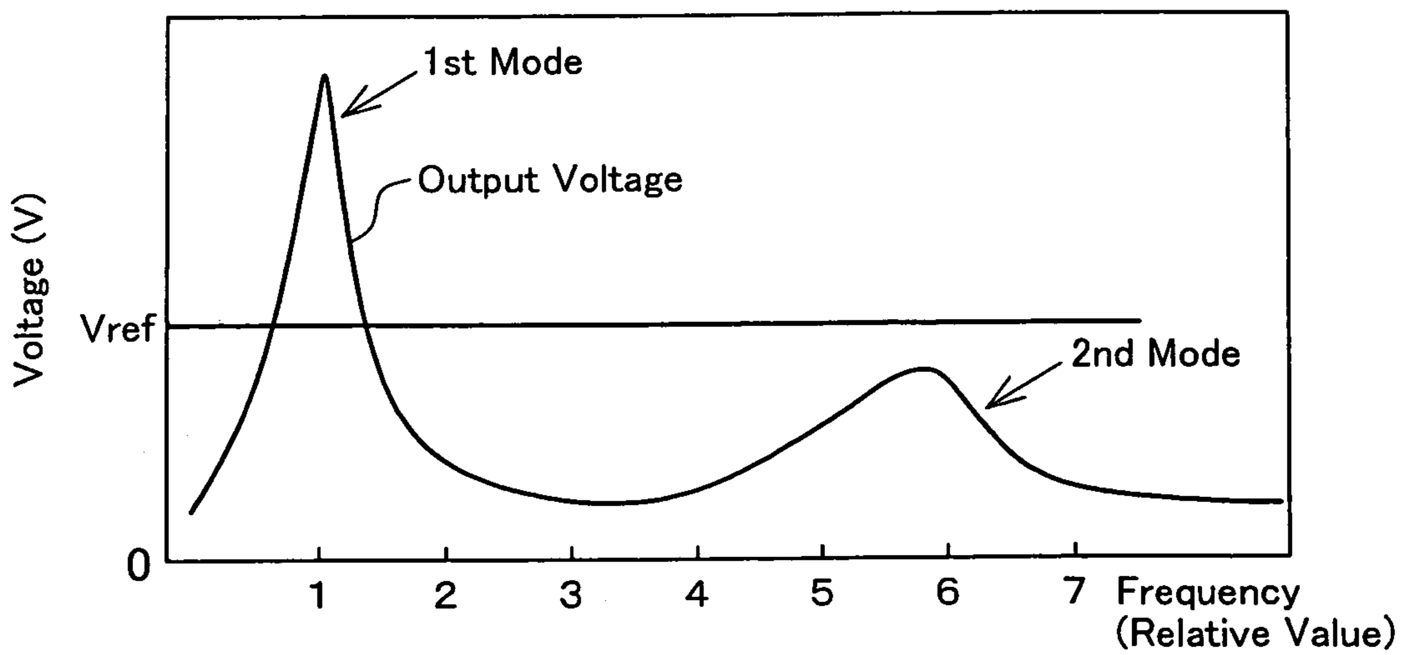
Output Voltage of Sensor in Frequency Domain
