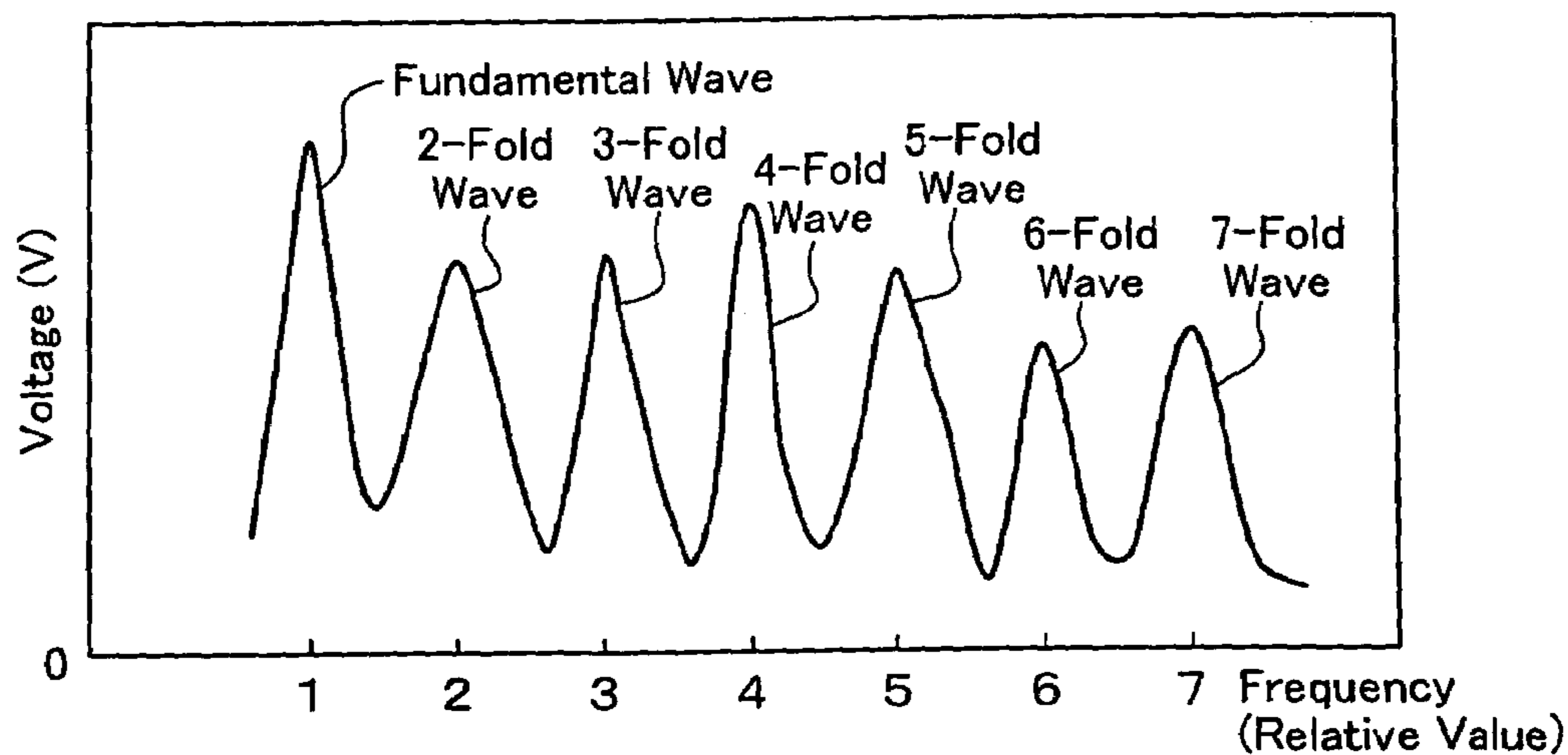
Applied Voltage of Piezoelectric Element in Frequency Domain
