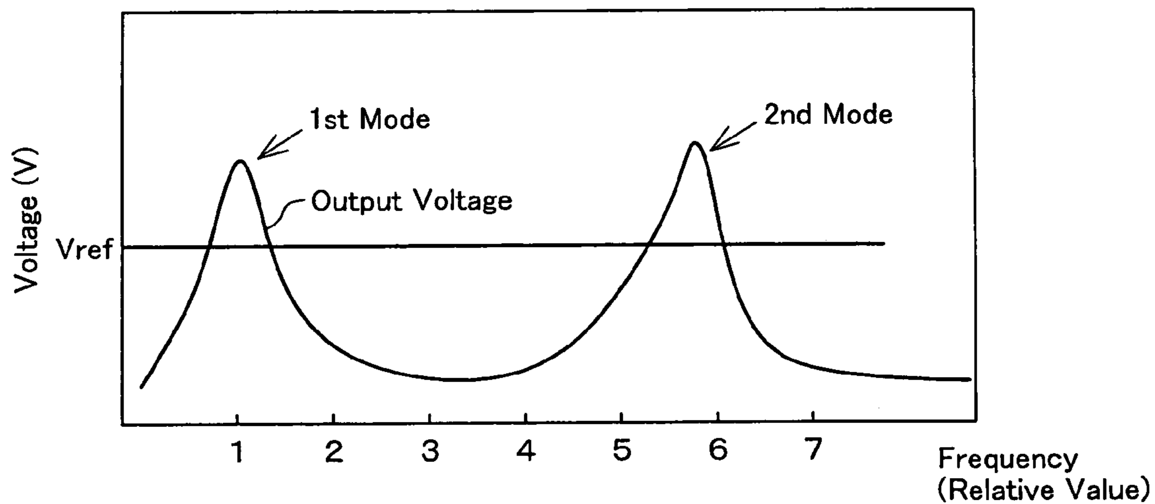
Output Voltage of Sensor in Frequency Domain
