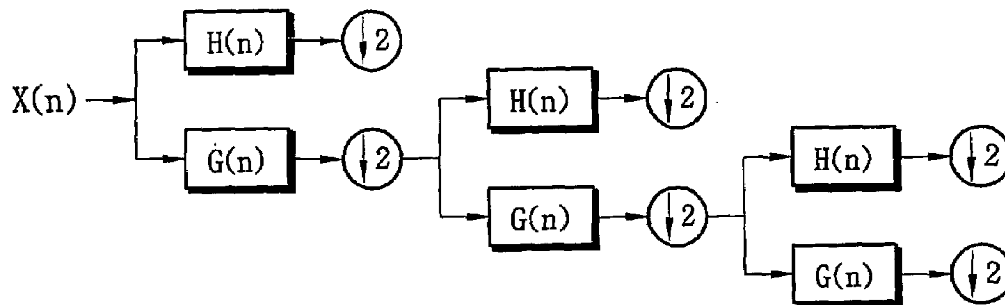
DISCRETE WAVELET TRANSFORM BY A FILTER BANK
