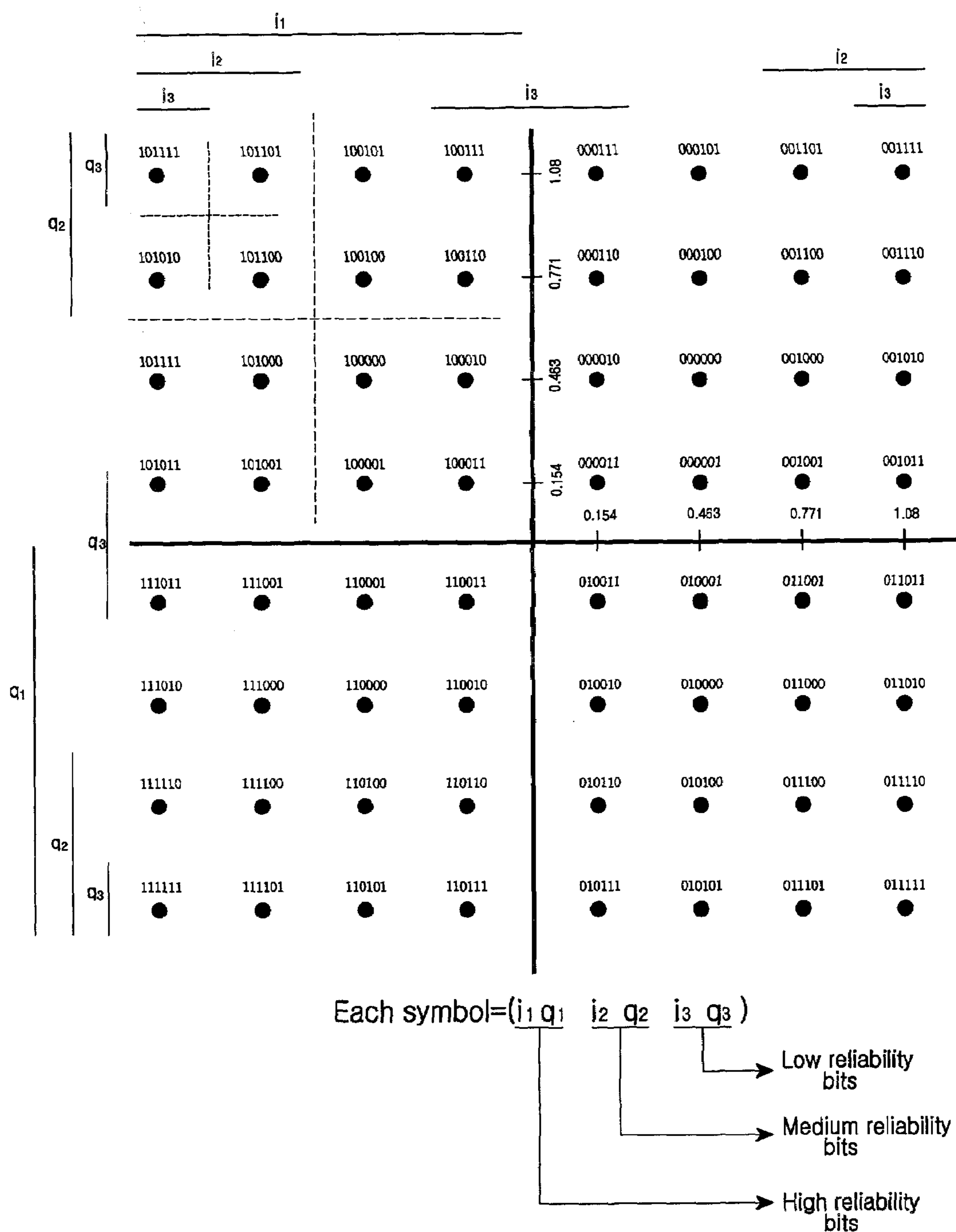
FIG.3 (PRIOR ART)
