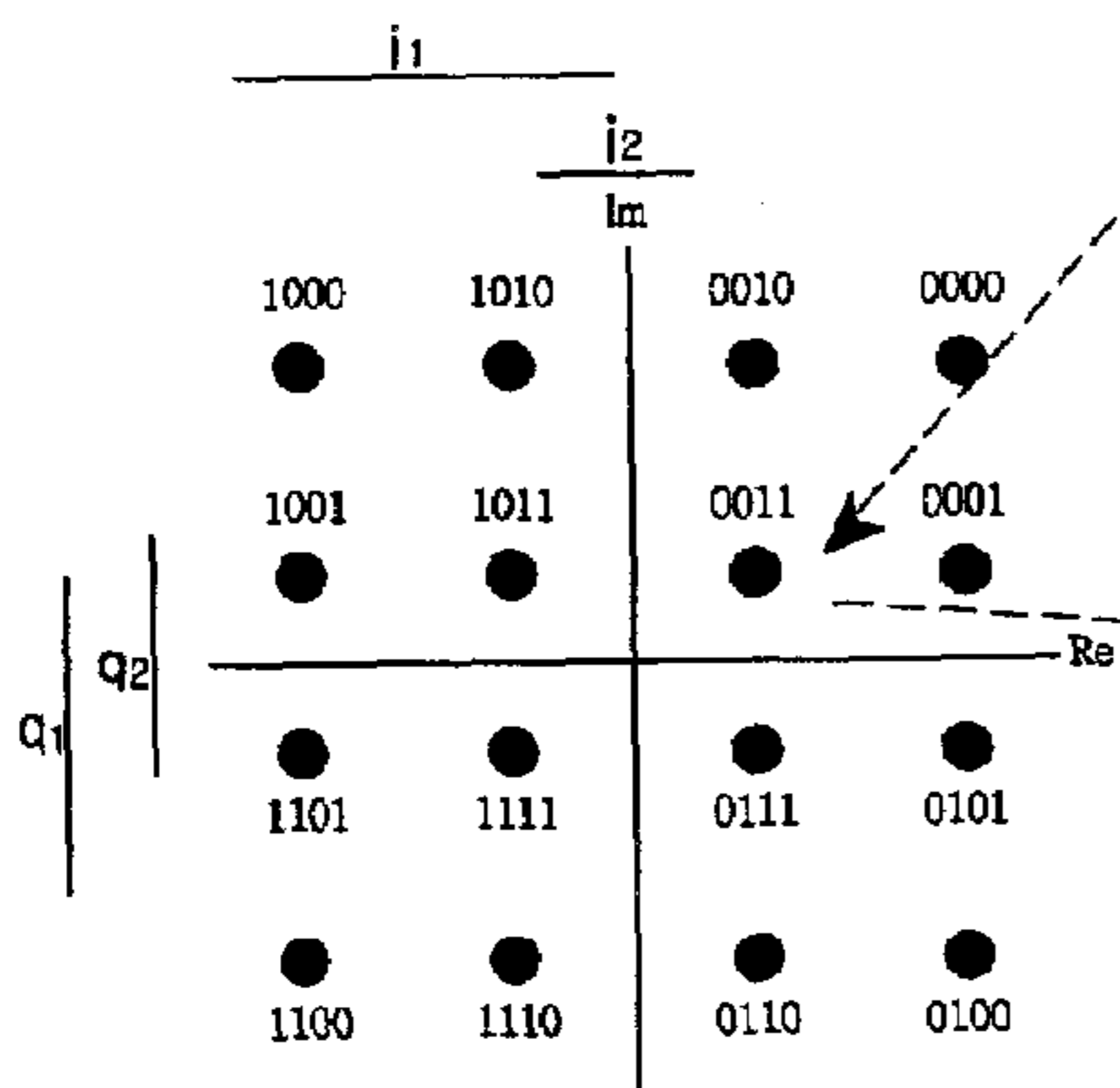
FIG. 7C (PRIOR ART)
