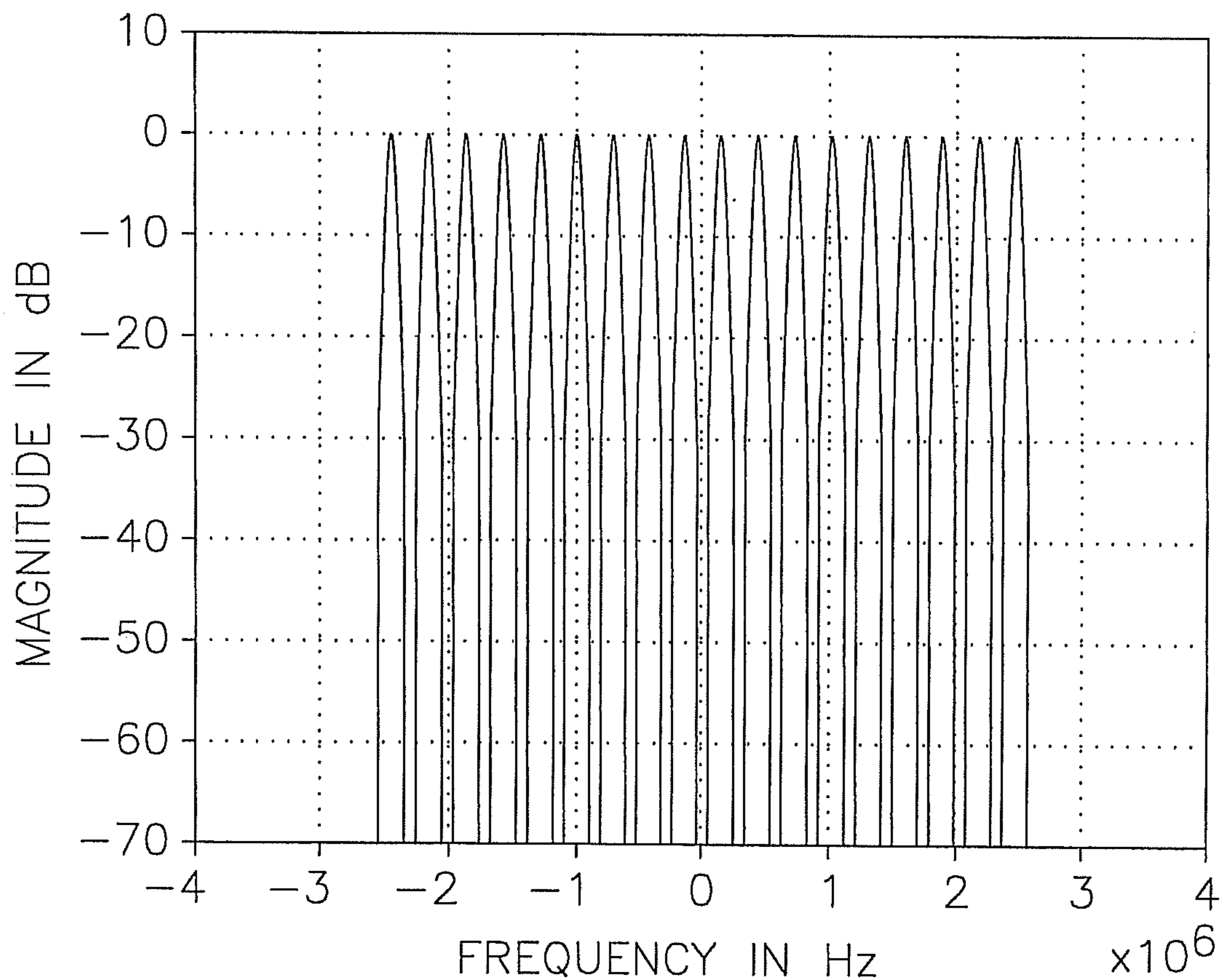
Magnitude response of a single polyphase filter bank
