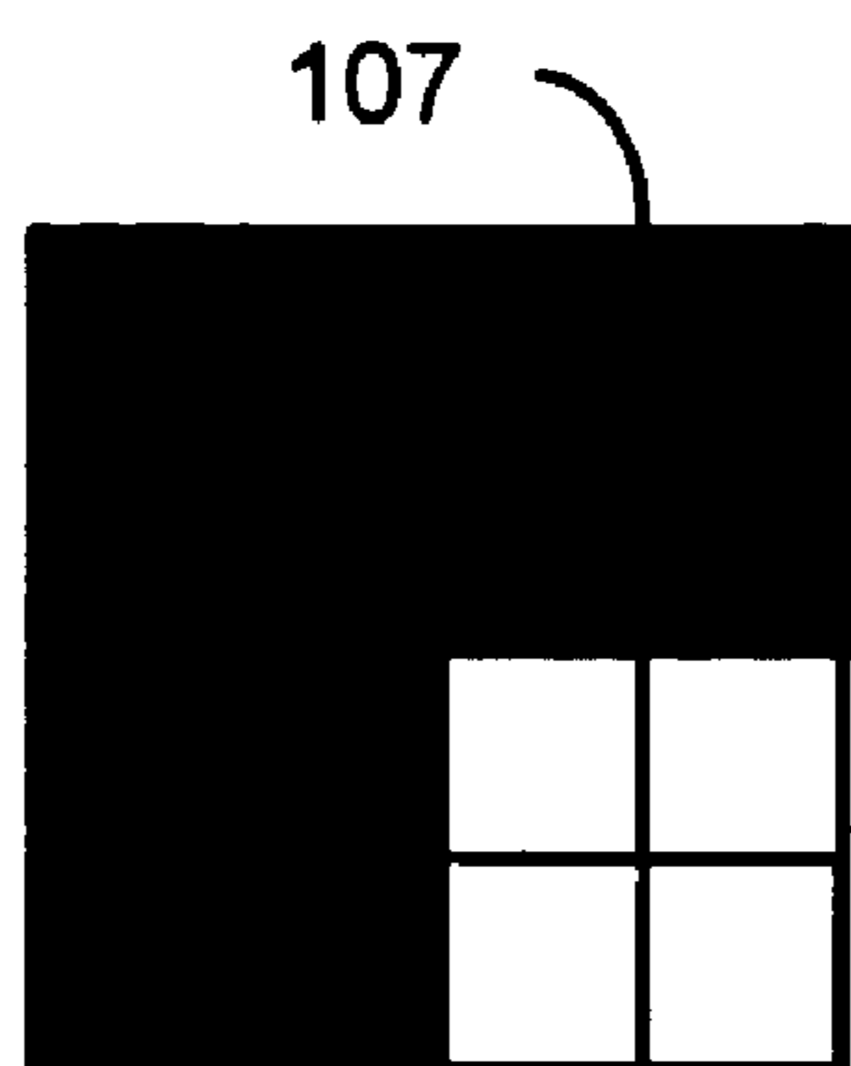
coverage
