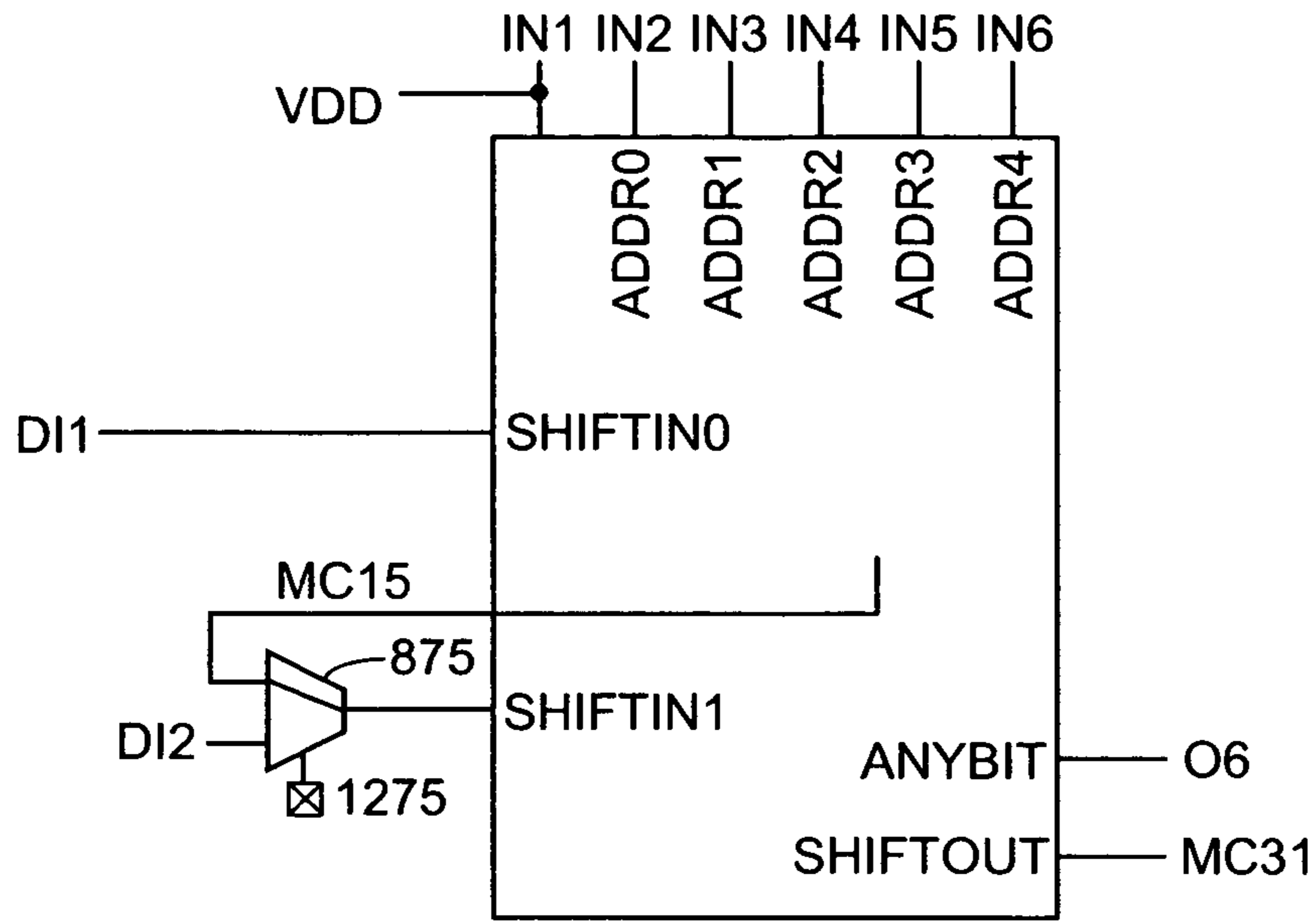
FIG. 12 (32x1 SRL)
