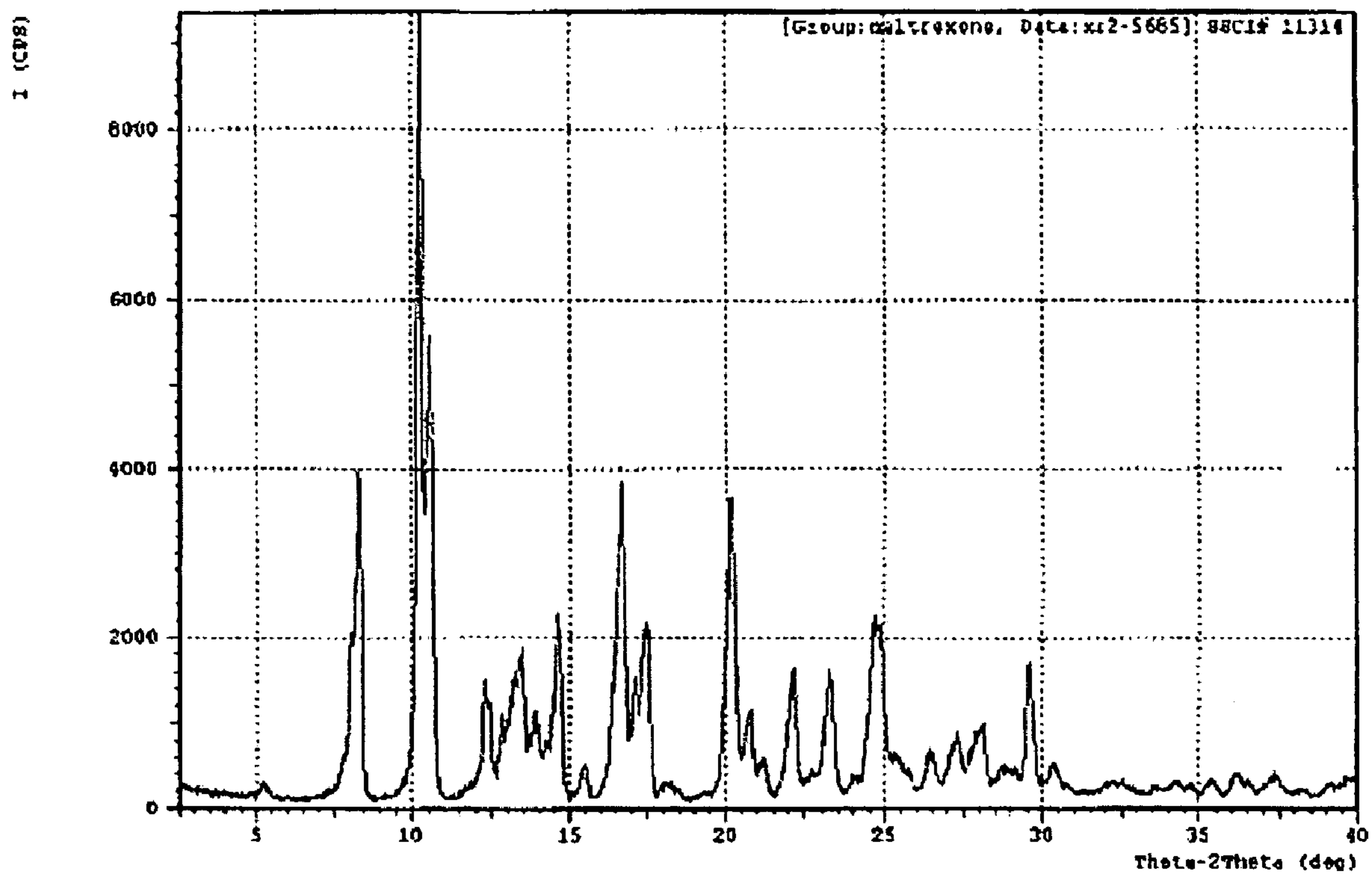
Figure 7. XRPD pattern of naltrexone lot 00-119-095 G (SSCI number 11314).
