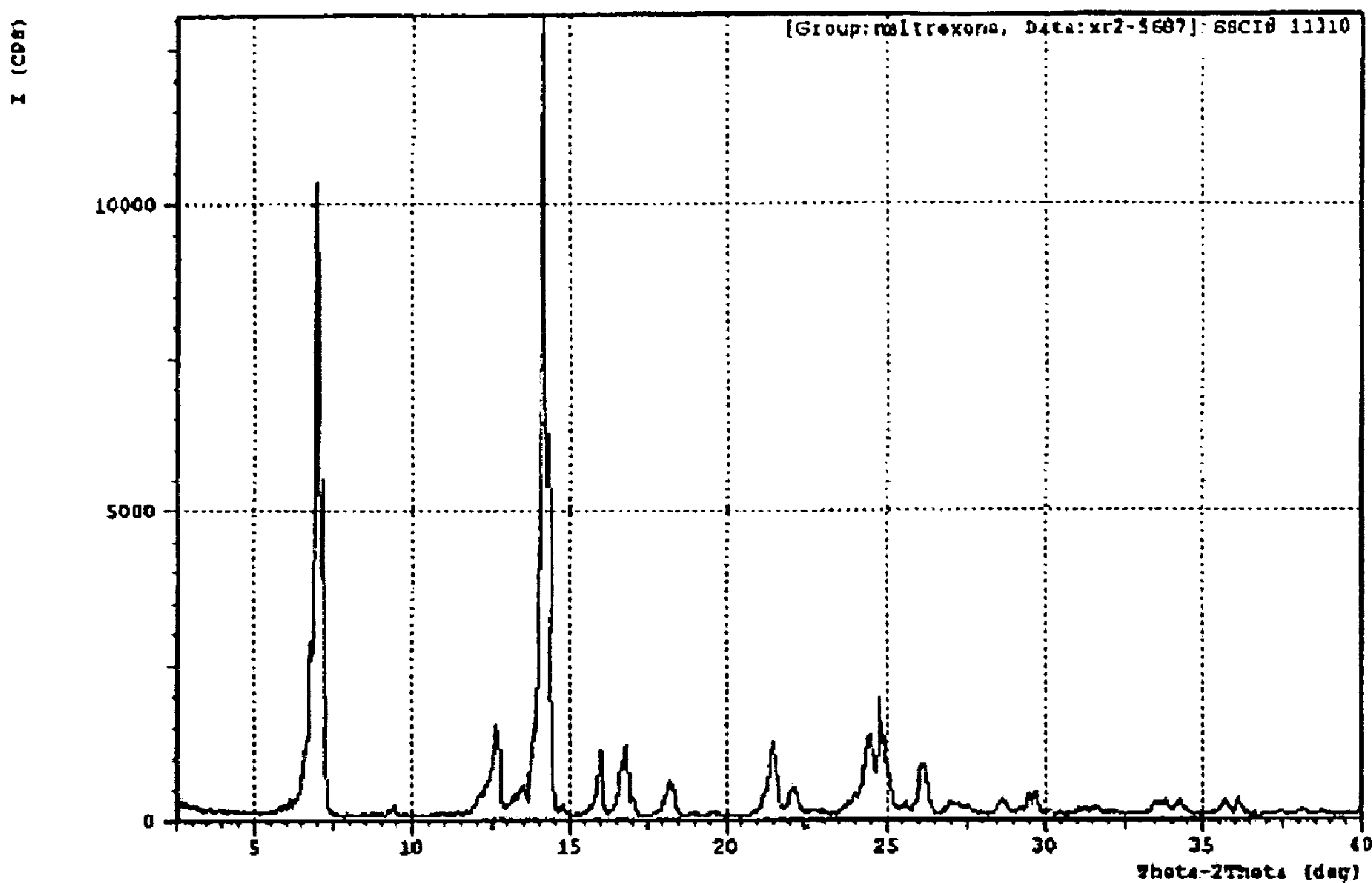
Figure 3. XRPD pattern of naltrexone lot 00-119-093 C (SSCI number 11310).
