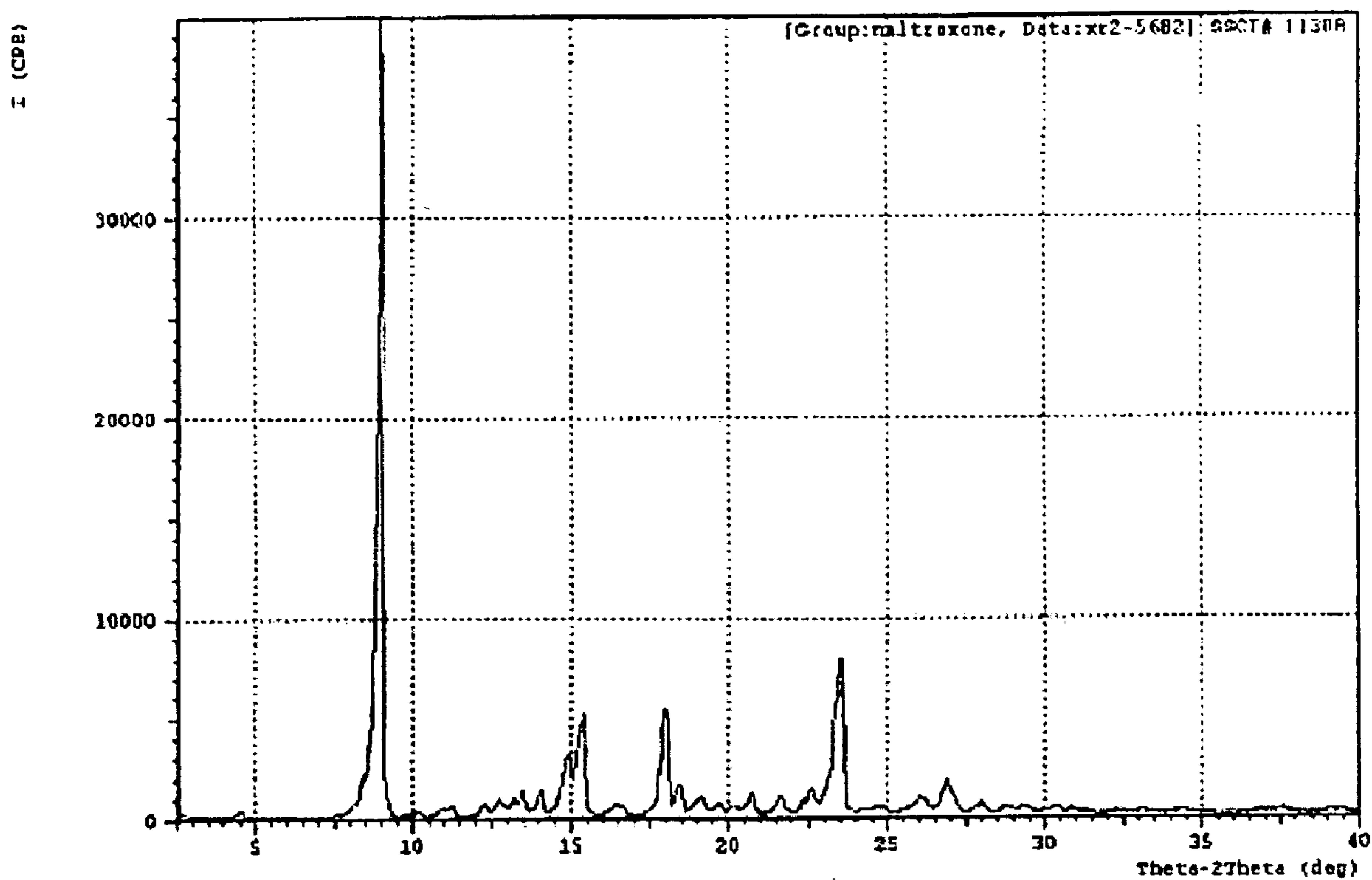
Figure 1. XRPD pattern of naloxone lot 00-119-095A (SSCI number 11308).
