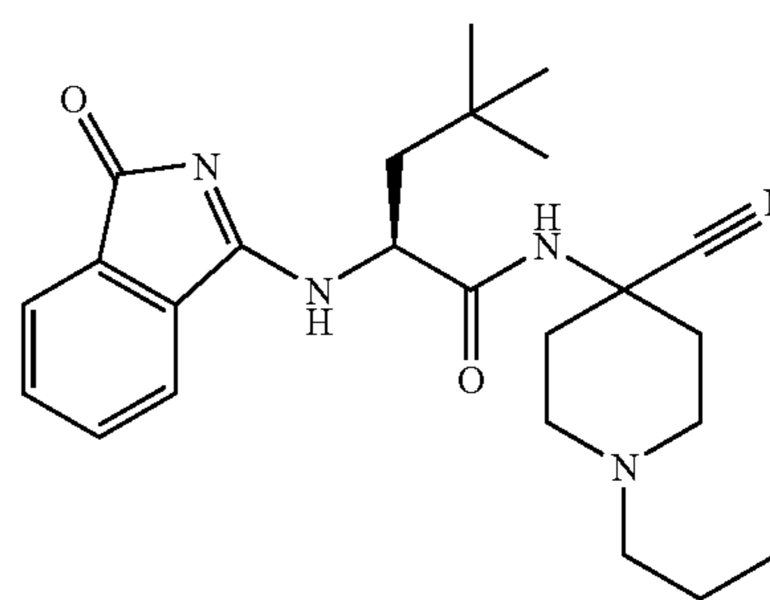
4,4-Dimethyl-2-(3-oxo-3 H-isoindol-1-ylamino)-pentanoic acid-(4-cyano-1-propyl-piperidin-4-yl)-amide
