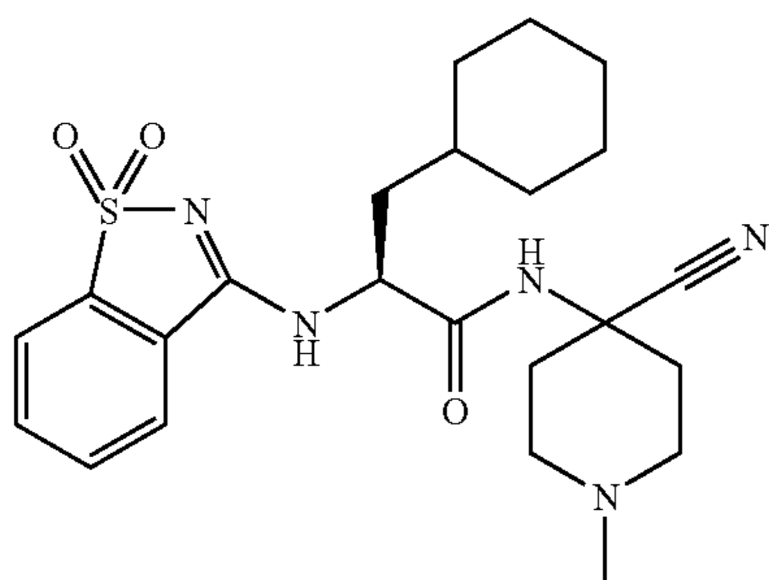
N-(4-Cyano-1-methyl-piperidin-4-yl)-3-cyclohexyl-2-(1,1-dioxo-1H-λ 6 -benzo[d]isothiazol-3-ylamino)-propionamide (Method G)
