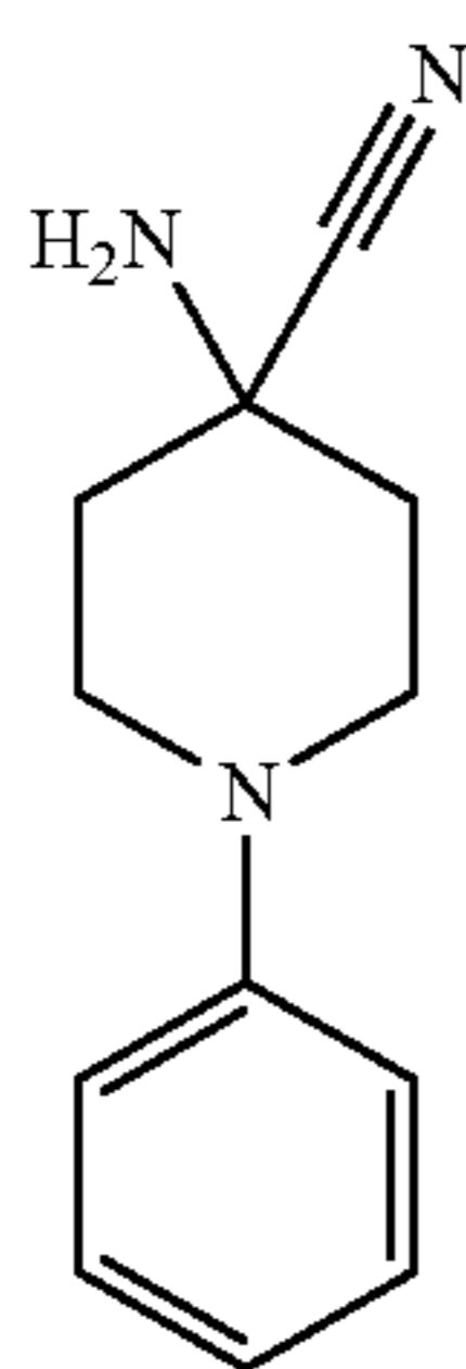
(b) 4-Amino-4-cyano-1-phenyl-piperidine
