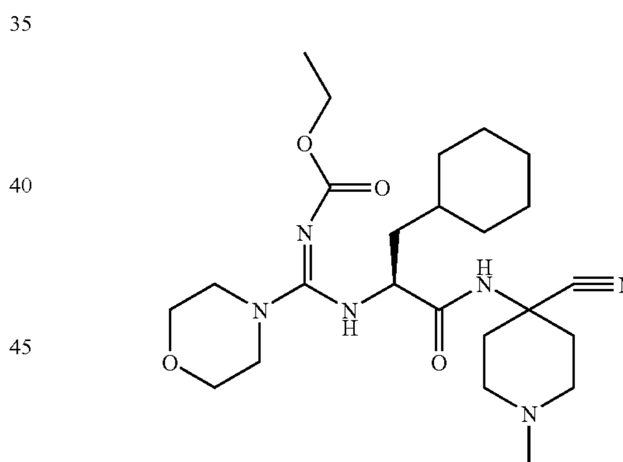
{[1-(4-Cyano-1-methyl-piperidin-4-yl)carbamoyl]-2-cyclohexyl-ethylamino]-morpholin-4-yl-methylen]-carbamic acid ethyl ester (Method E)
