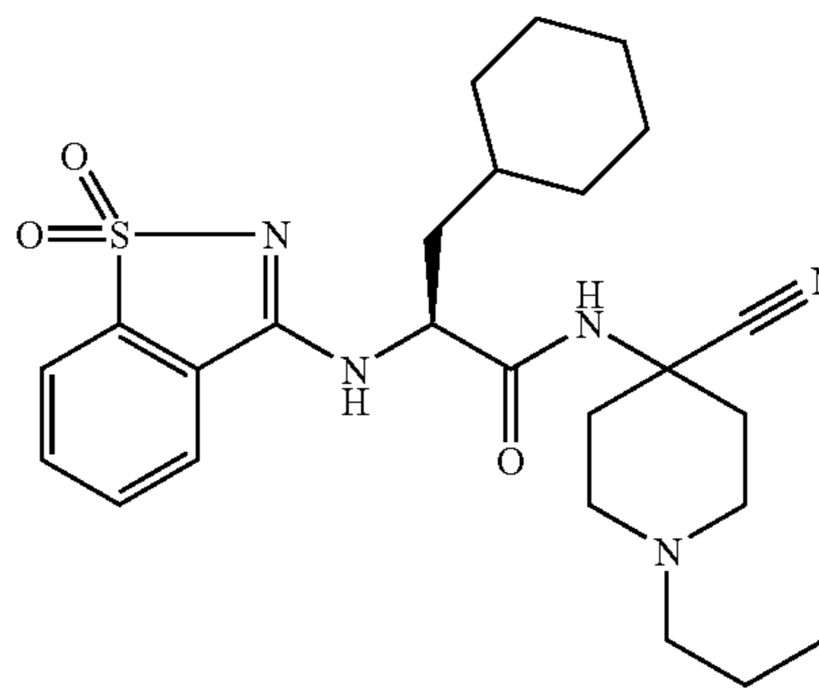
N-(4-Cyano-1-propyl-piperidin-4-yl)-3-cyclohexyl-2-(1,1-dioxo-1H-λ 6 -benzo[d]isothiazol-3-ylamino)-propionamide
