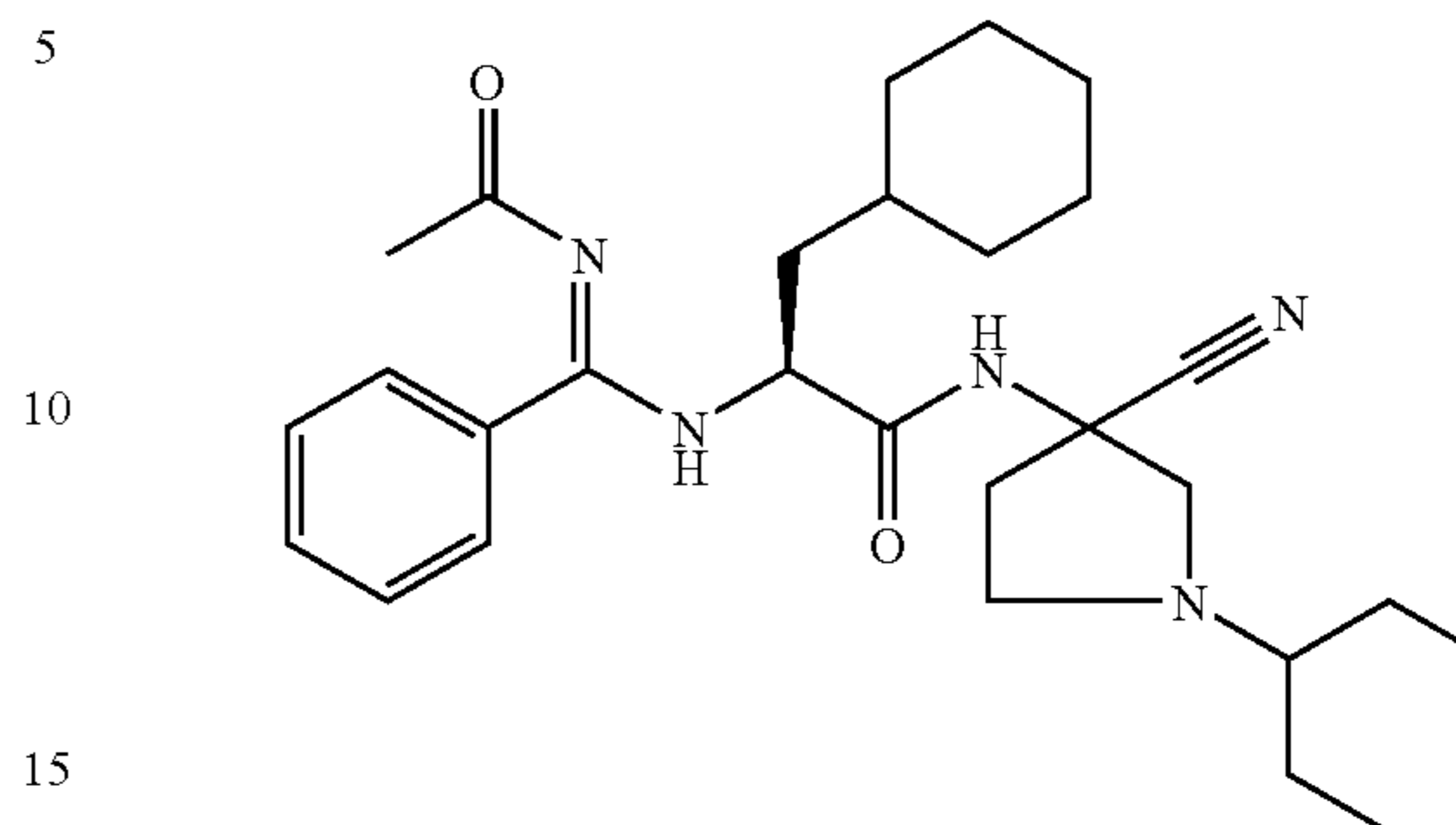
2-[(Acetylimino-phenyl-methyl)-amino]-N-[3-cyano-1-(1-ethyl-propyl)-pyrrolidin-3-yl]-3-cyclohexyl-propionamide
