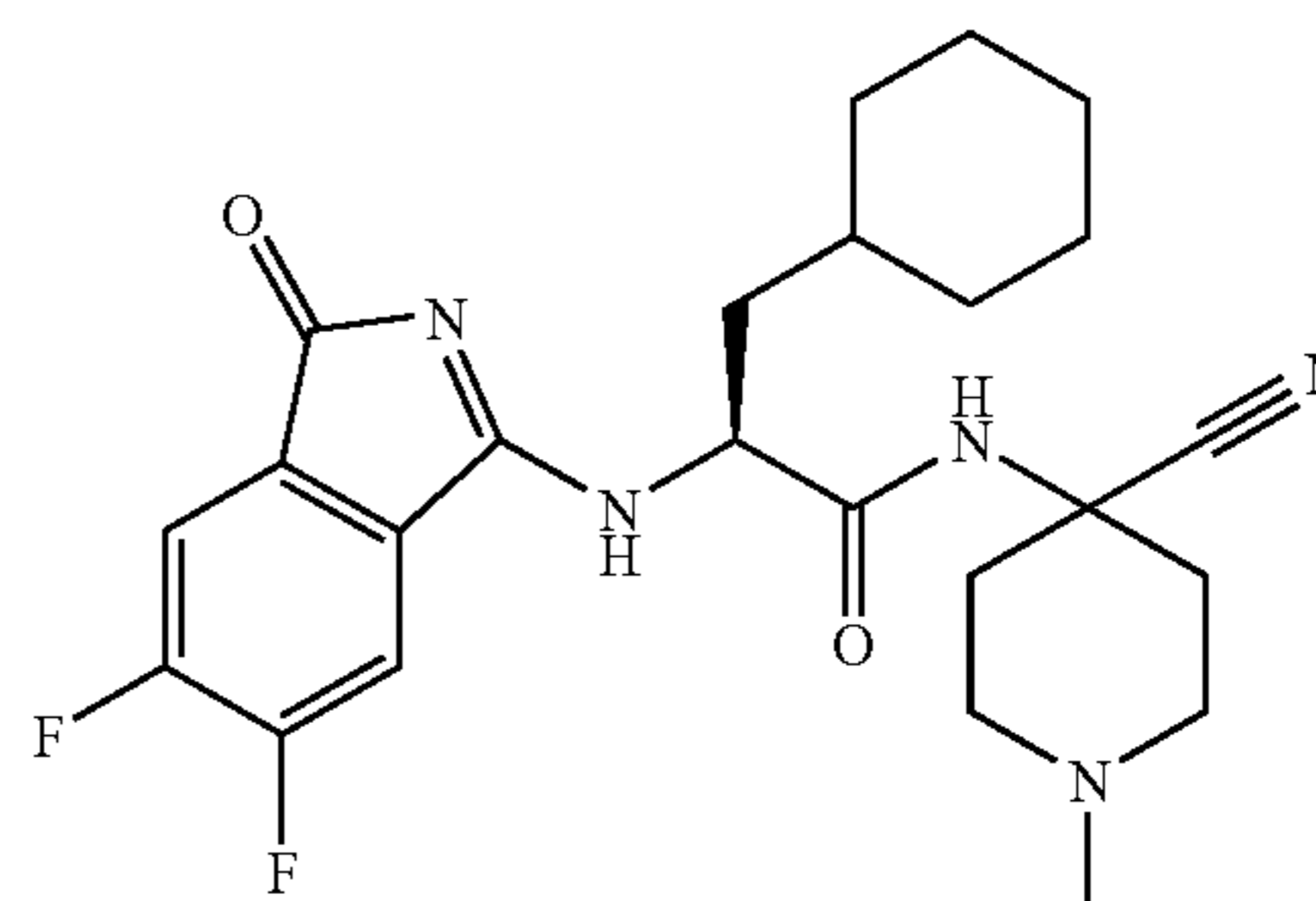
N-(4-cyano-1-methyl-piperidin-4-yl)-3-cyclohexyl-2-(5,6-difluoro-3-oxo-3H-isoindol-1-ylamino)propionamide
