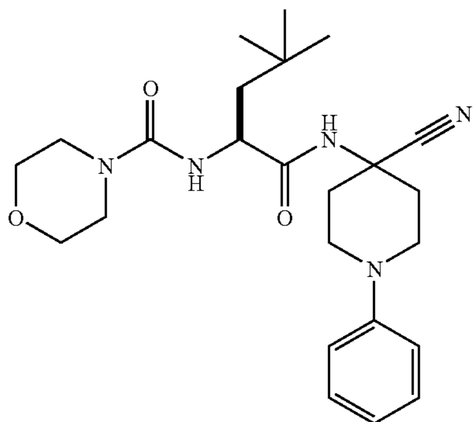
(c) Morpholine-4-carboxylic acid [1-(4-cyano-1-phenyl-piperidin-4-ylcarbonyl)-3,3-dimethyl-butyl]-amide
