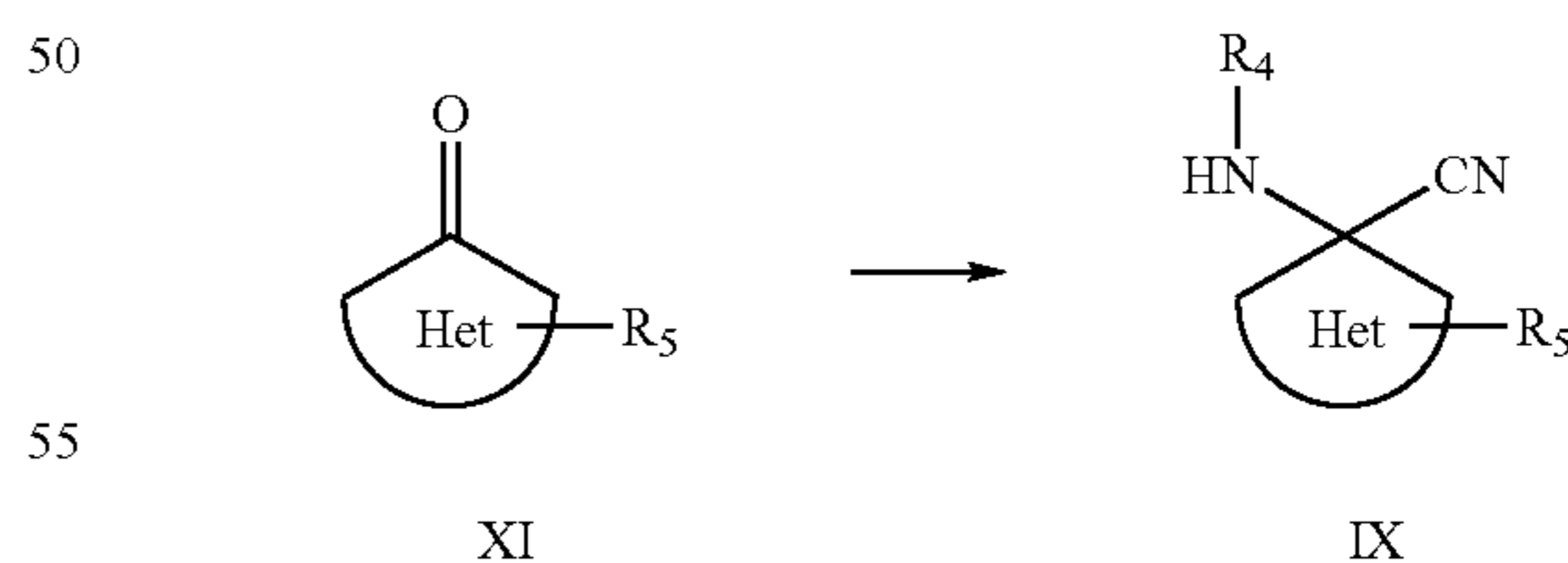
Scheme VII
