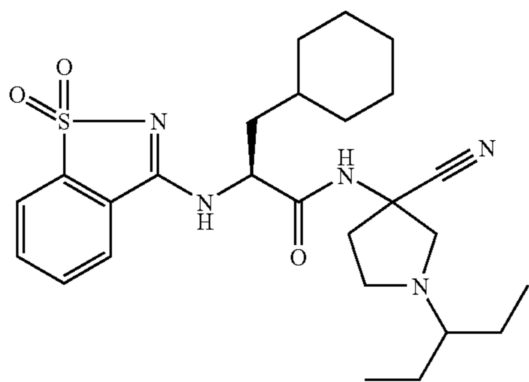
N-[3-Cyano-1-(1-ethyl-propyl)-pyrrolidin-3-yl]-3-cyclohexyl-2-(1,1-dioxo-1H-1λ 6 -benzo]isothiazol-3-ylamino)-propionamide
