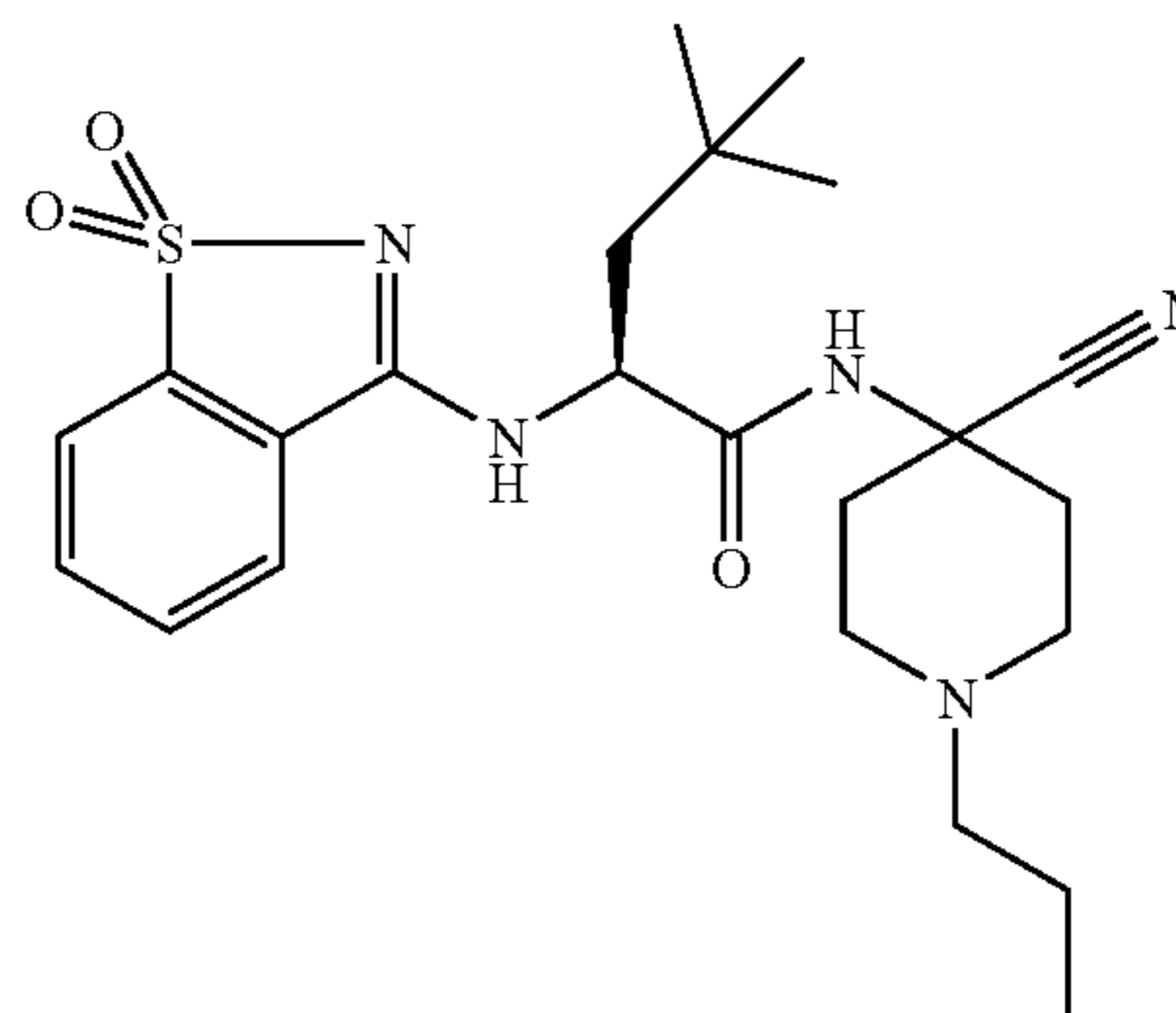
2-(1,1-dioxo-1H-λ 6 -benzo[d]isothiazol-3-ylamino)-4,4-dimethyl-pentanoic acid(4-cyano-1-propylpiperidin-4-yl)-amide
