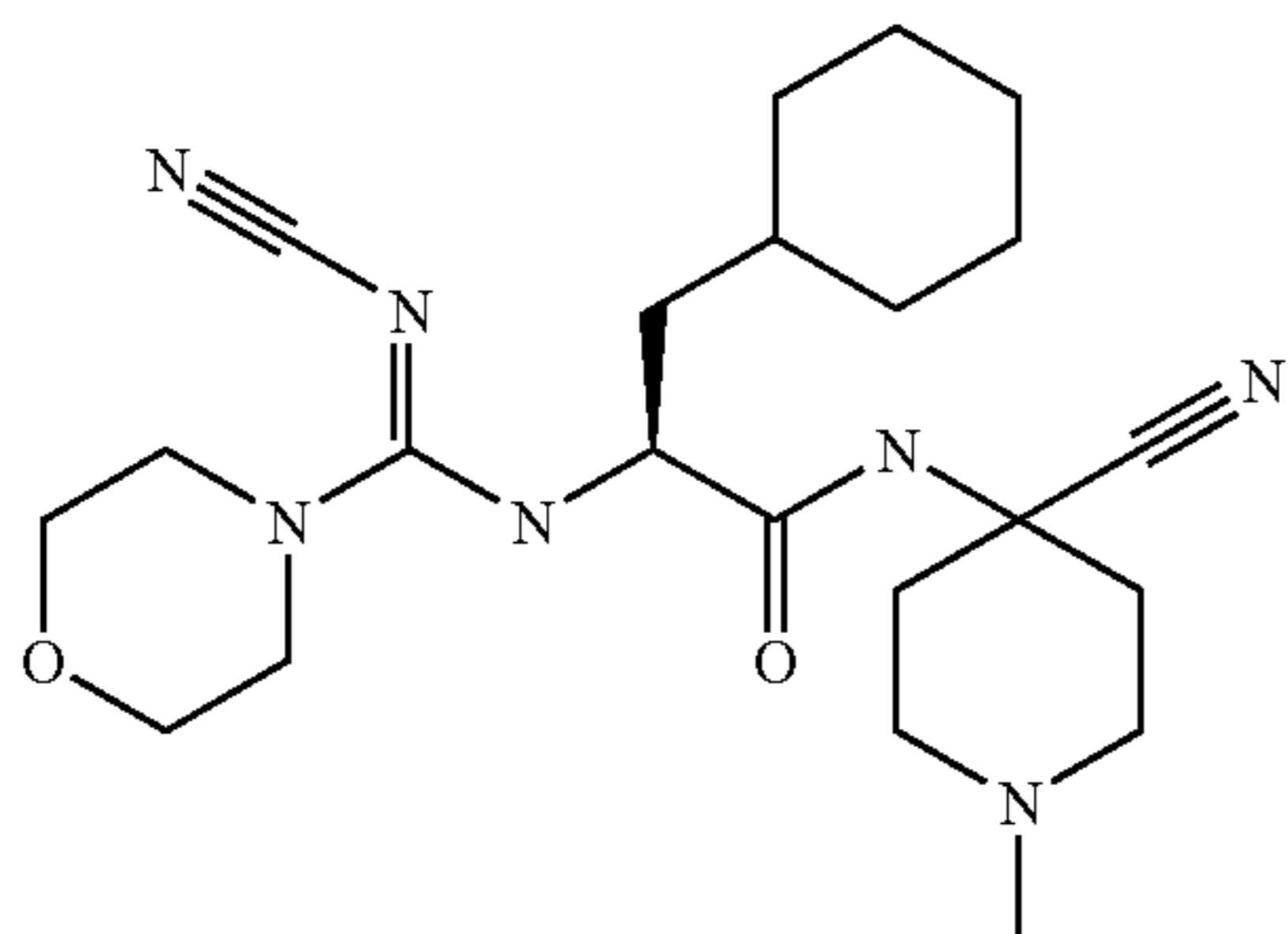
N-(4-cyano-1-methyl-piperidine-4-yl)-3-cyclohexyl-2-[N-cyano-morpholine-4-carboximidoyl]-amino]-propionamide (Method H)
