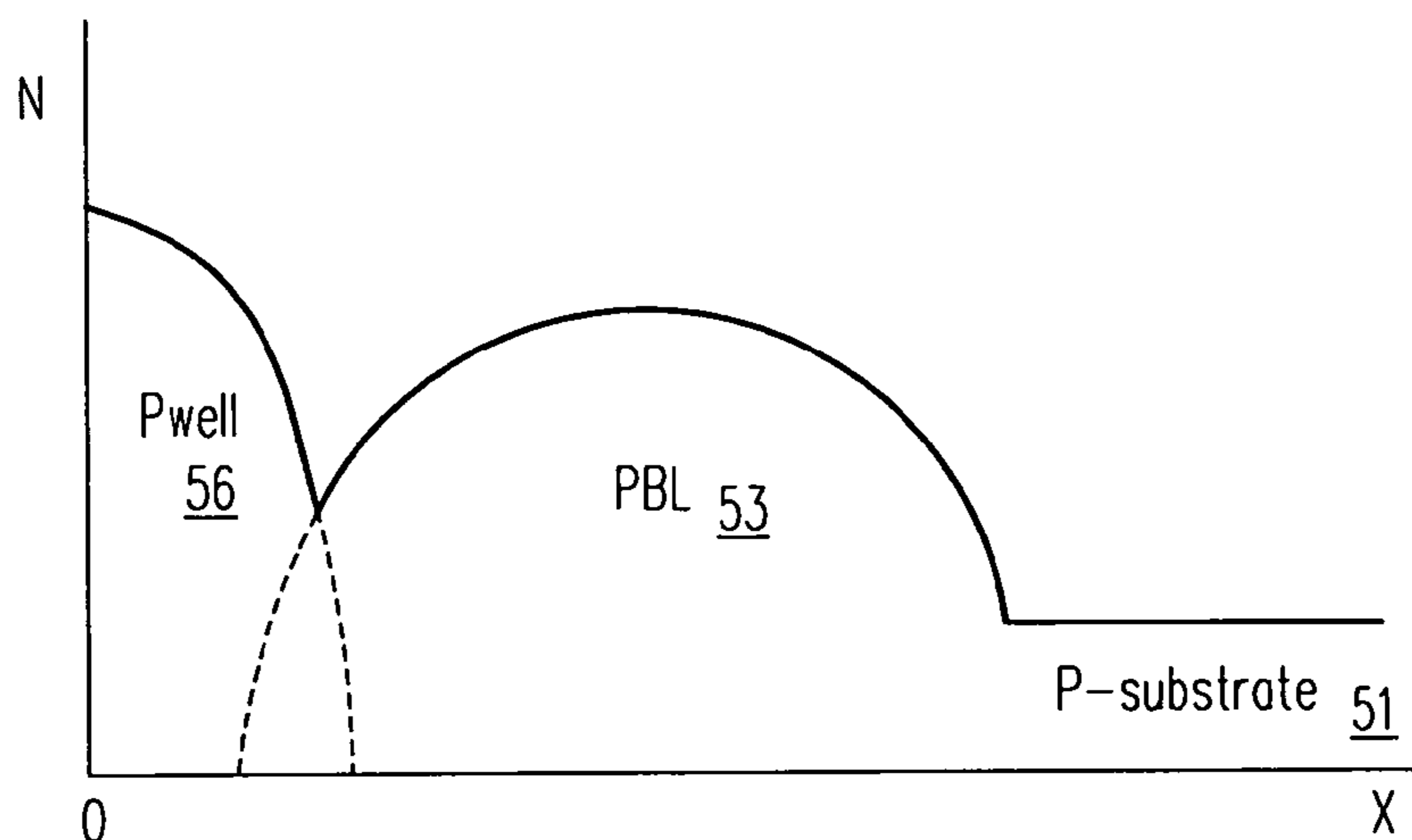
FIG. 3C (Prior Art)
