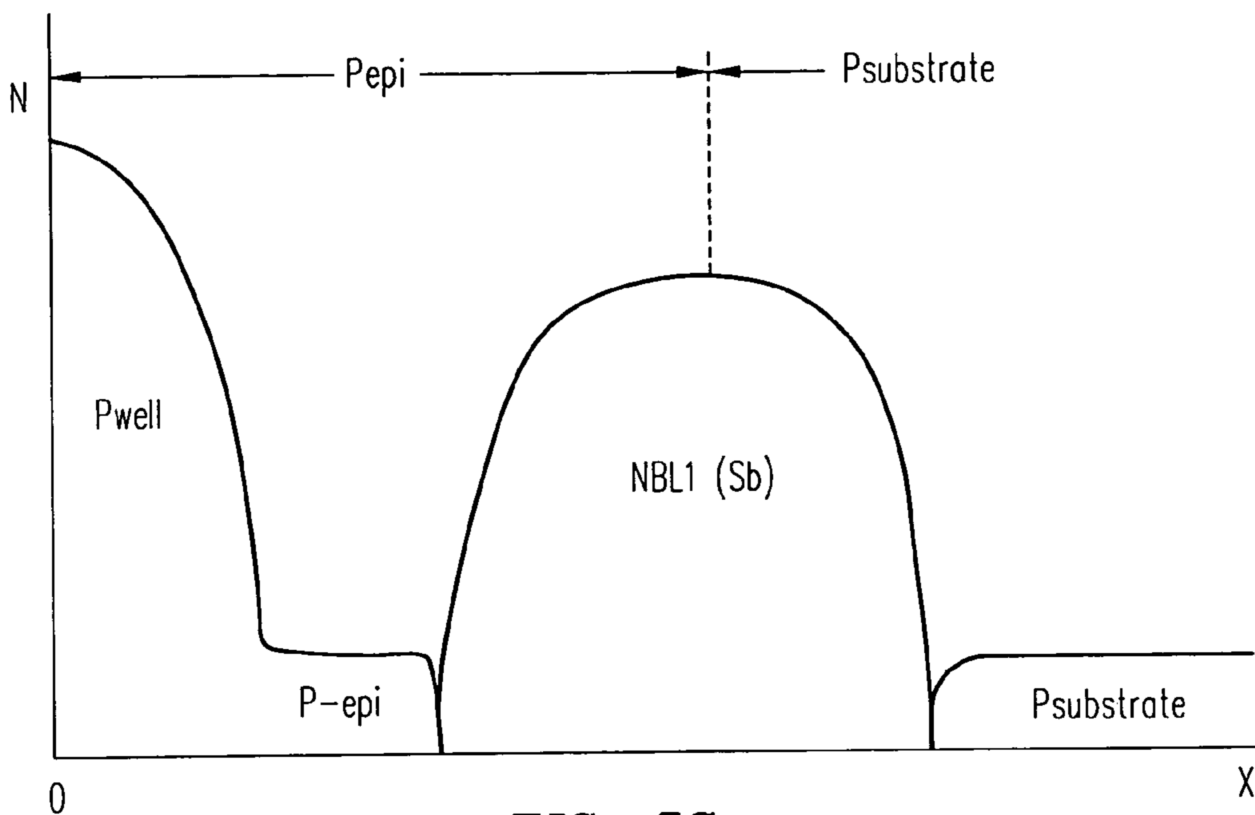
FIG. 5C (Prior Art)
