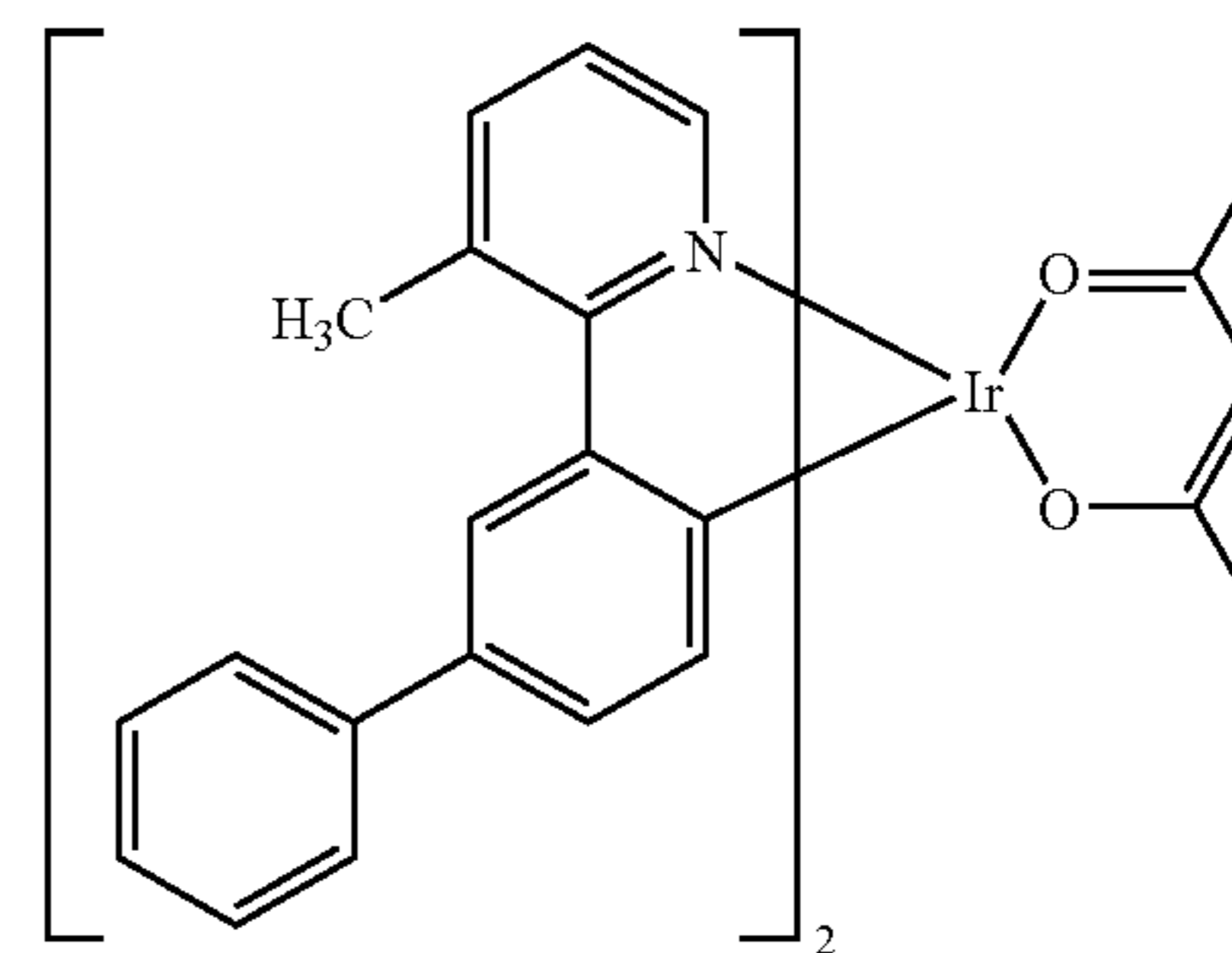
\text{Ir}(5\text{-3'-Mepq})_2(\text{acac})
