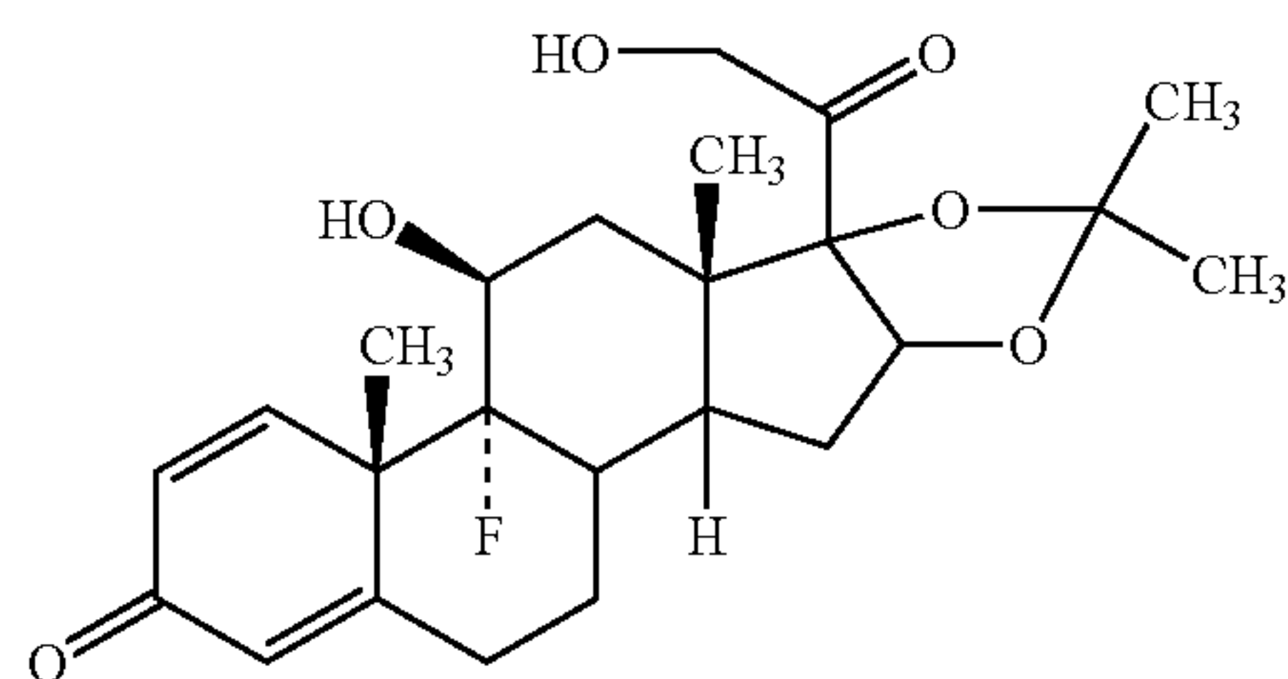
Triamcinolone acetonide
