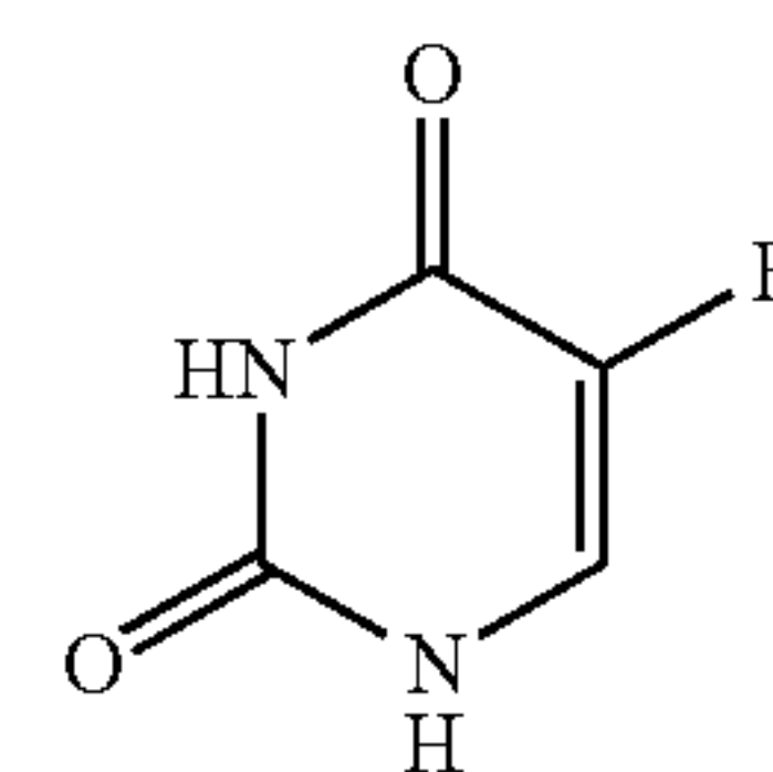
5-Fluorouracil (5FU).
