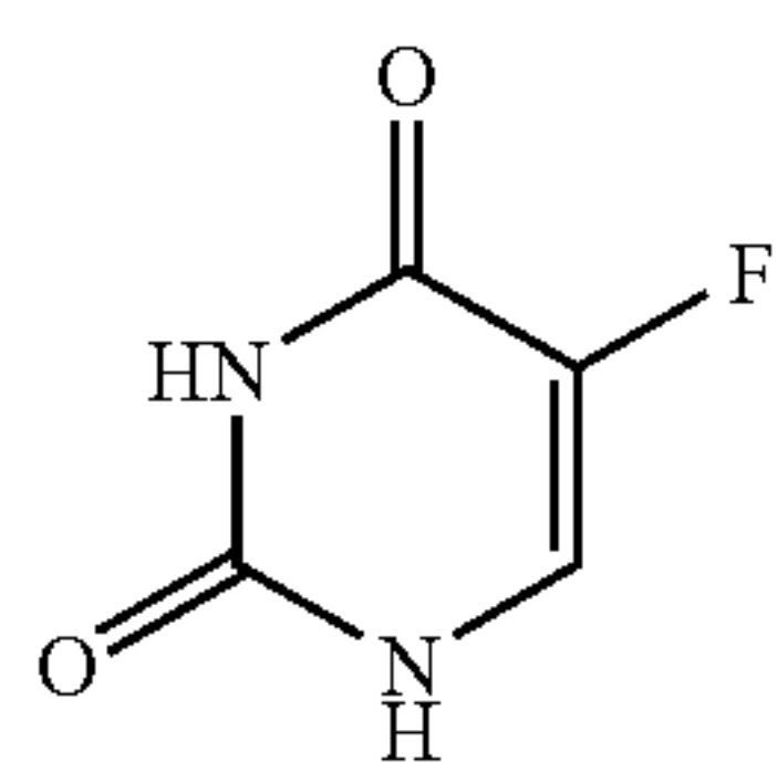
5-Fluorouracil (5FU)
