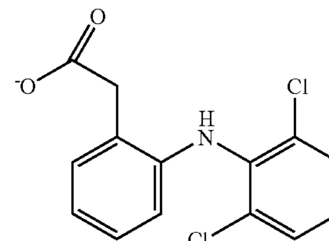
Ciprofloxacin-Diclofenac
