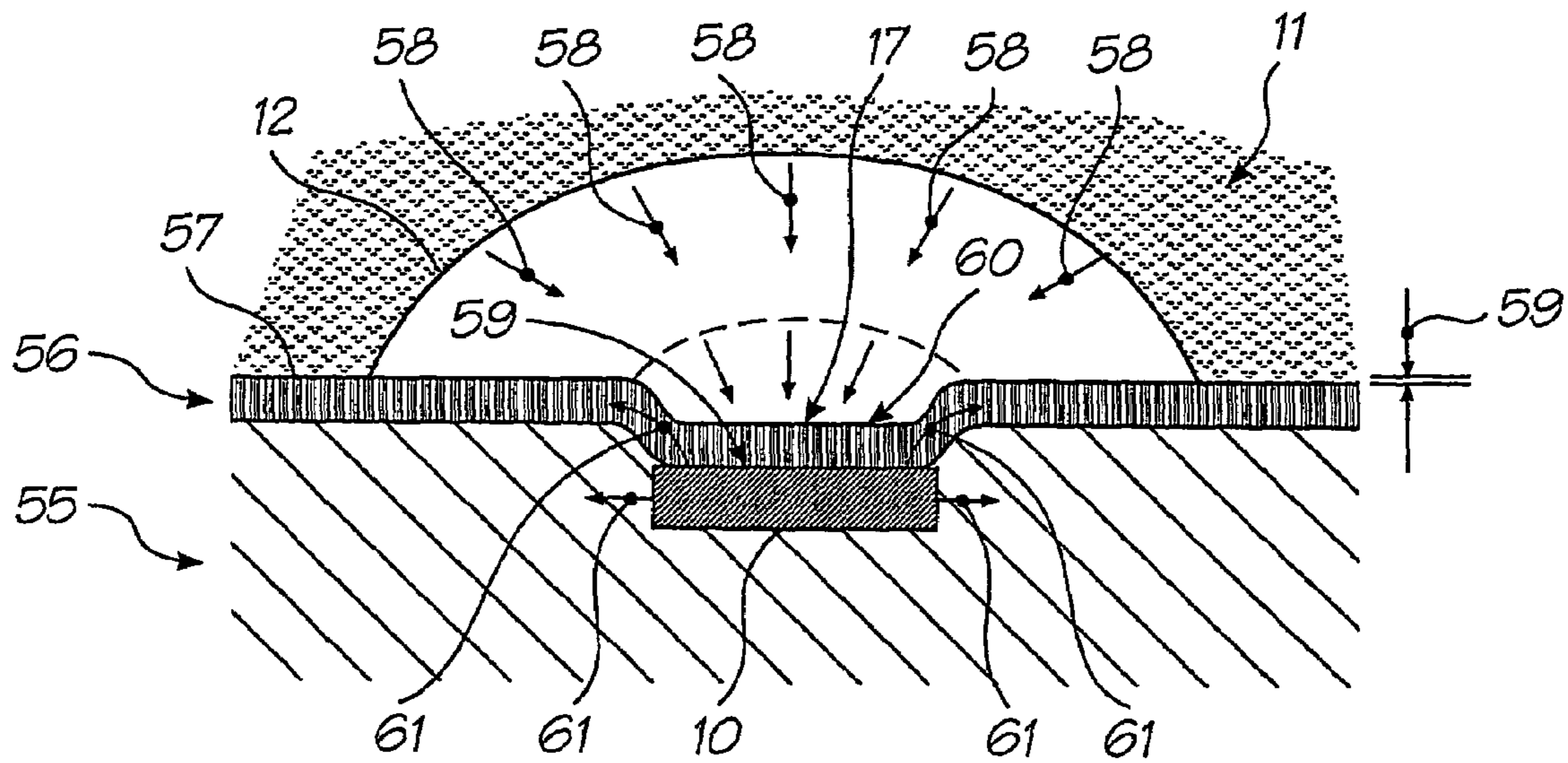
FIG. 47 (PRIOR ART)
