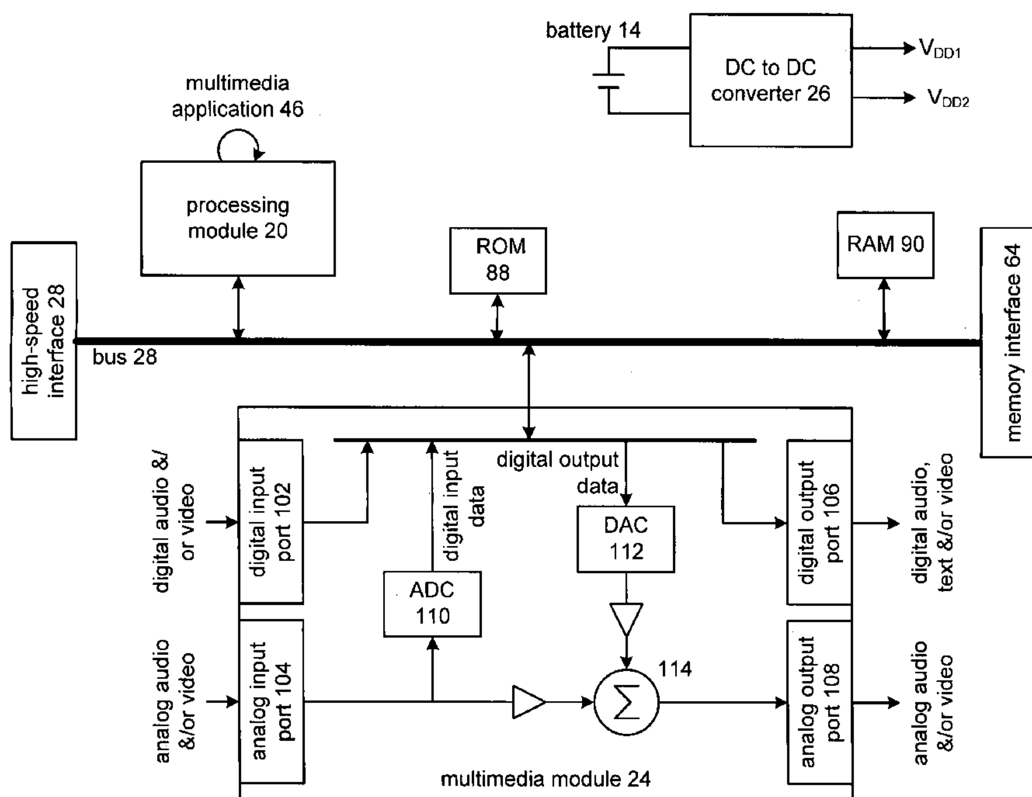
battery-optimized system-on--chip 100
