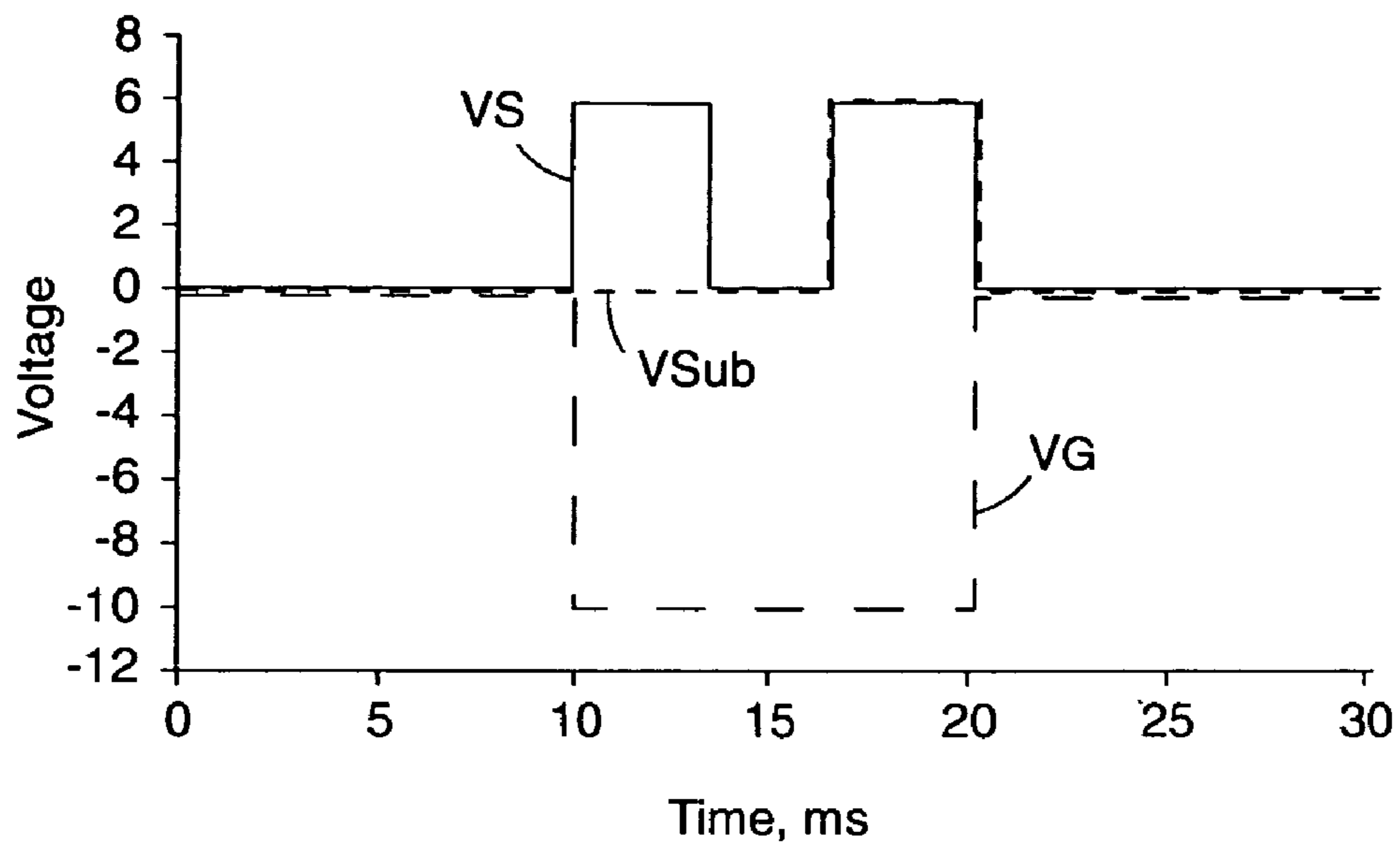
Fig. 5 Prior Art
