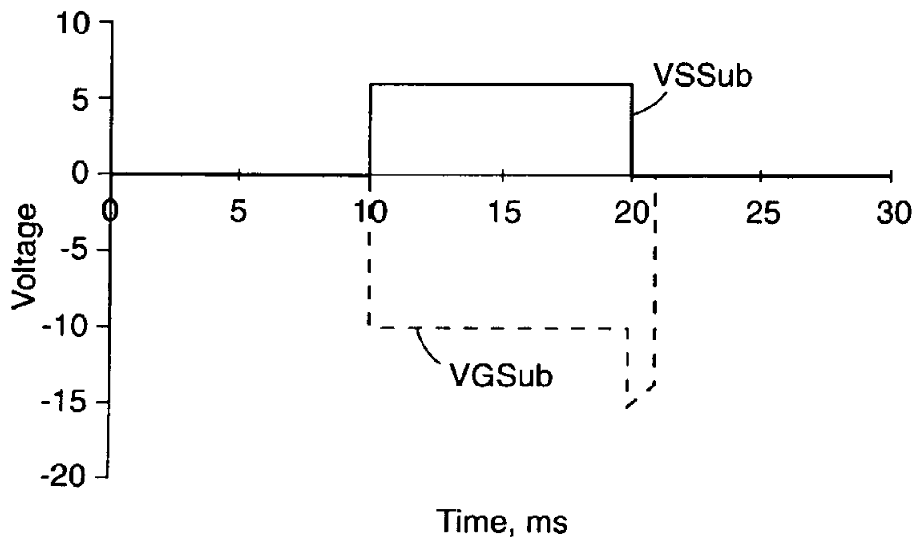
Source erase with delayed gate discharge
