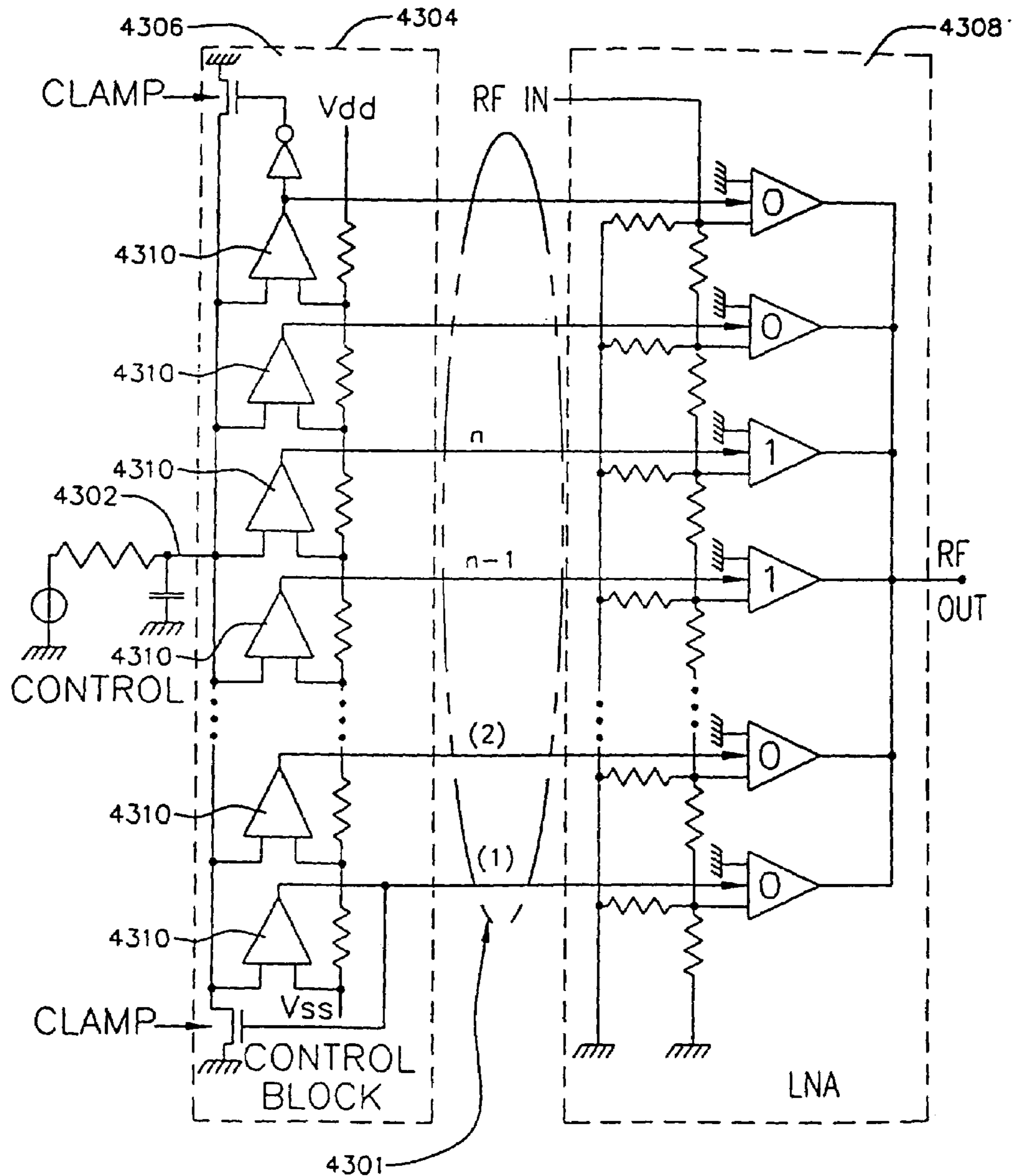
FIG. 43 CLAMPING CONTROL RANGE
