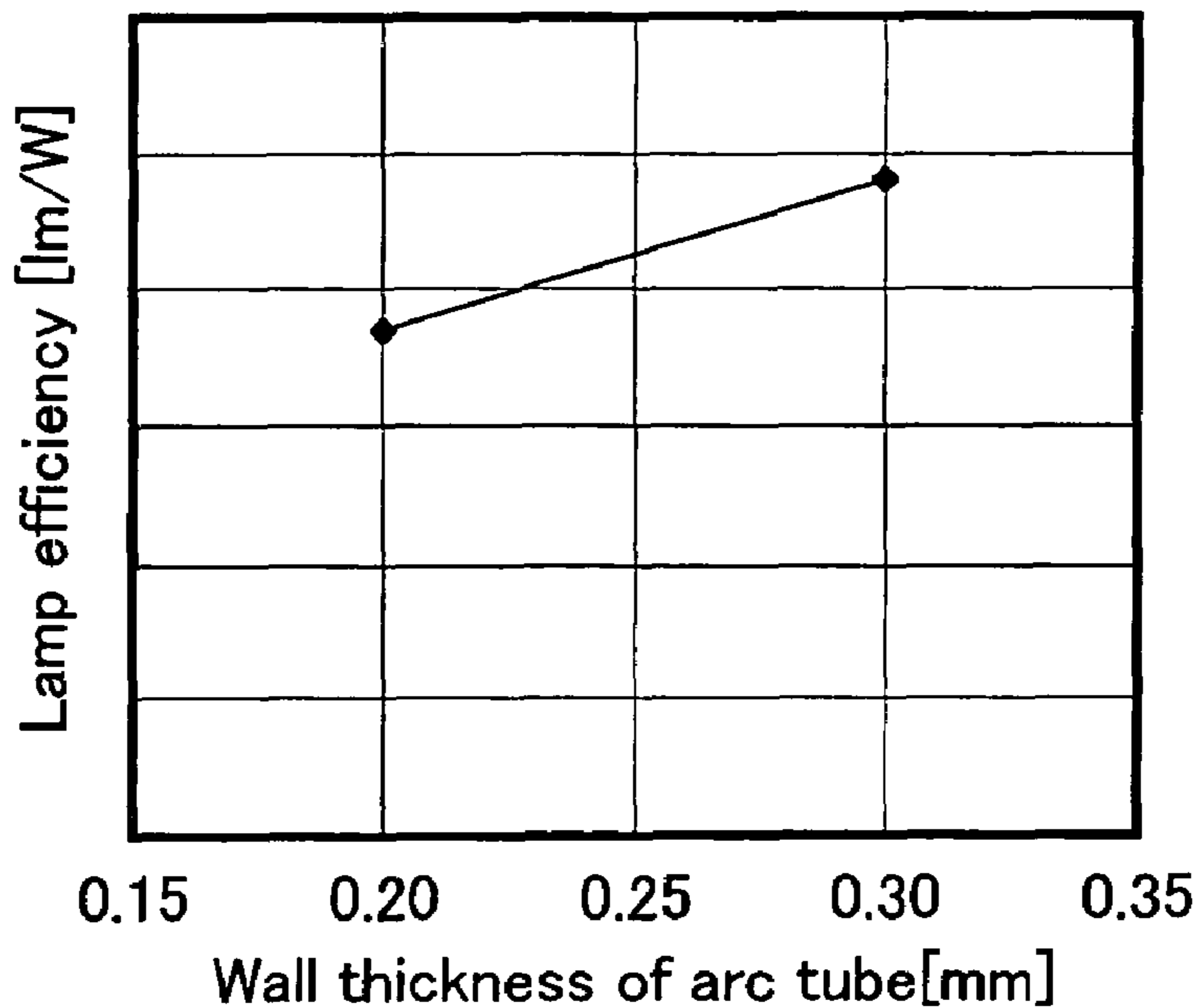
Correlation between wall thickness of arc tube and lamp efficiency
