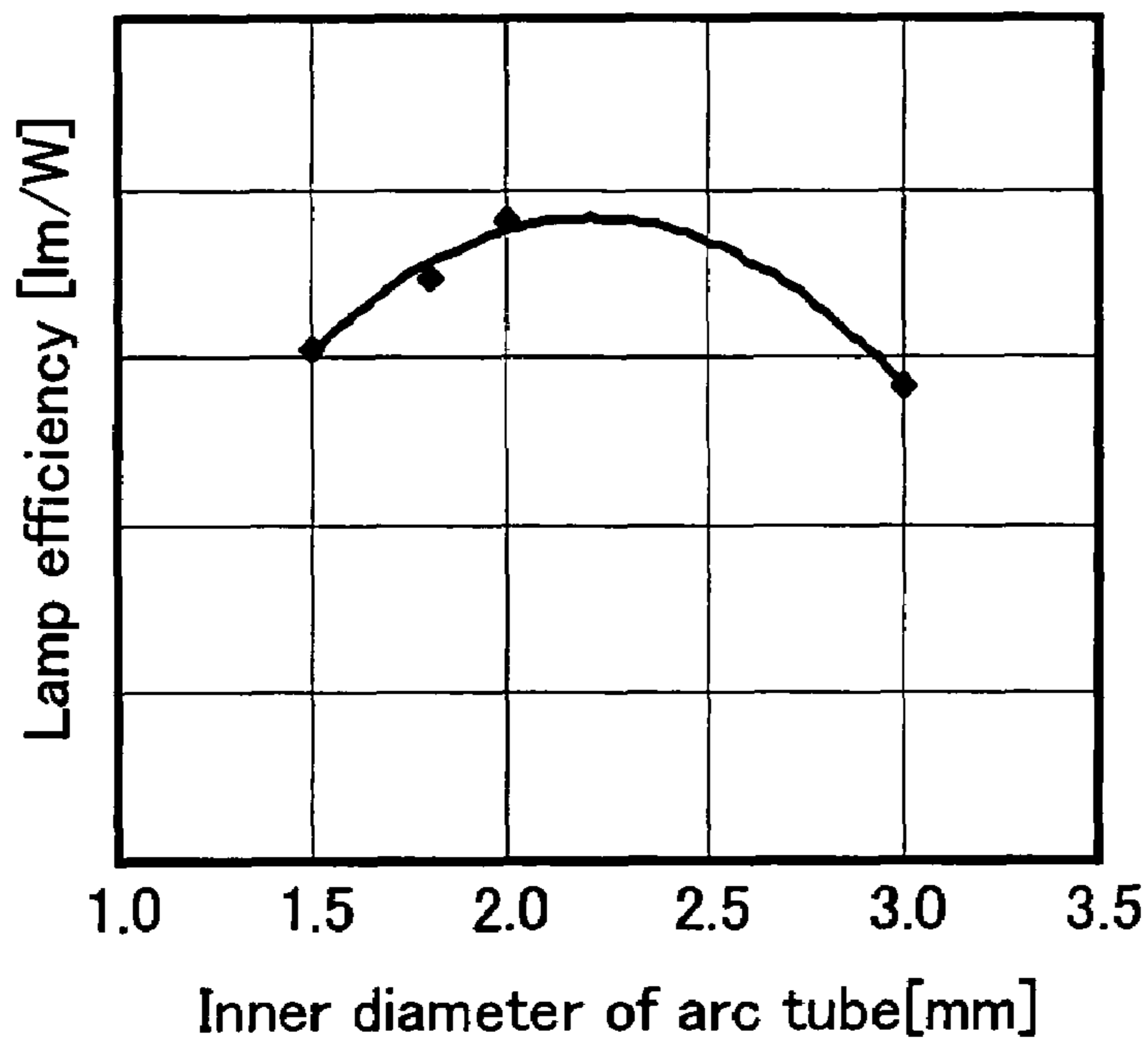
Correlation between inner diameter of arc tube and lamp efficiency
