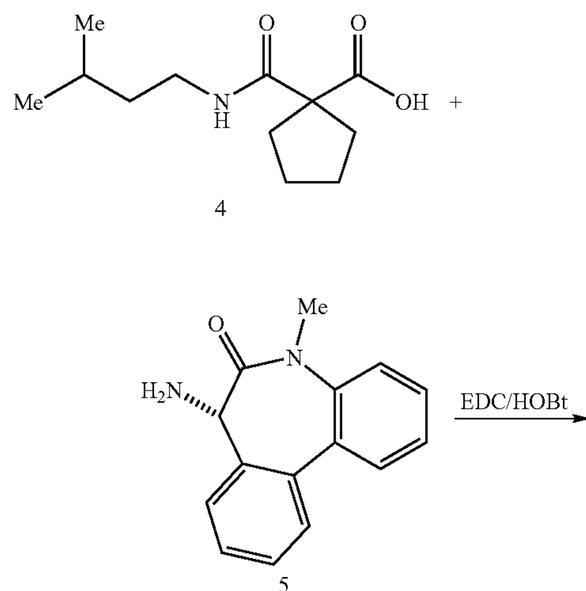
Scheme 2
