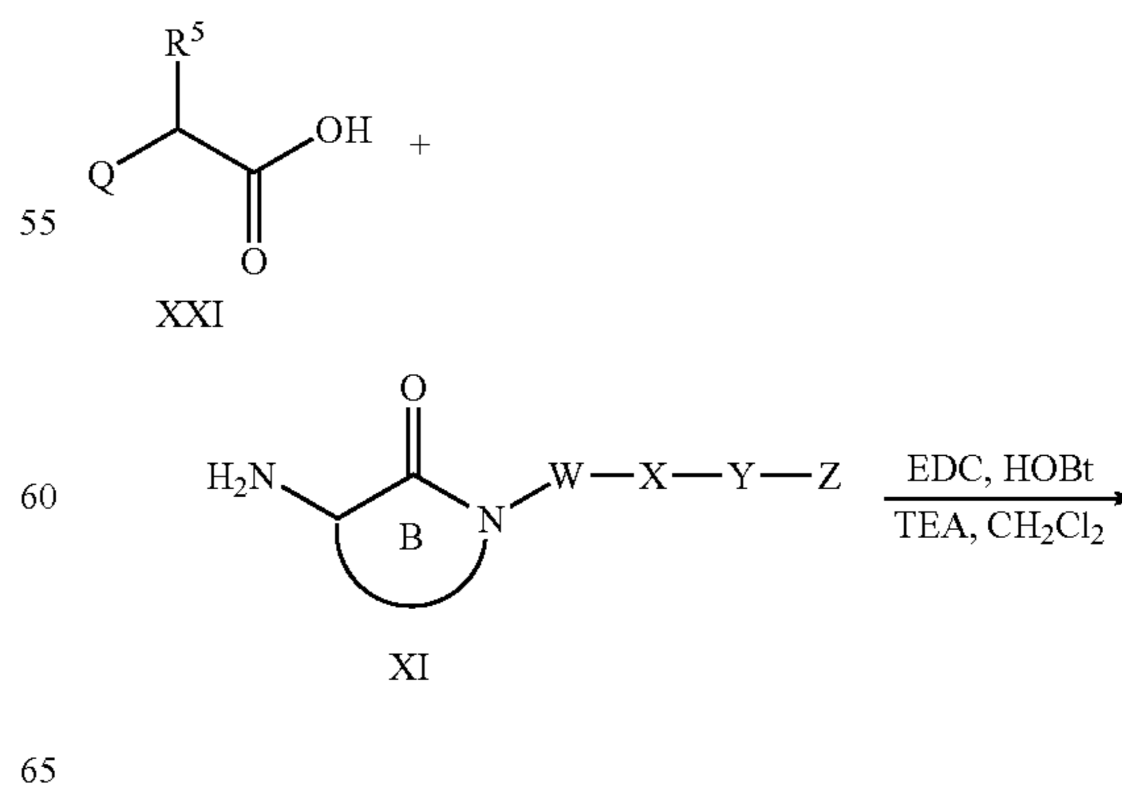
Scheme 6
