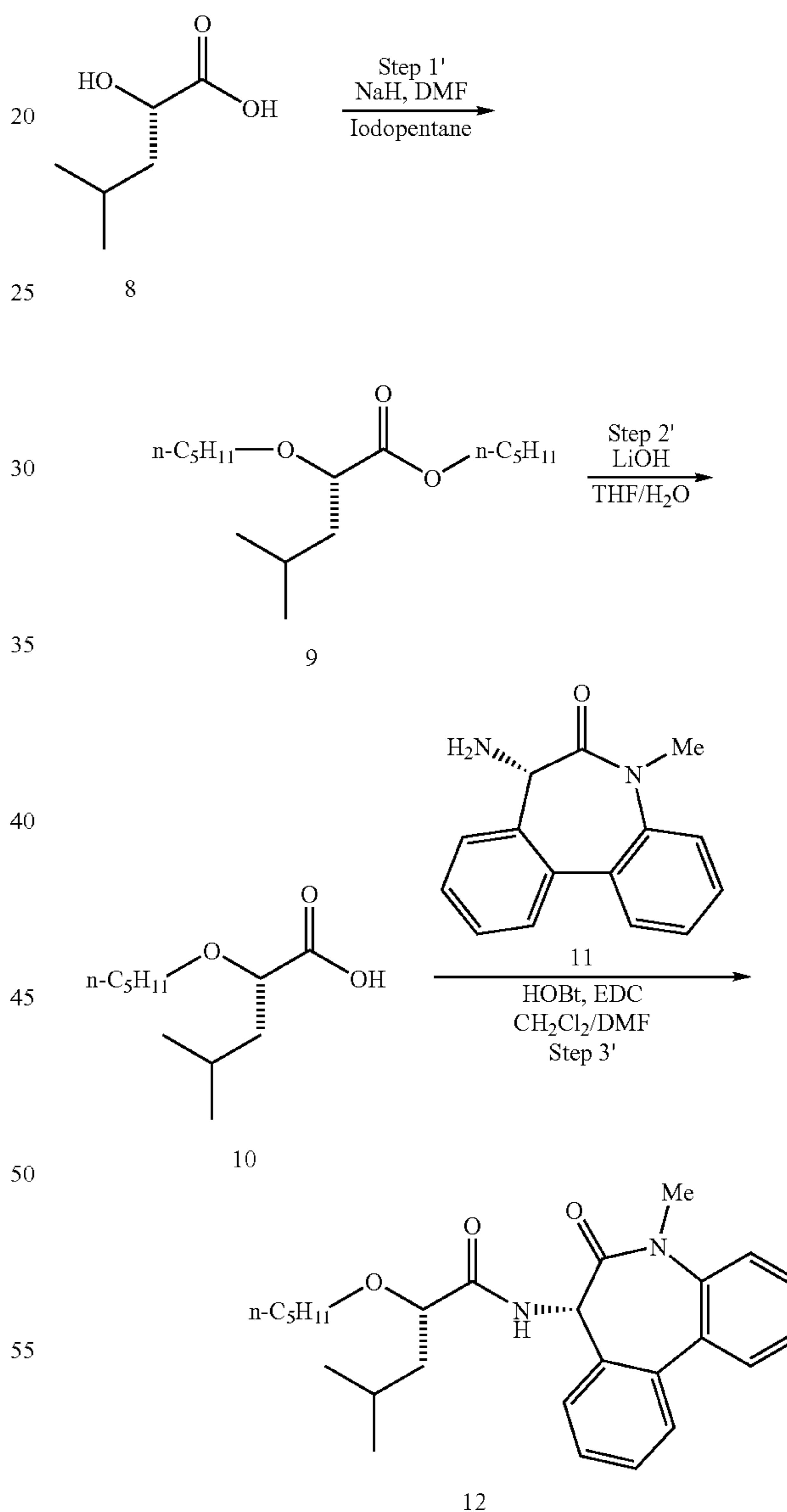
Scheme 8
