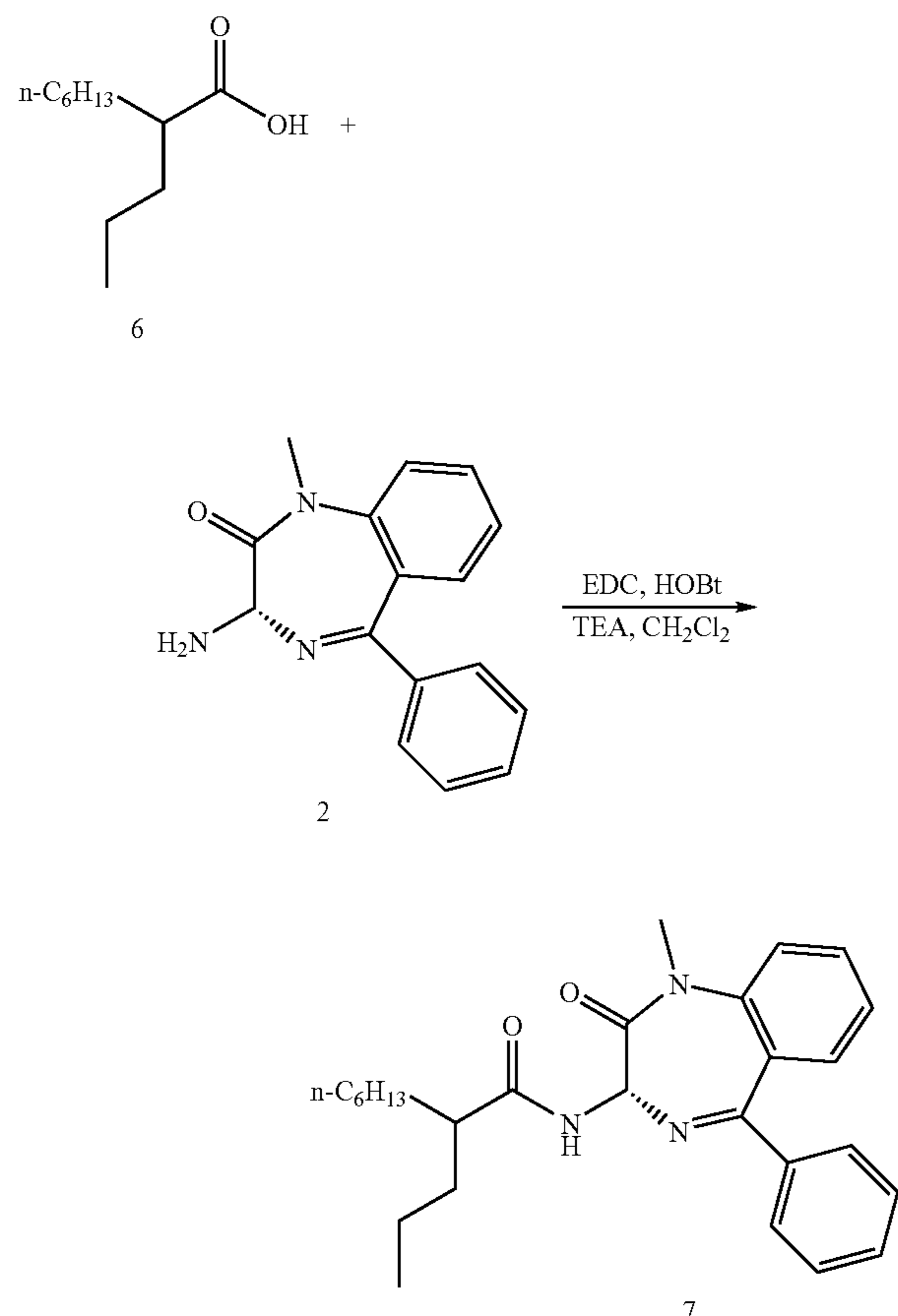
Scheme 7
