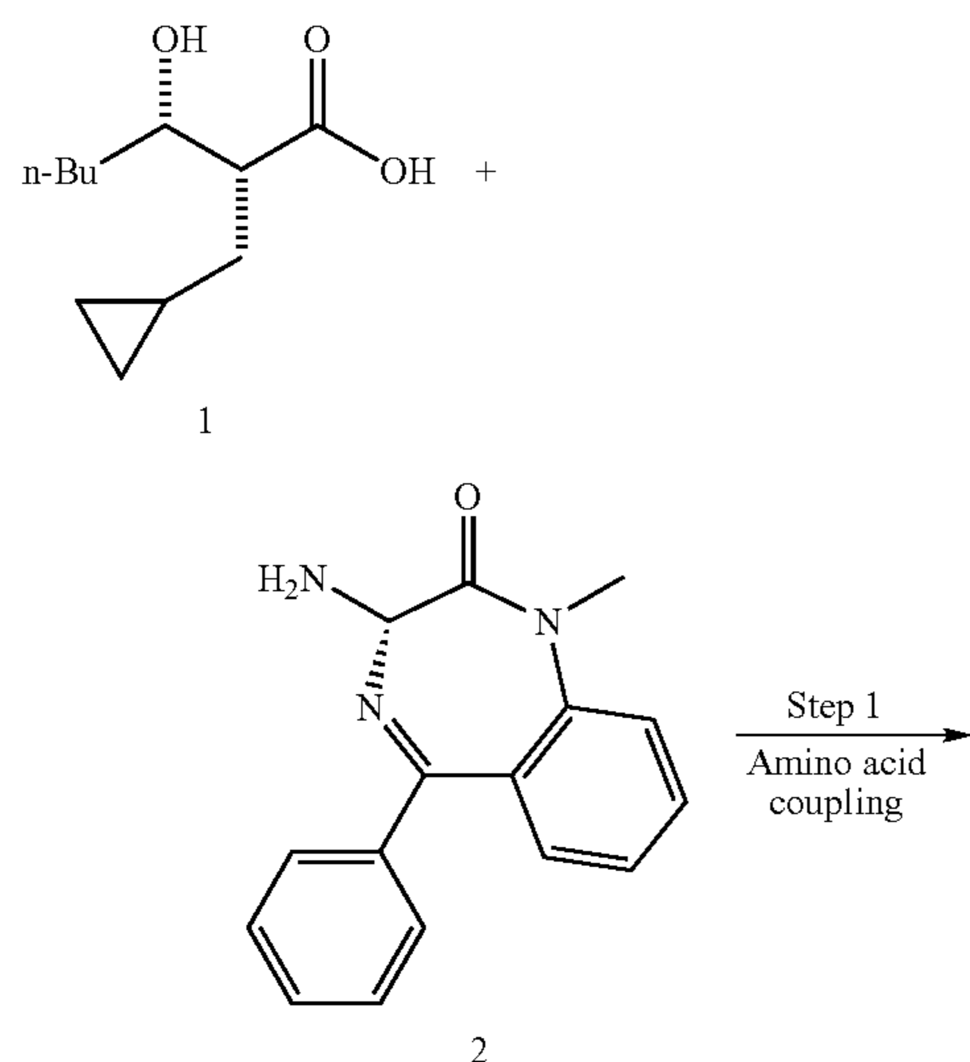
Scheme 5
