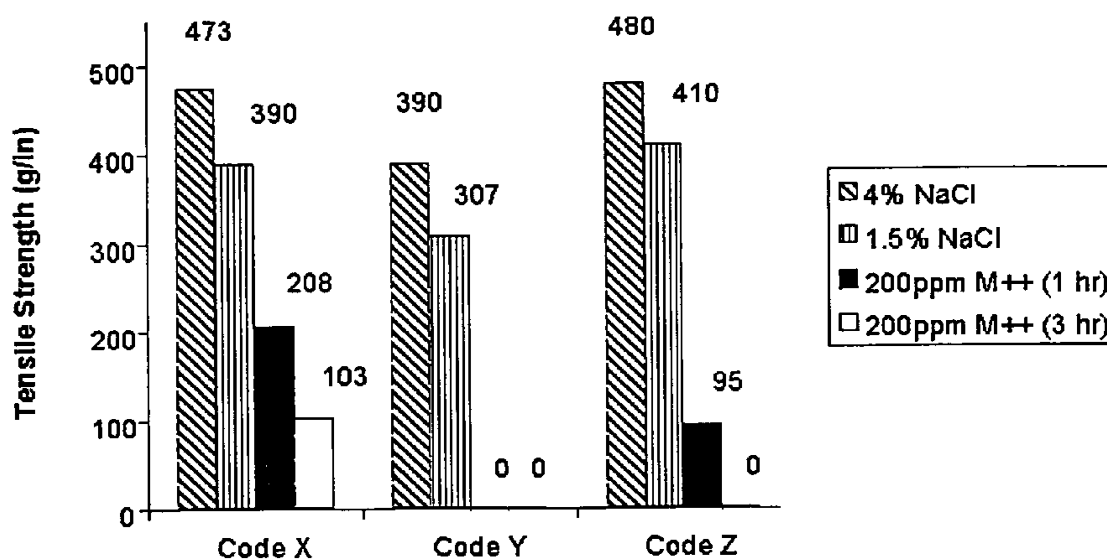
CDWT (in 1.5% and 4.0% NaCl) and soaked CD tensiles (1 and 3 hour soak in hard water) for NaAMPS-SSB/Dur-O-Set RB-based basesheets
