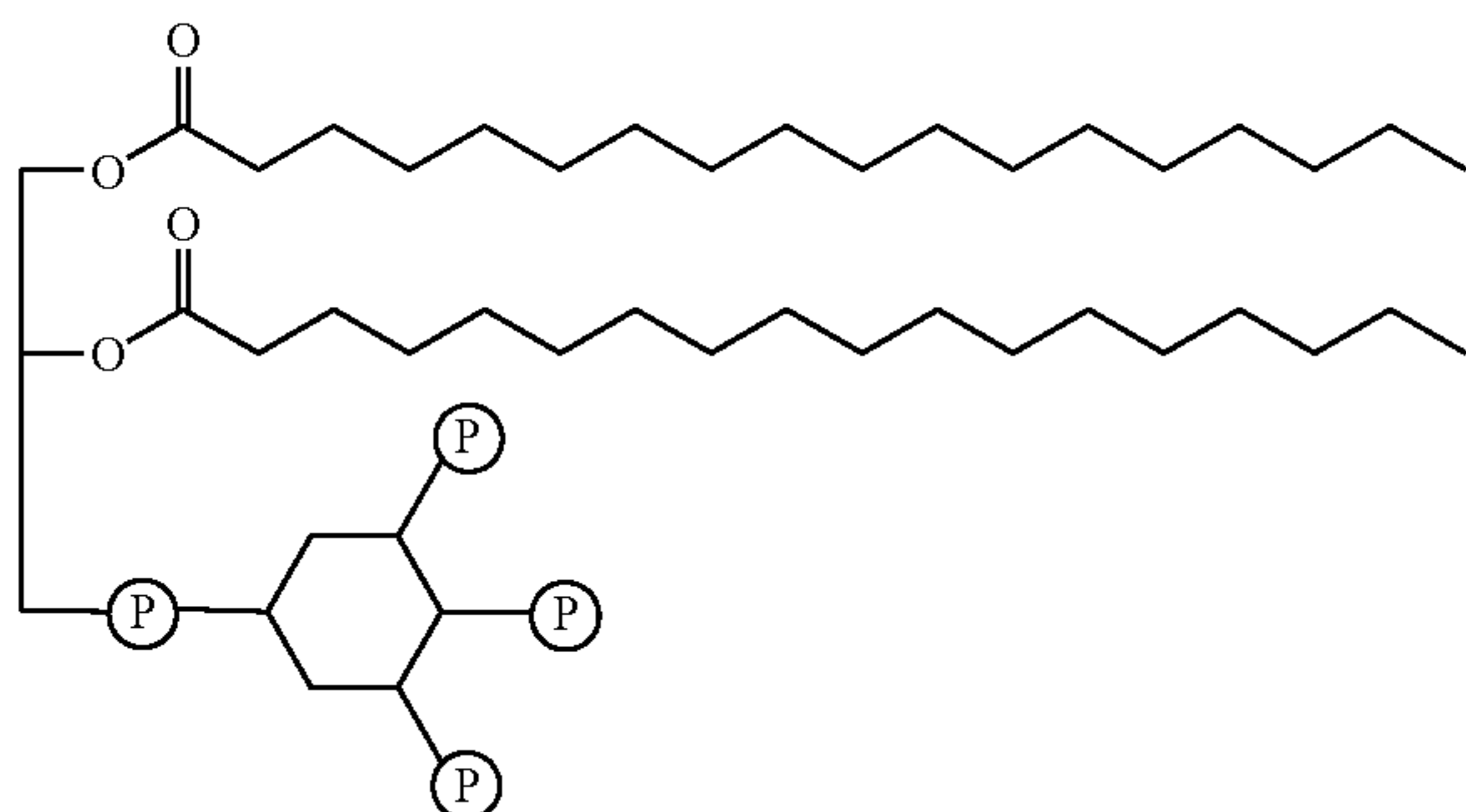
PIP3
