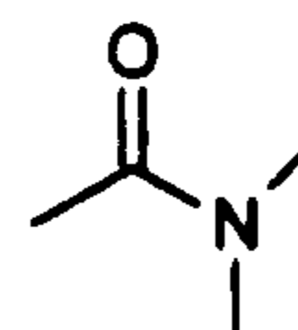
N,N-dimethylacetamide (DMA)
