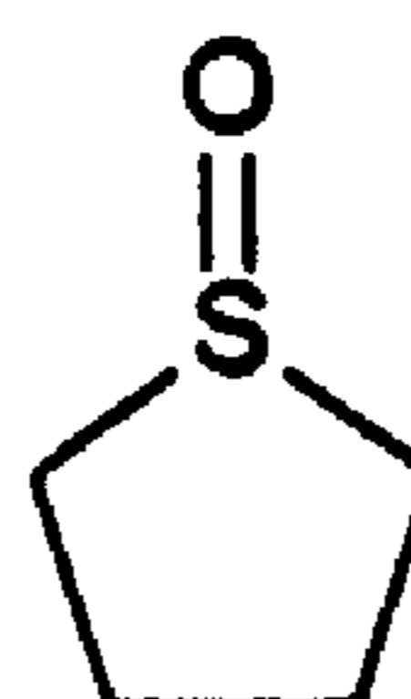
Tetramethylene sulfoxide
