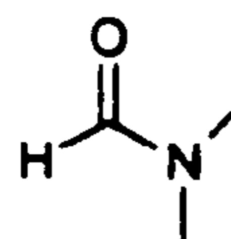
N,N-dimethylformamide (DMF)
