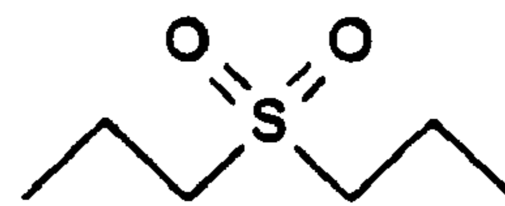
n-Propyl sulfone
