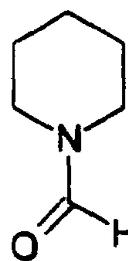
N-formyl piperidine
