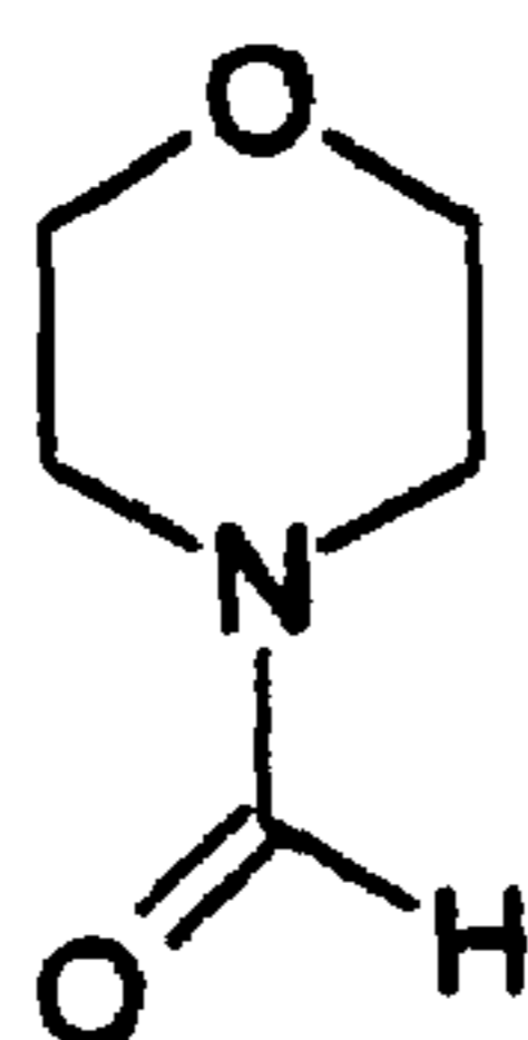
N-formyl morpholine
