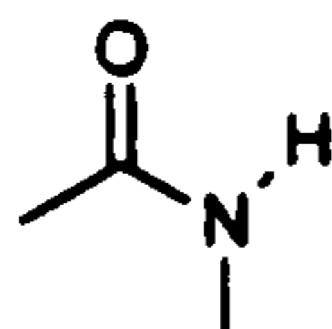
N-methylacetamide (MMA)
