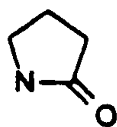
2-pyrrolidone
