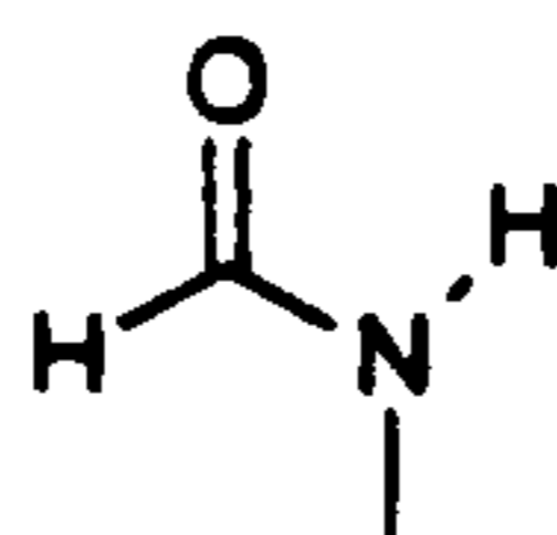
N-methylformamide (MMF)
