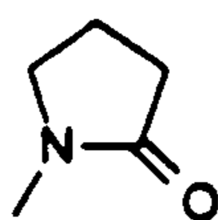
N-methylpyrrolidone (NMP)
