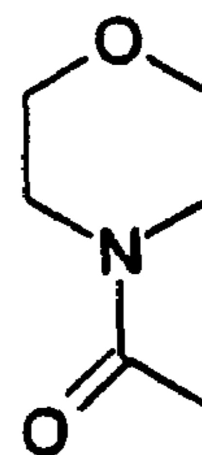
N-acetyl morpholine
