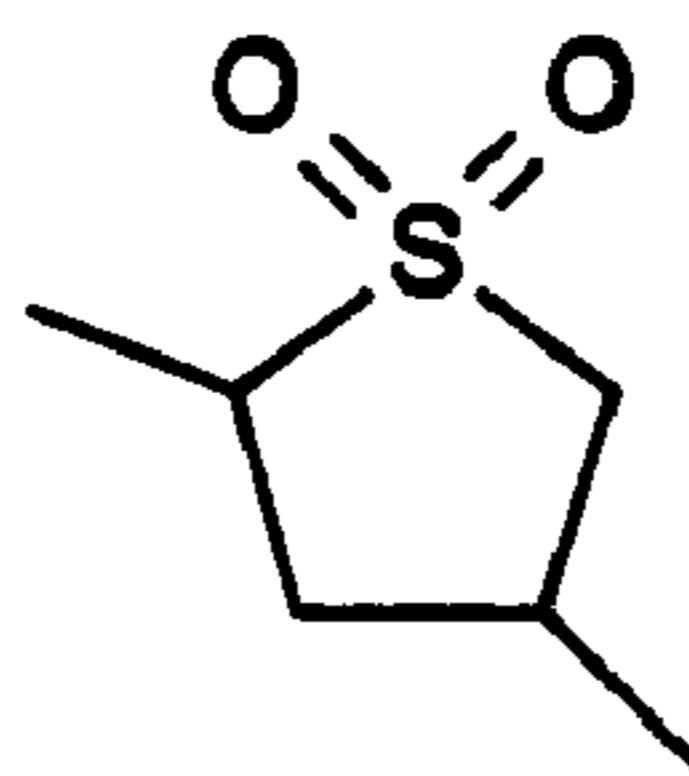
2,4-Dimethylsulfolane
