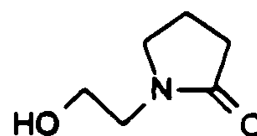
N-hydroxyethylpyrrolidone (HEP)
