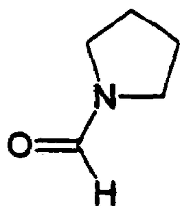
N-formyl pyrrolidine
