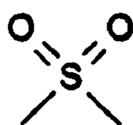
Methyl sulfone
