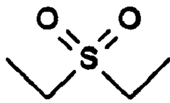
Ethyl sulfone
