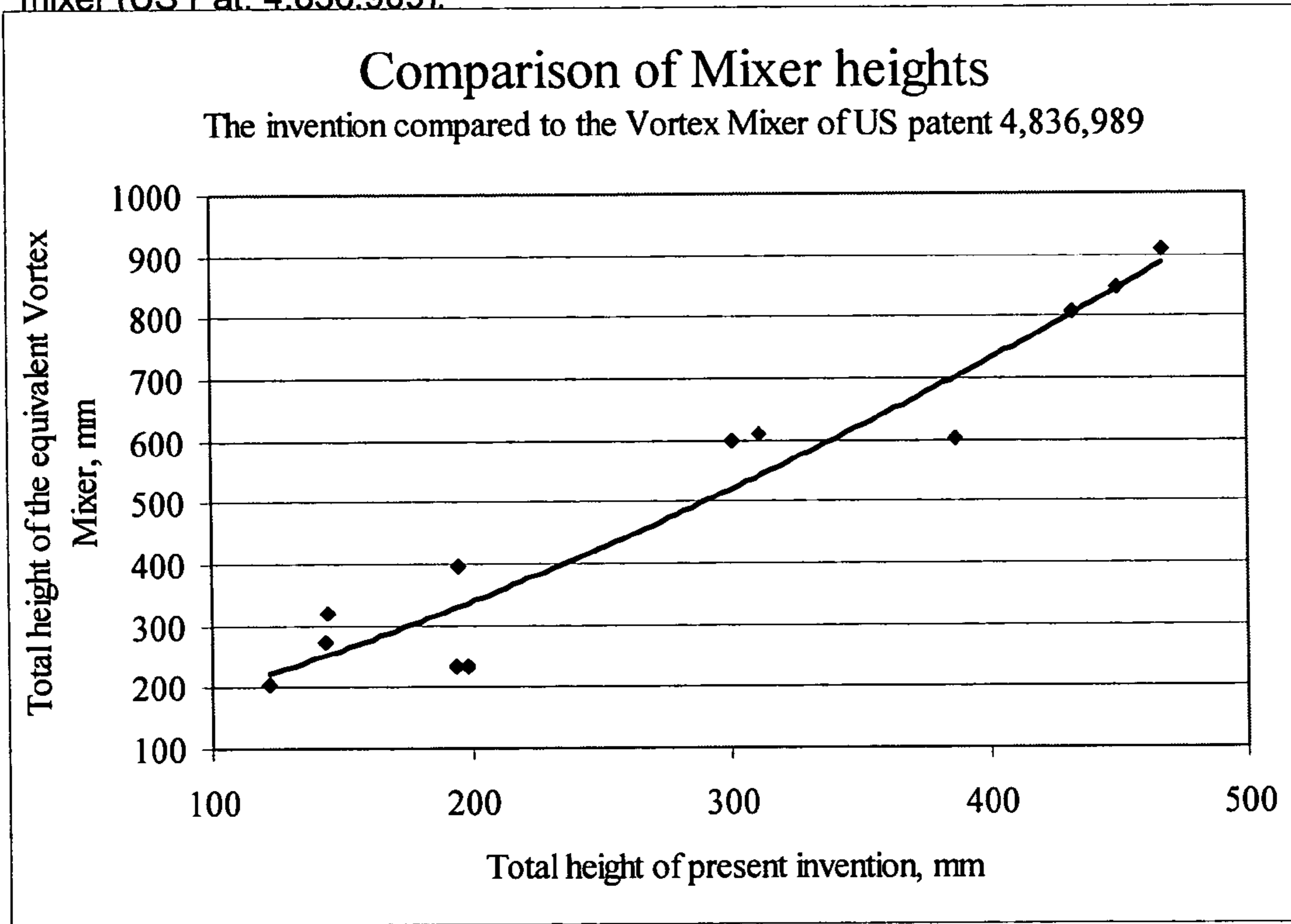
Graph 1: The height of the present invention compared to the height of the vortex mixer (US Pat. 4.836.989).
