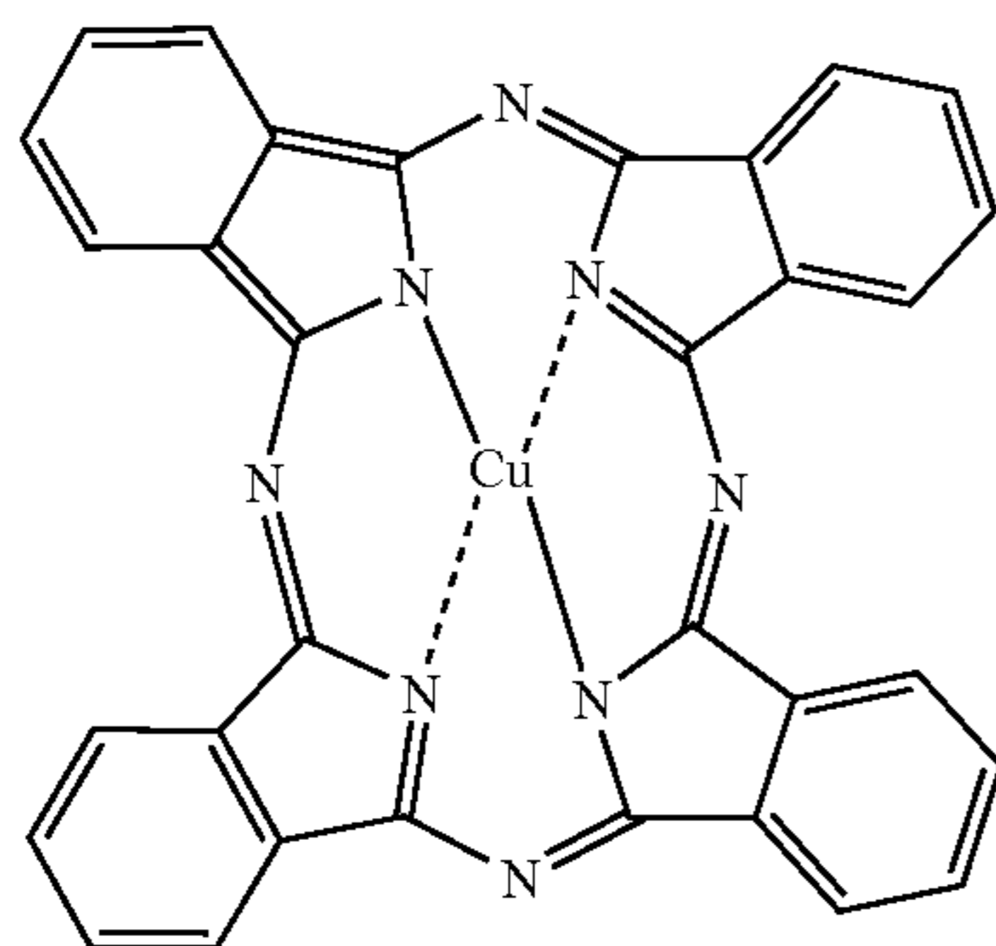
CuPc
