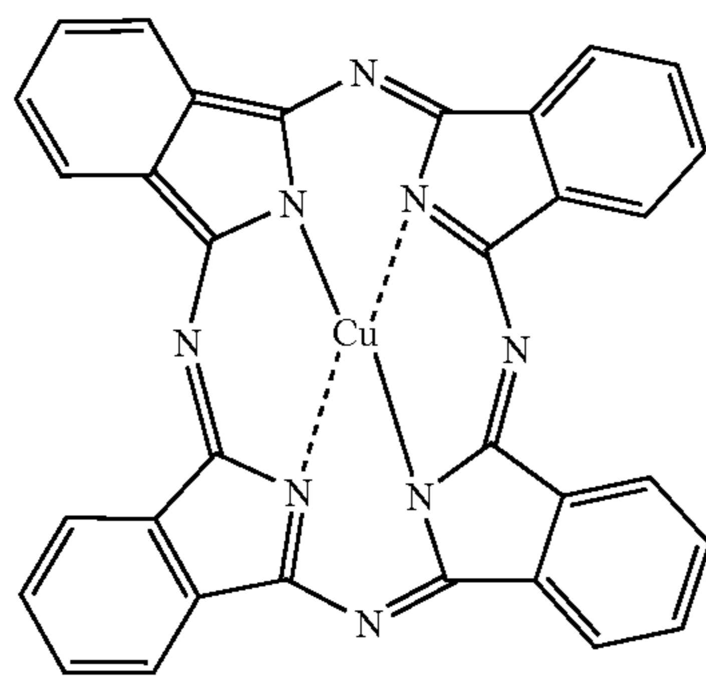
CuPc
