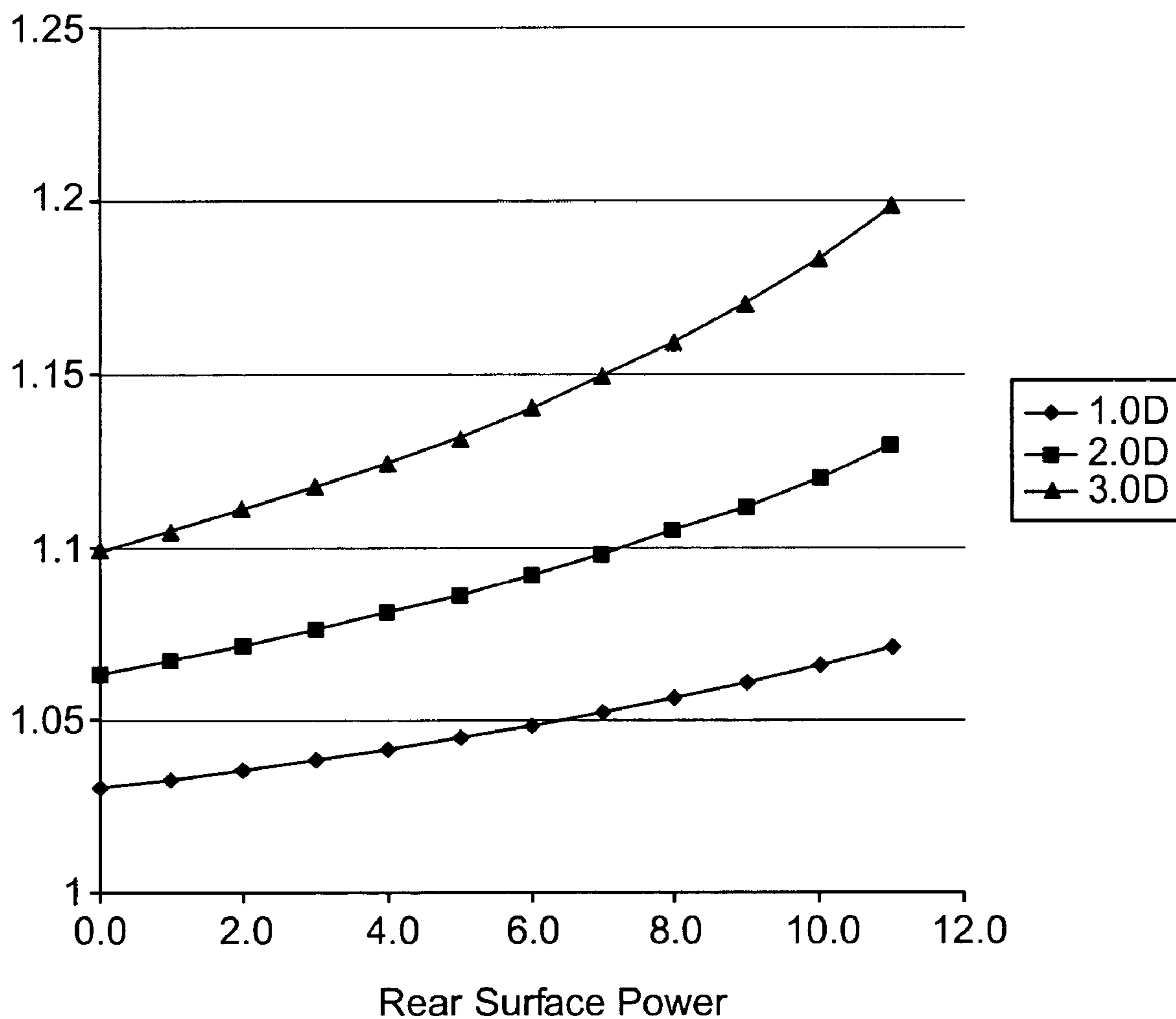
FIG. 4 Angular Magnification
