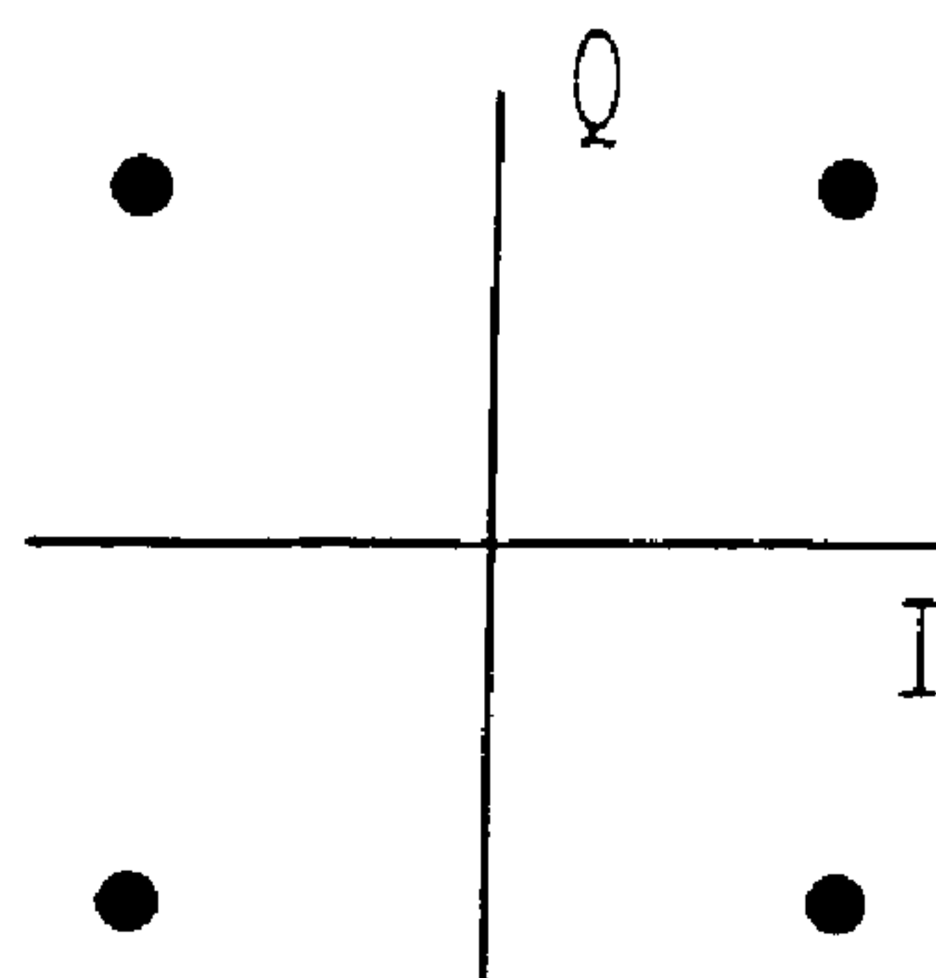
QPSK CONSTELLATION
