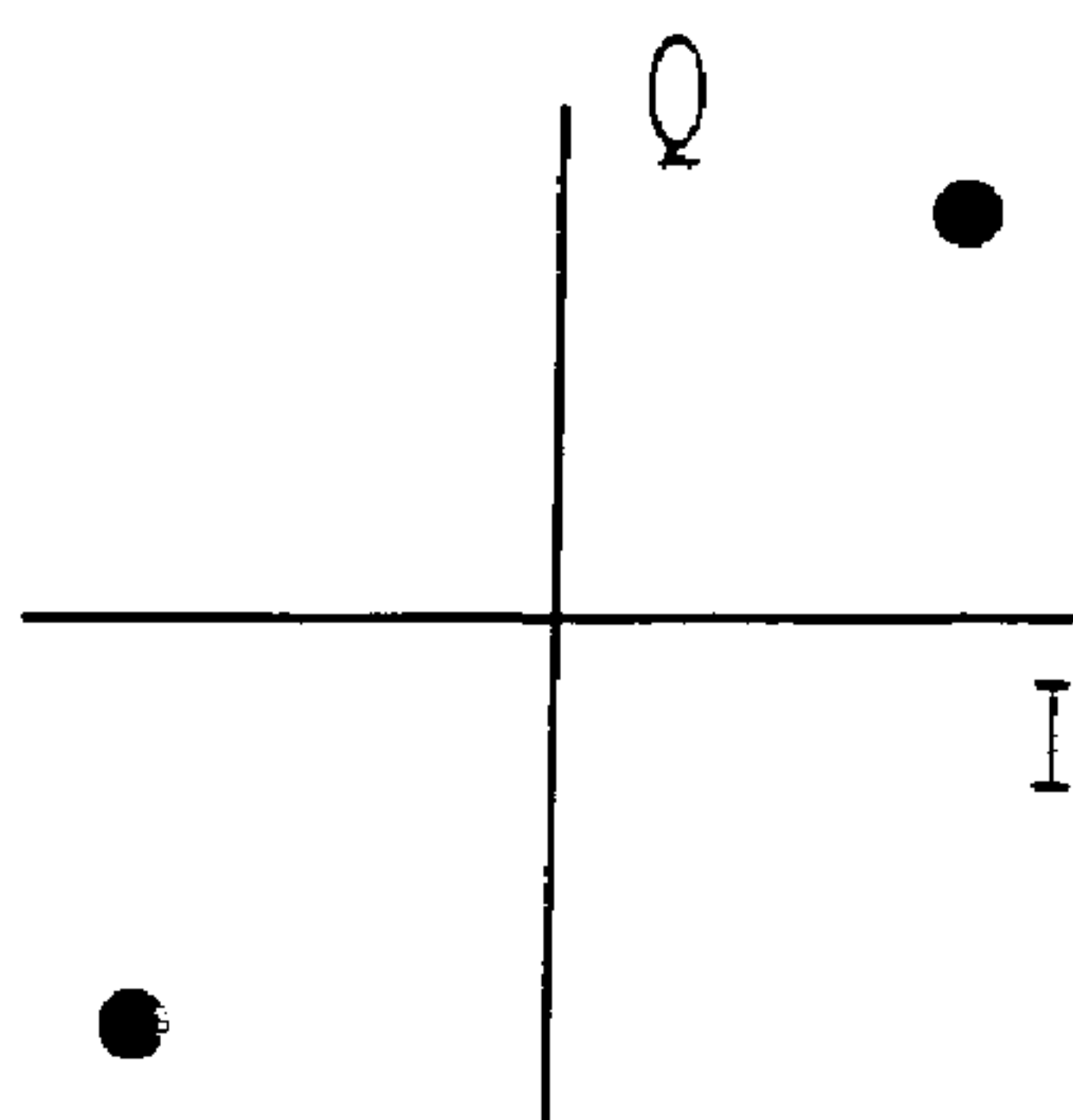
BPSK CONSTELLATION ORIENTED AT 45 DEGREE ANGLE TO BOTH AXES
