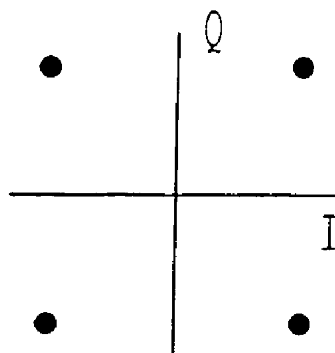
QPSK CONSTELLATION
