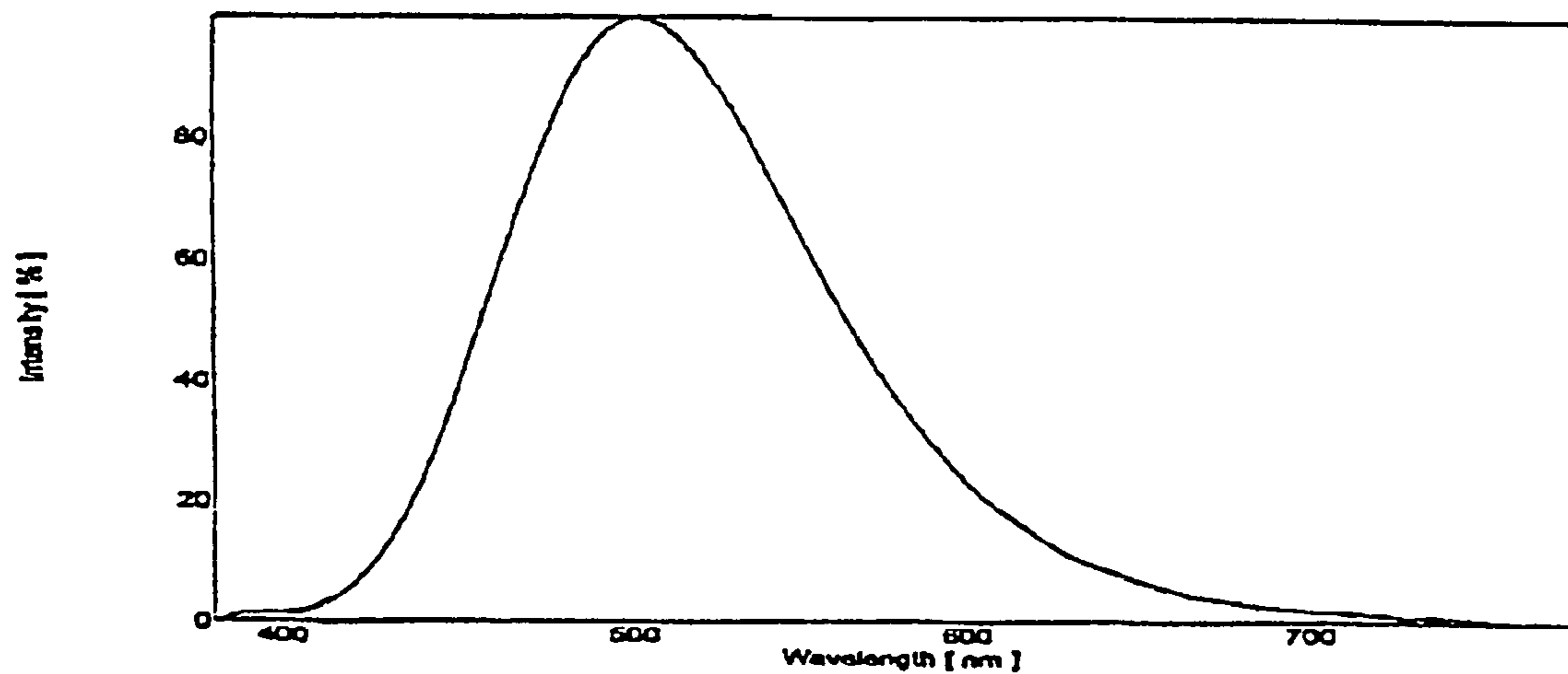
Blue-Green VF display: Emission spectrum Improved DOD tuned to Blue-Green VF display
