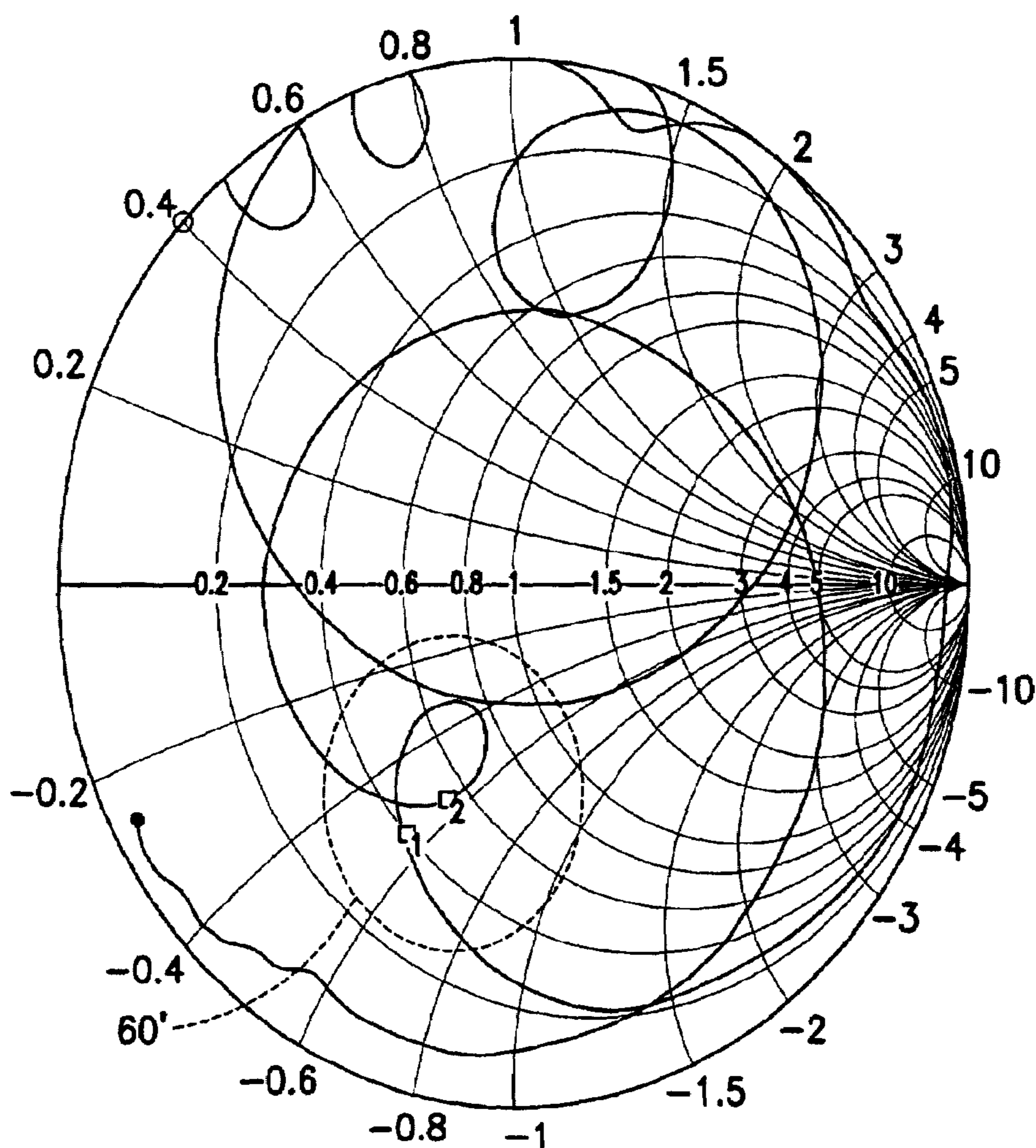
S-PARAMETER SMITH CHART
