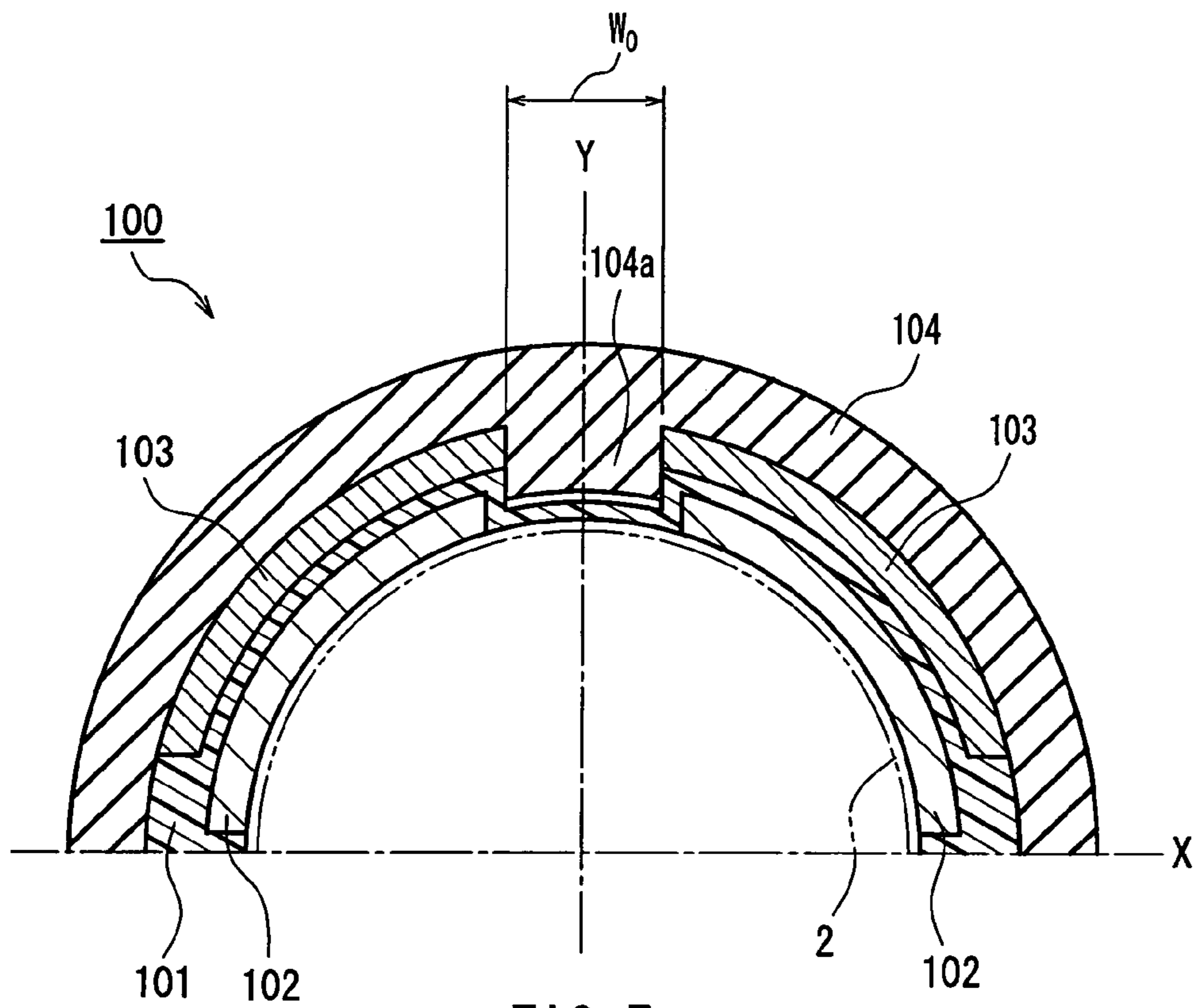
FIG. 7 PRIOR ART
