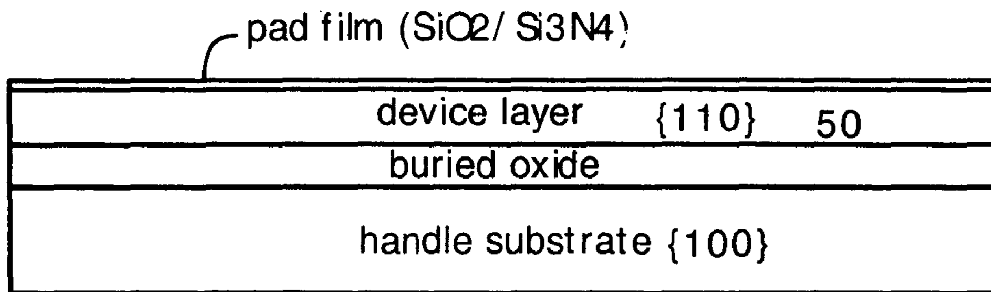
Fig. 3a SOI substrate with pad film
