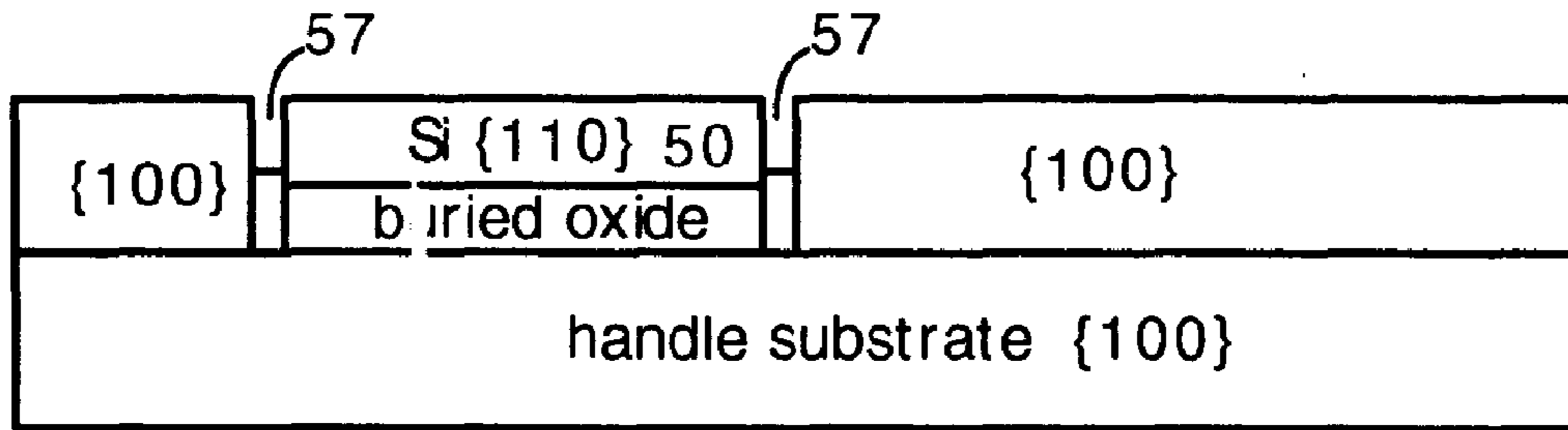
Fig. 3e Process spacer with selective etch
