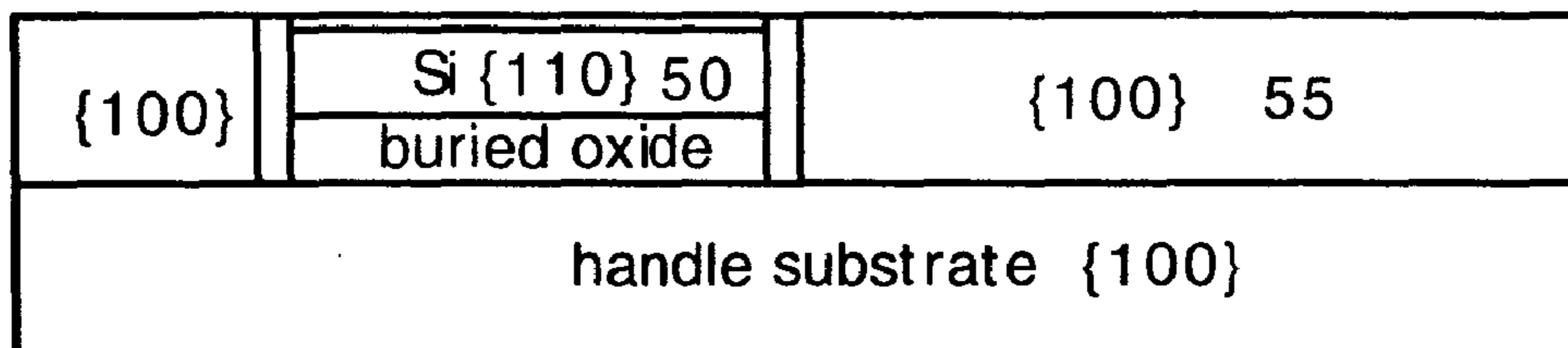
Fig. 3c Epitaxially grow substrate selectively
