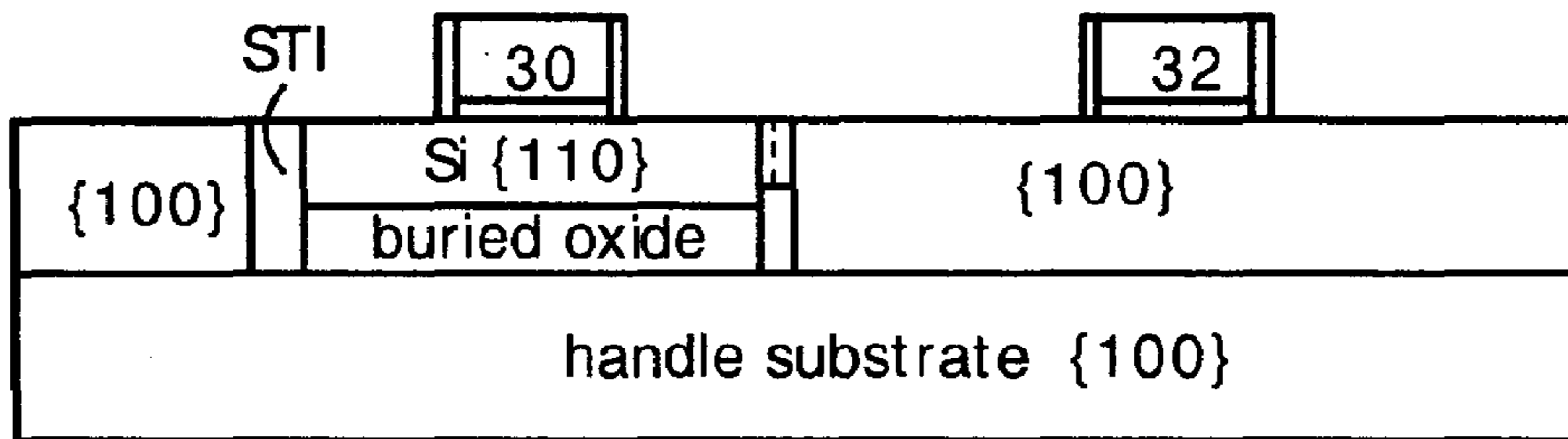
Fig. 3i Form gate electrodes and spacers
