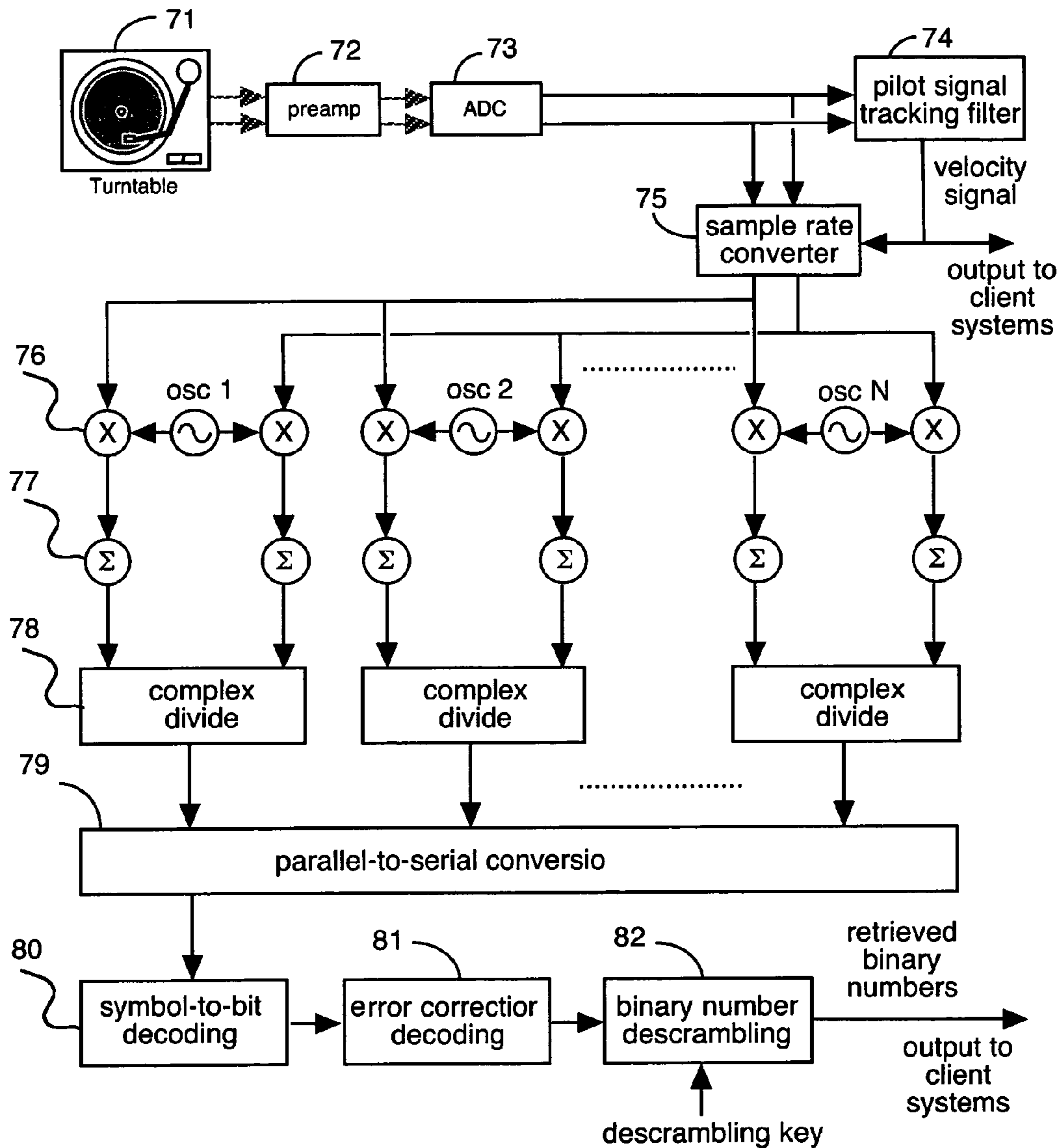
Figure 4. Processing system for recovering velocity and position information from samples.
