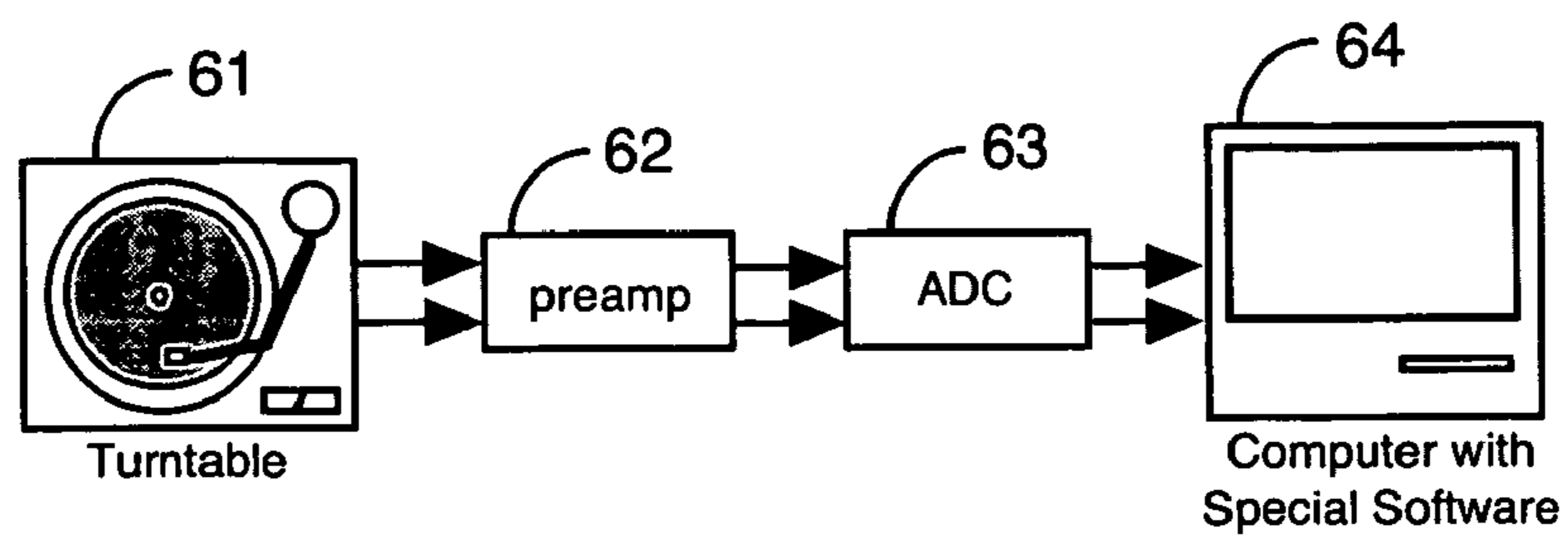
Figure 3. Simplest embodiment of the system for transducing velocity and position information according to present invention.
