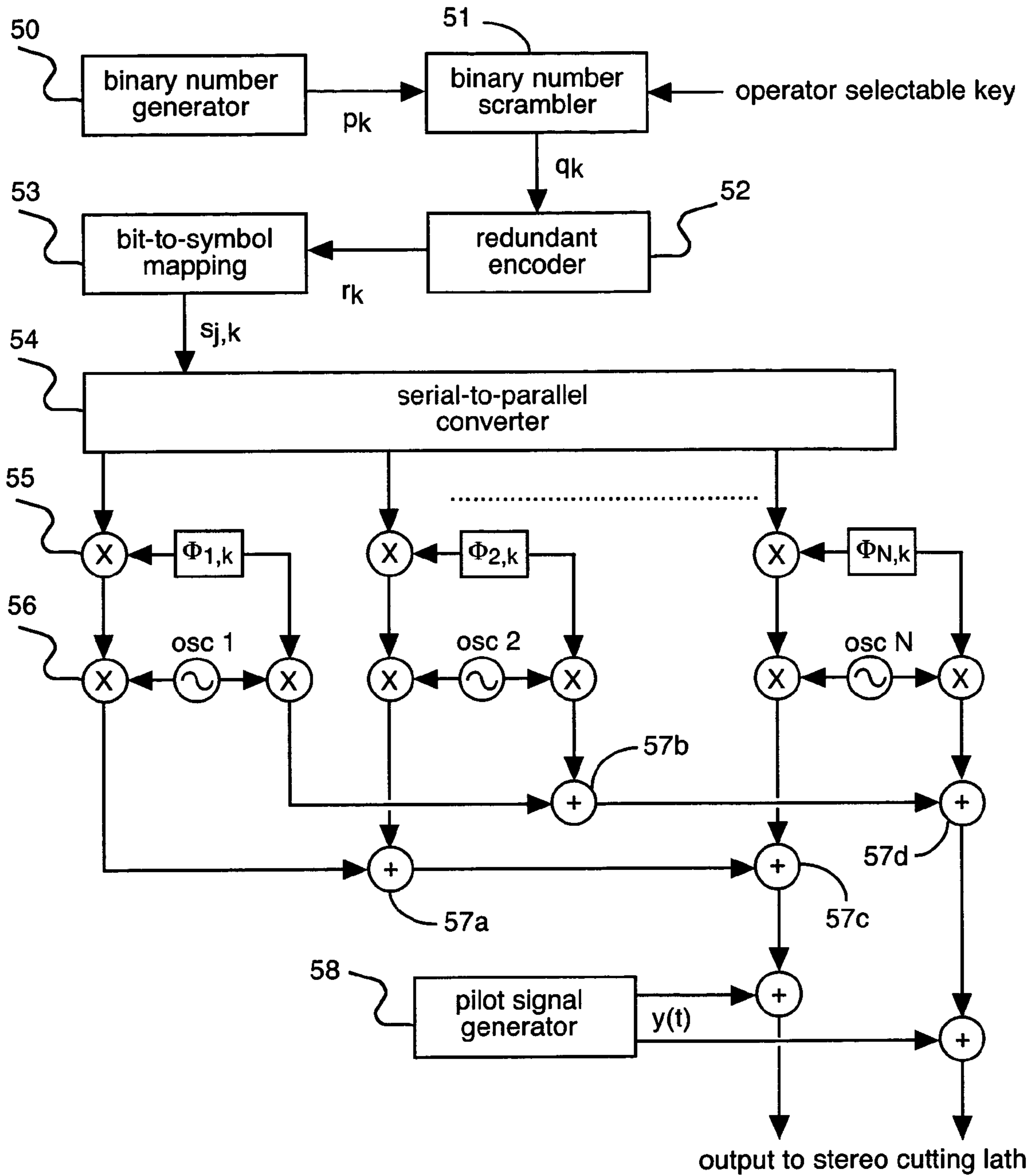
Figure 2. System for generating the signal to be recorded on the vinyl record.
