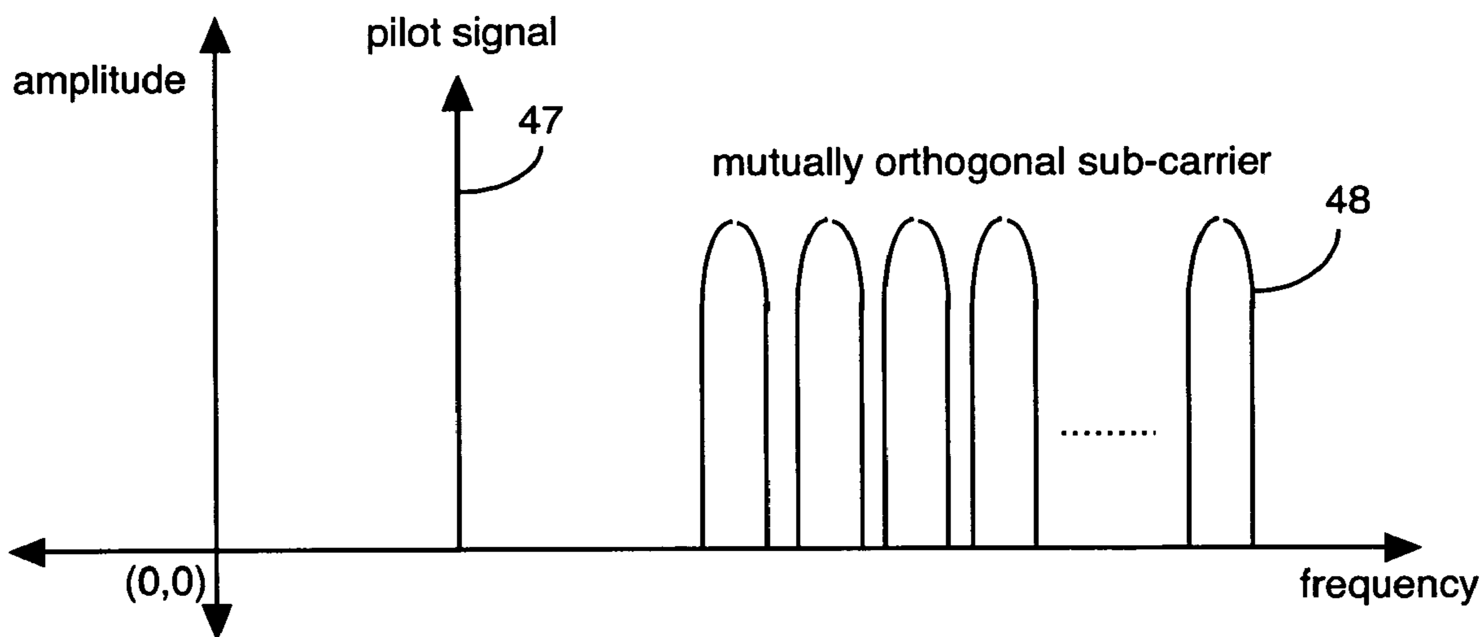
Frequency content of the signal to be recorded on the vinyl record.
