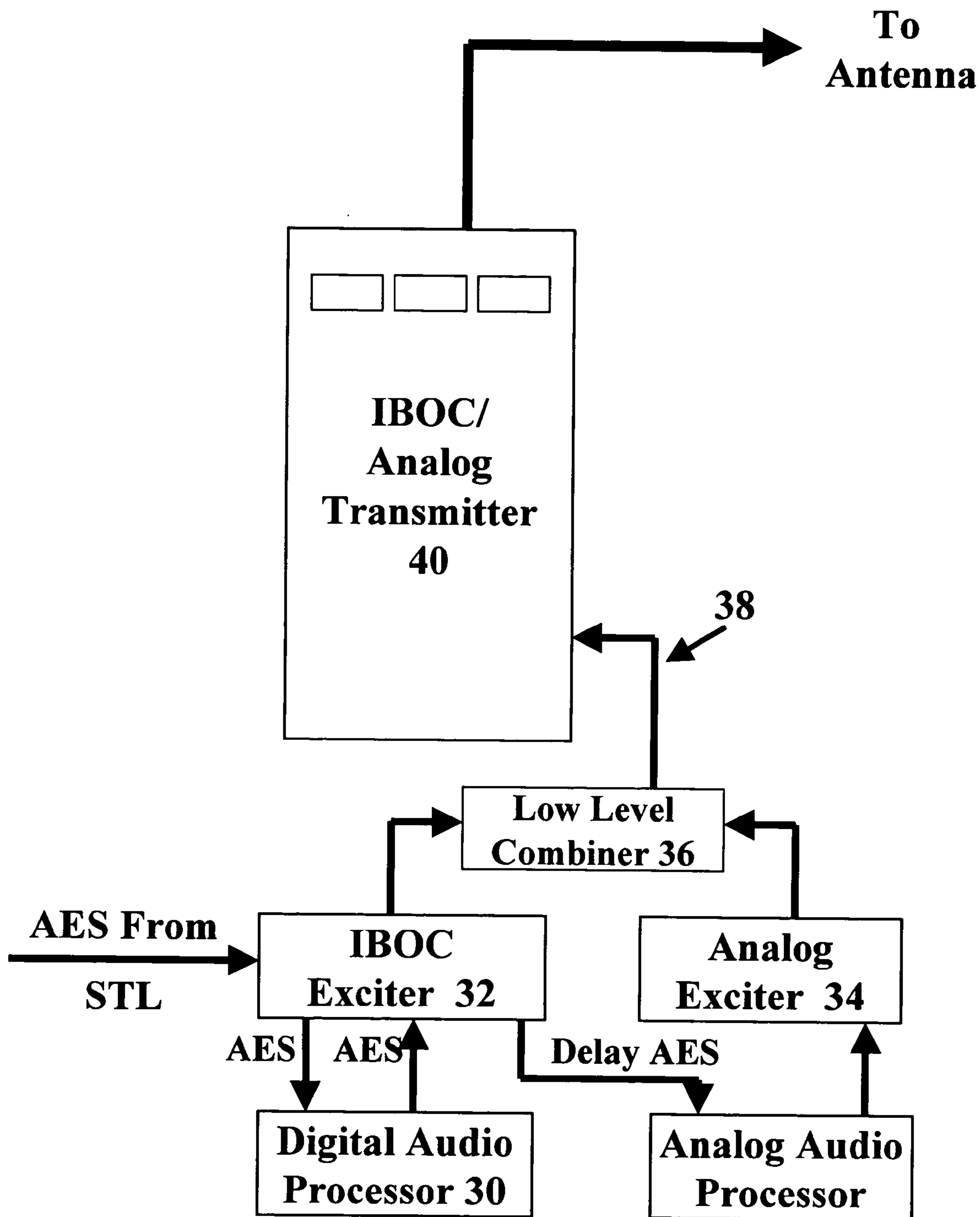
Fig. 2 (Prior Art)
