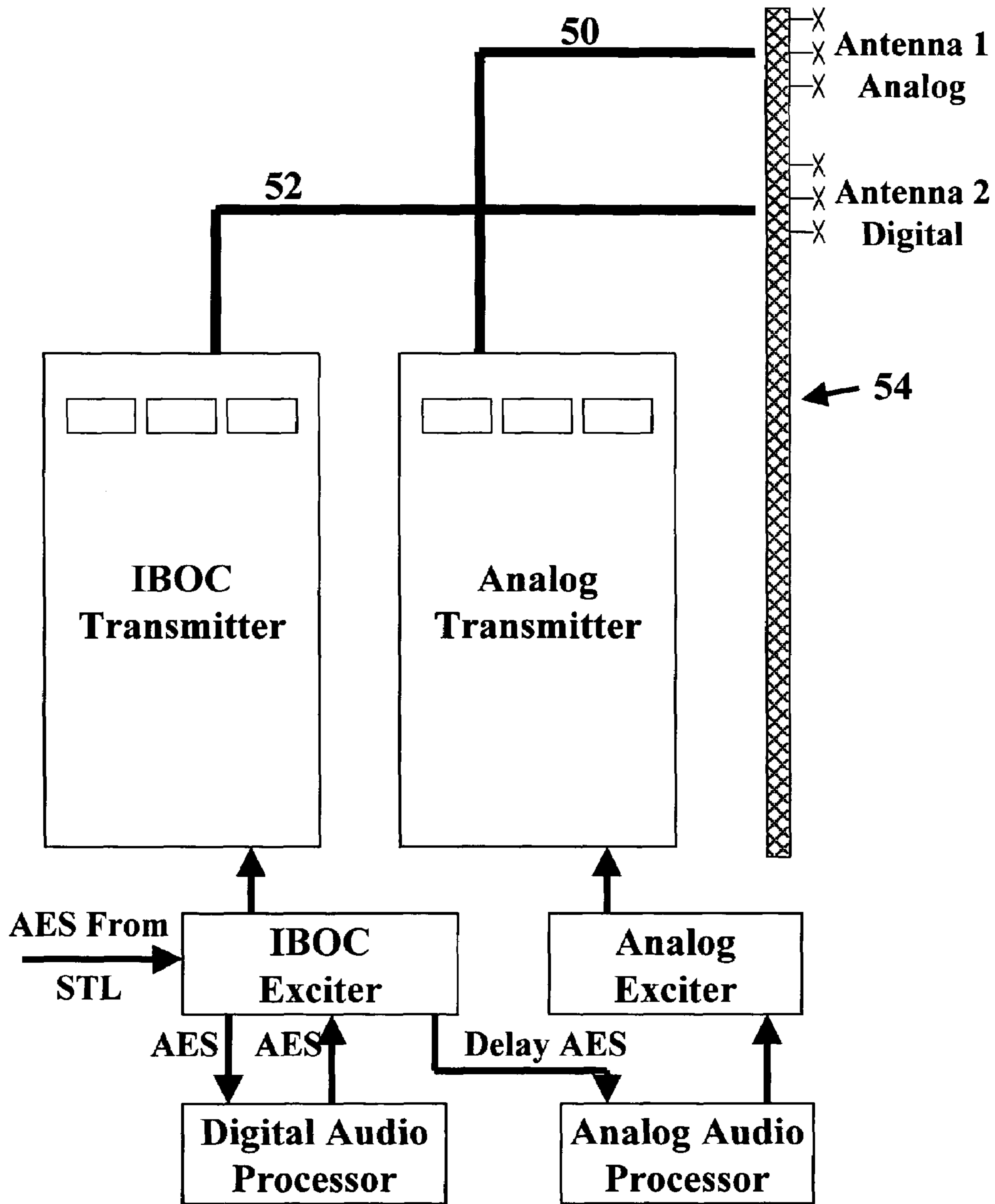
Fig. 3 (Prior Art)
