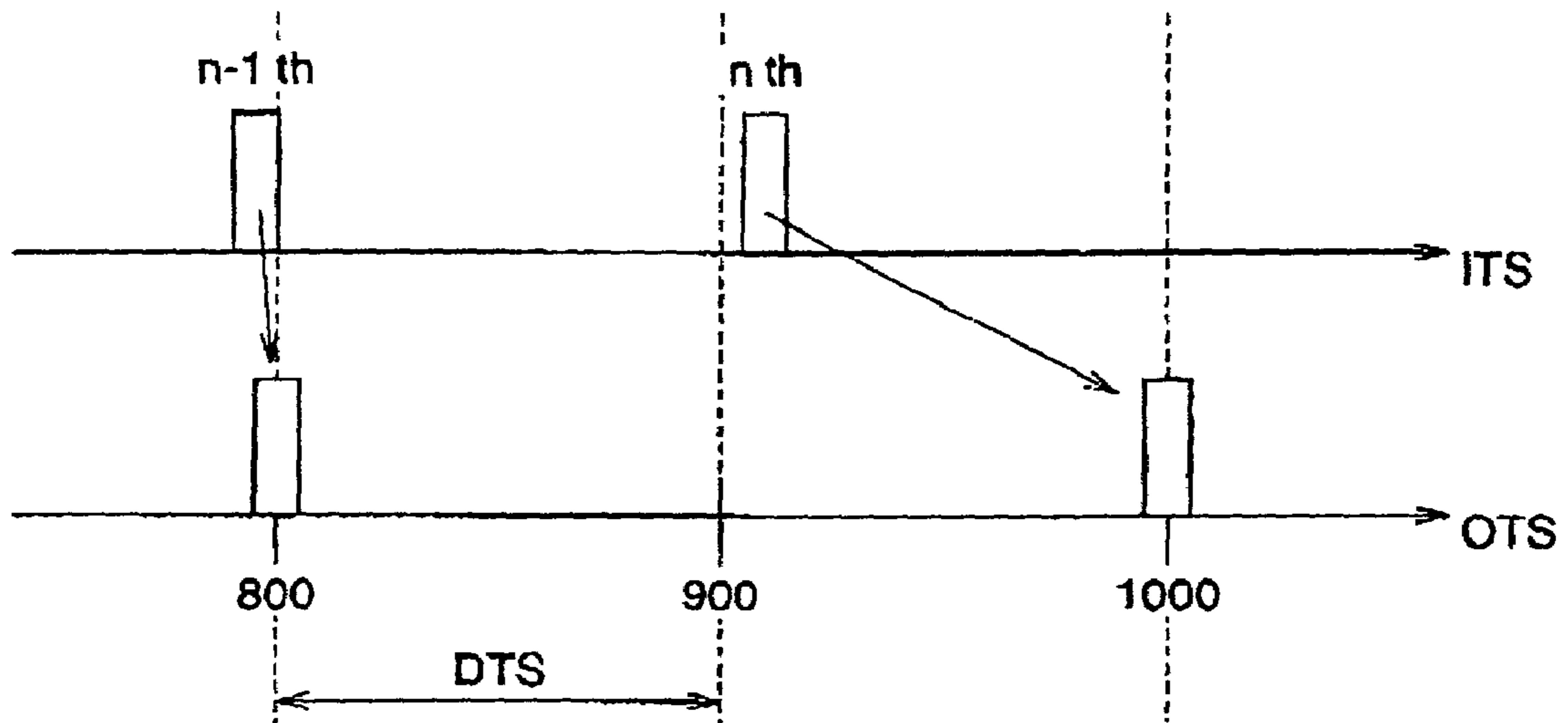
Fig.7 (a) ITS \leq OTS
