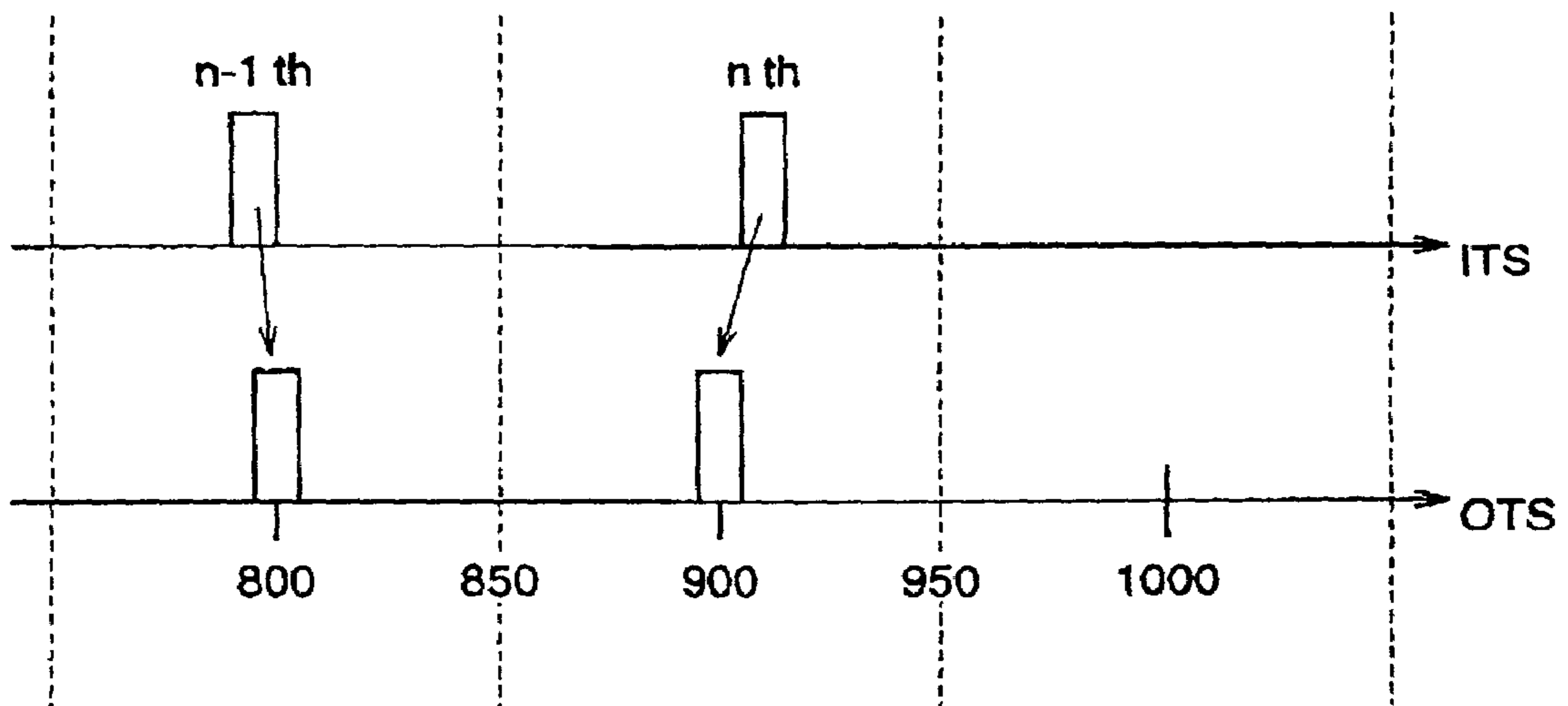
Fig.7 (b) ITS \leq OTS + DTS/2
