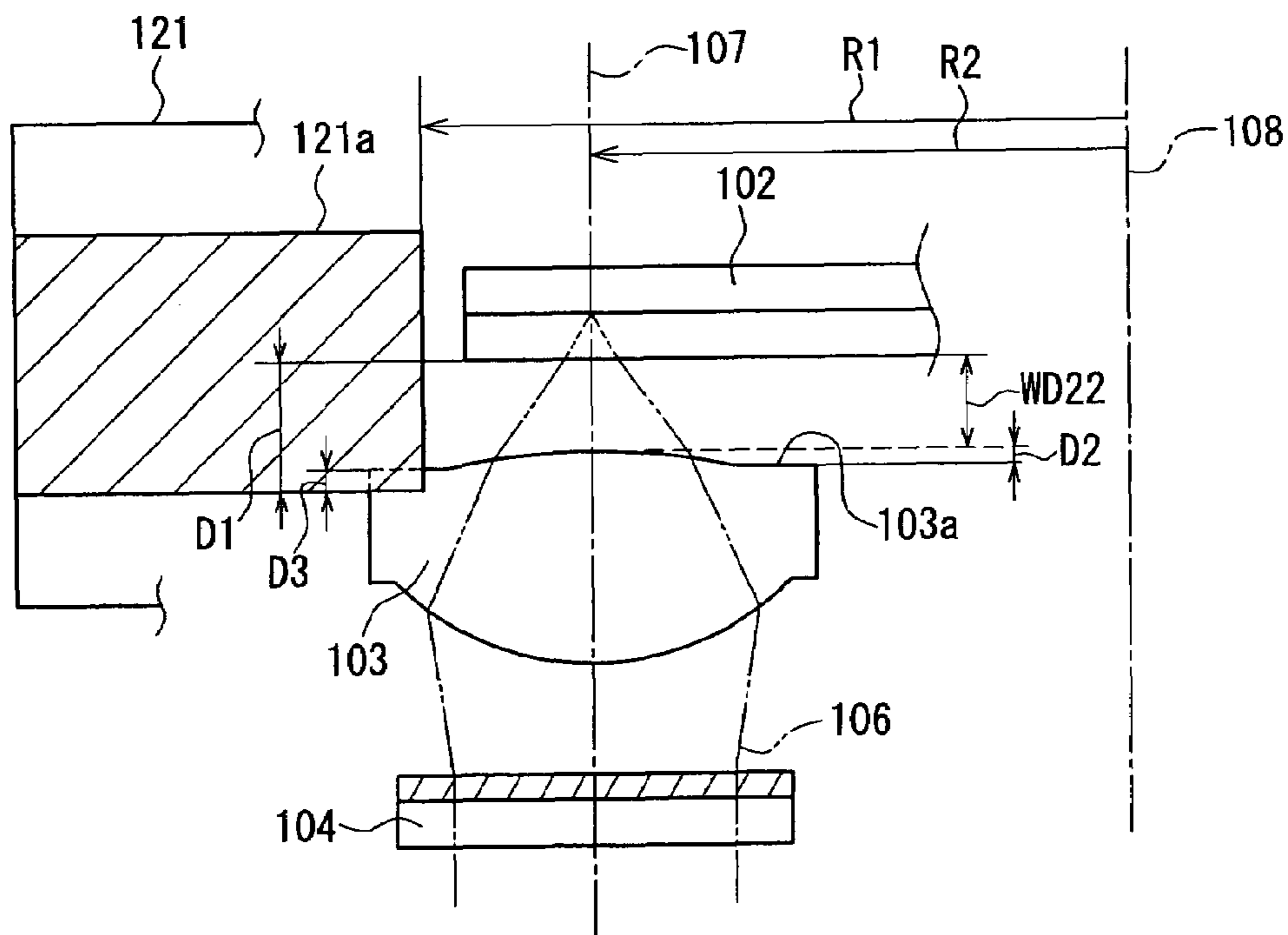
FIG. 5 PRIOR ART
