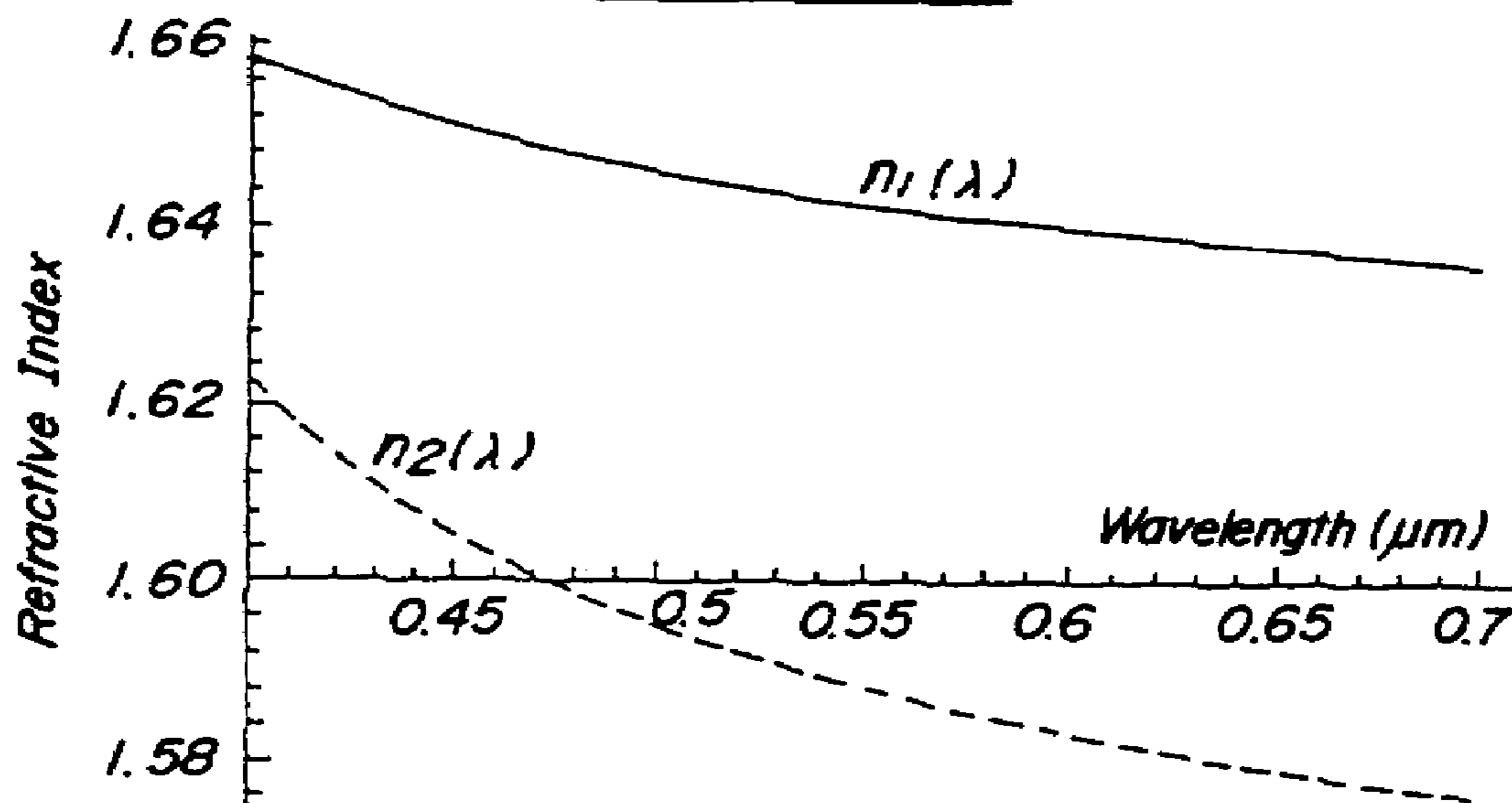
FIG. 5 PRIOR ART
