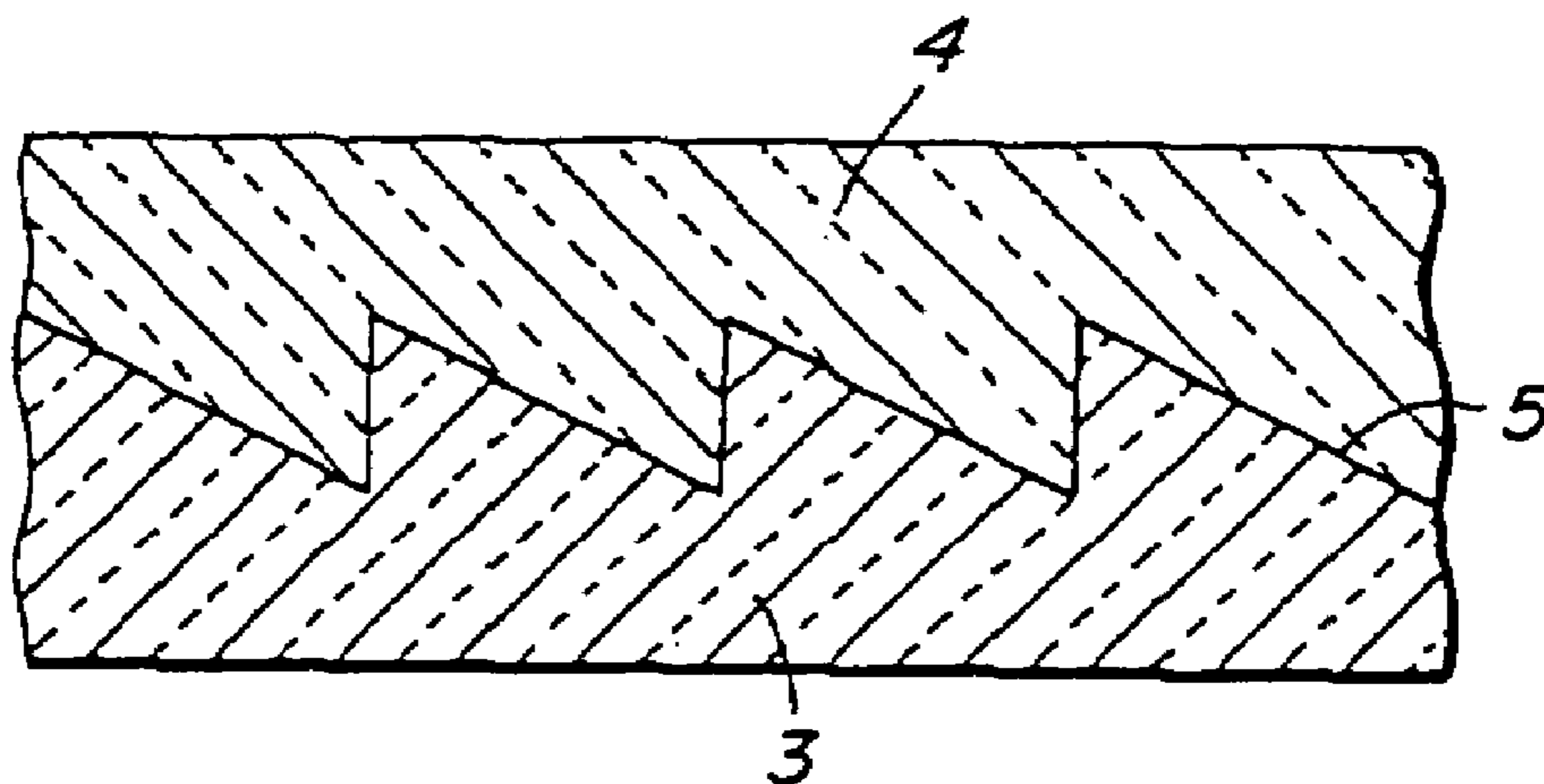
FIG. 4 PRIOR ART
