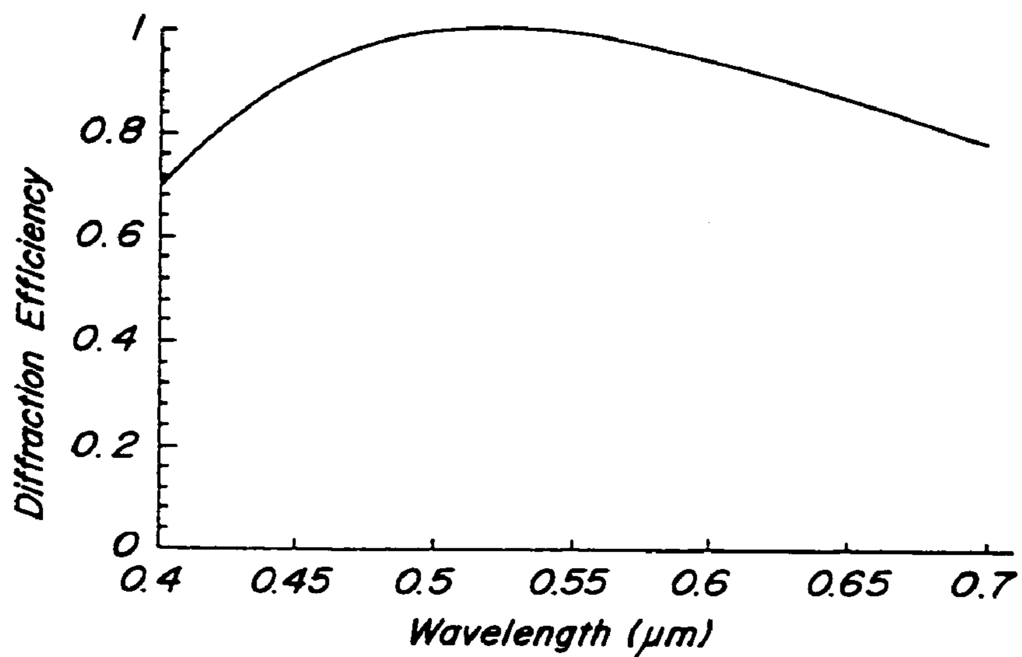
FIG. 2 PRIOR ART
