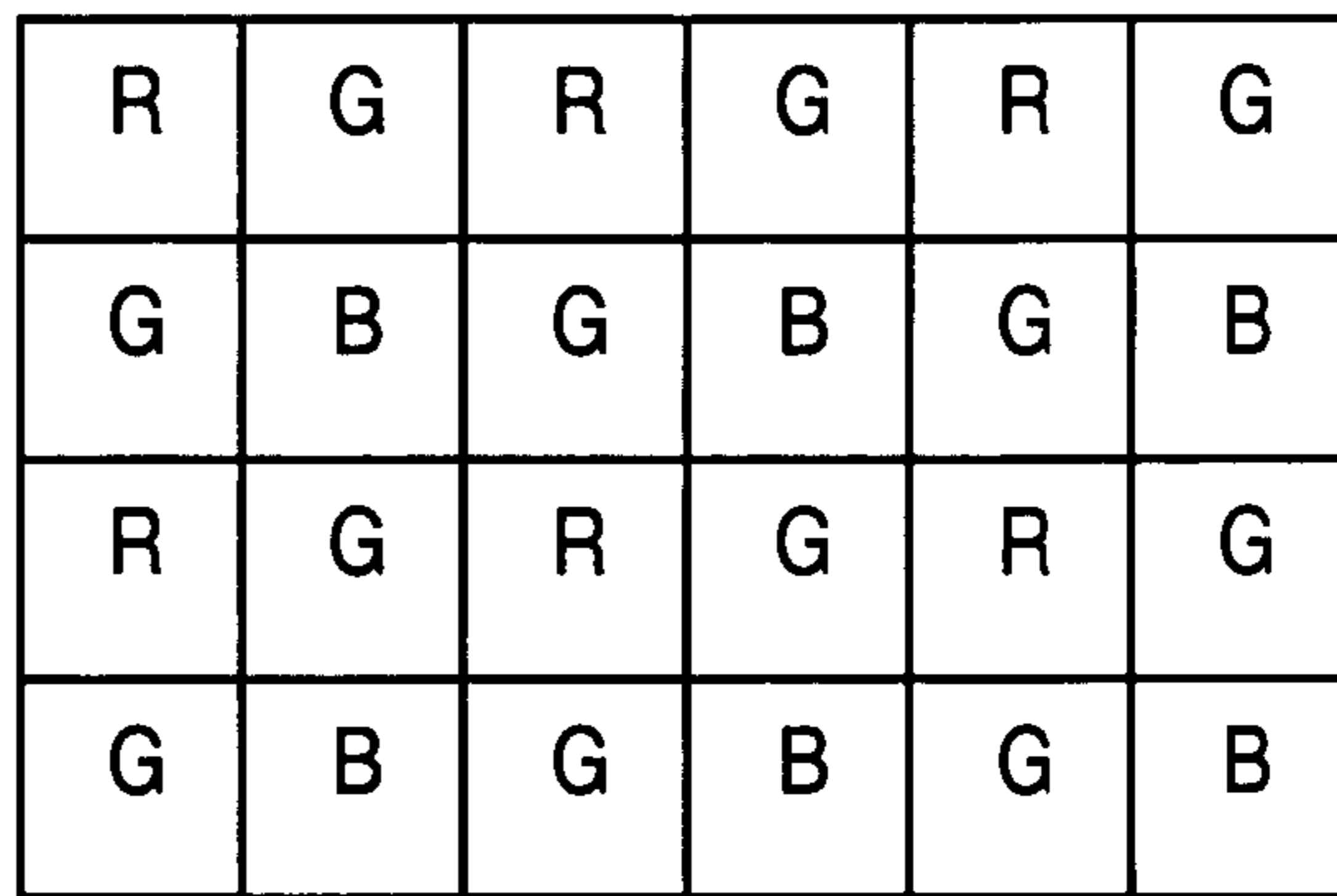
Bayer mosaic of several 2x2 pixel blocks
