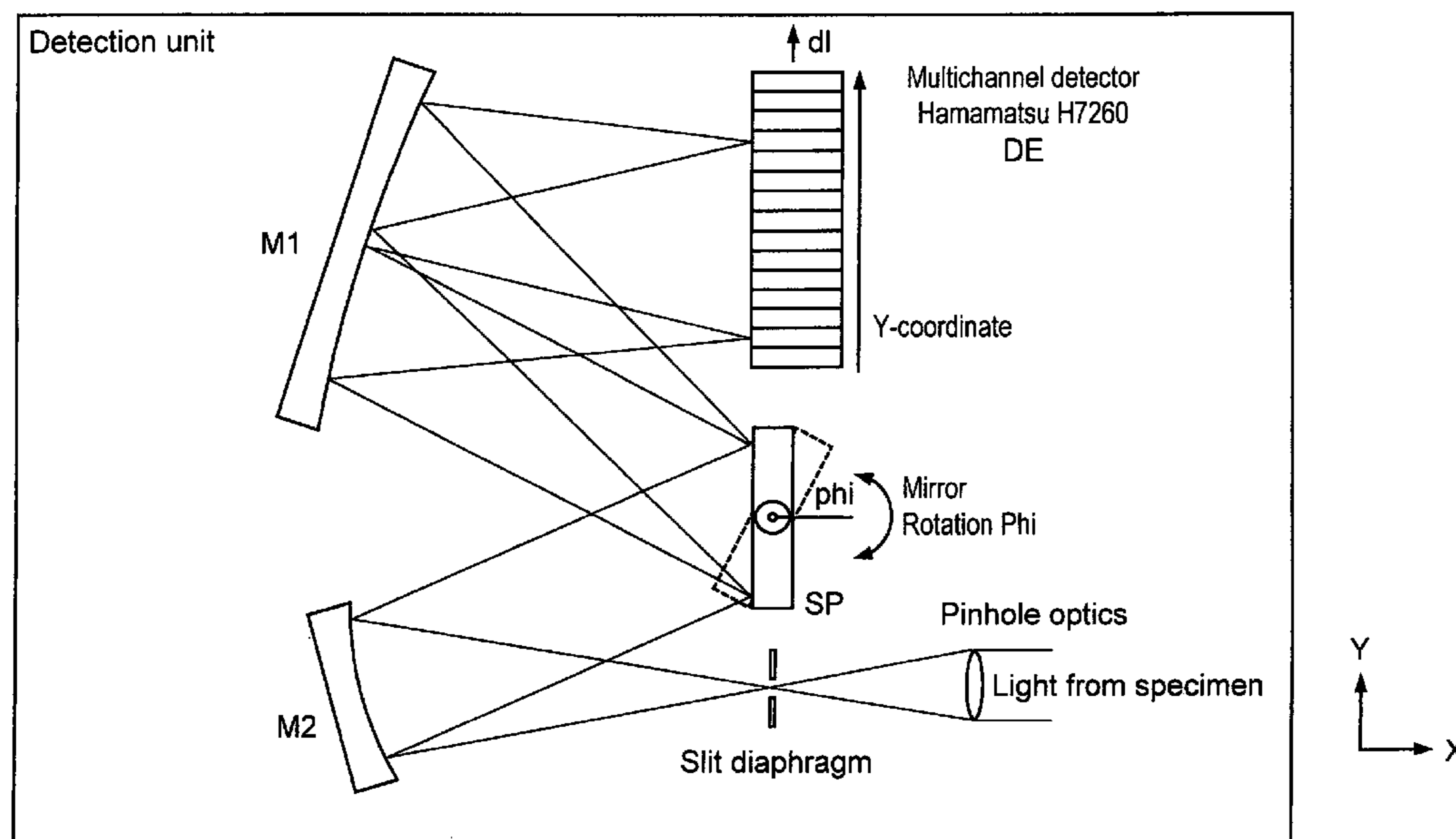
Example of detector unit / optics construction for line scanner
