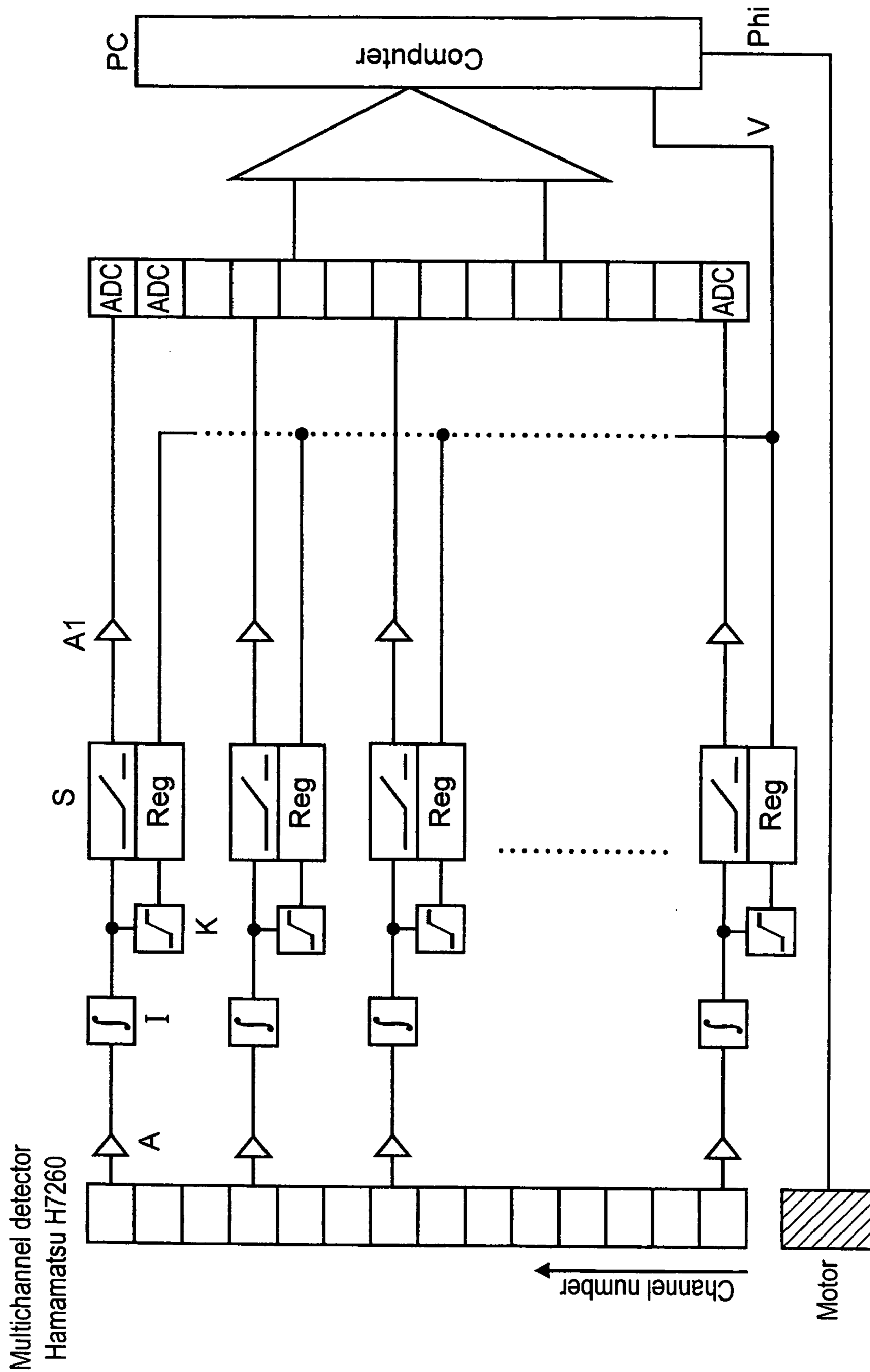
FIG. 12. Example for construction of electronics
