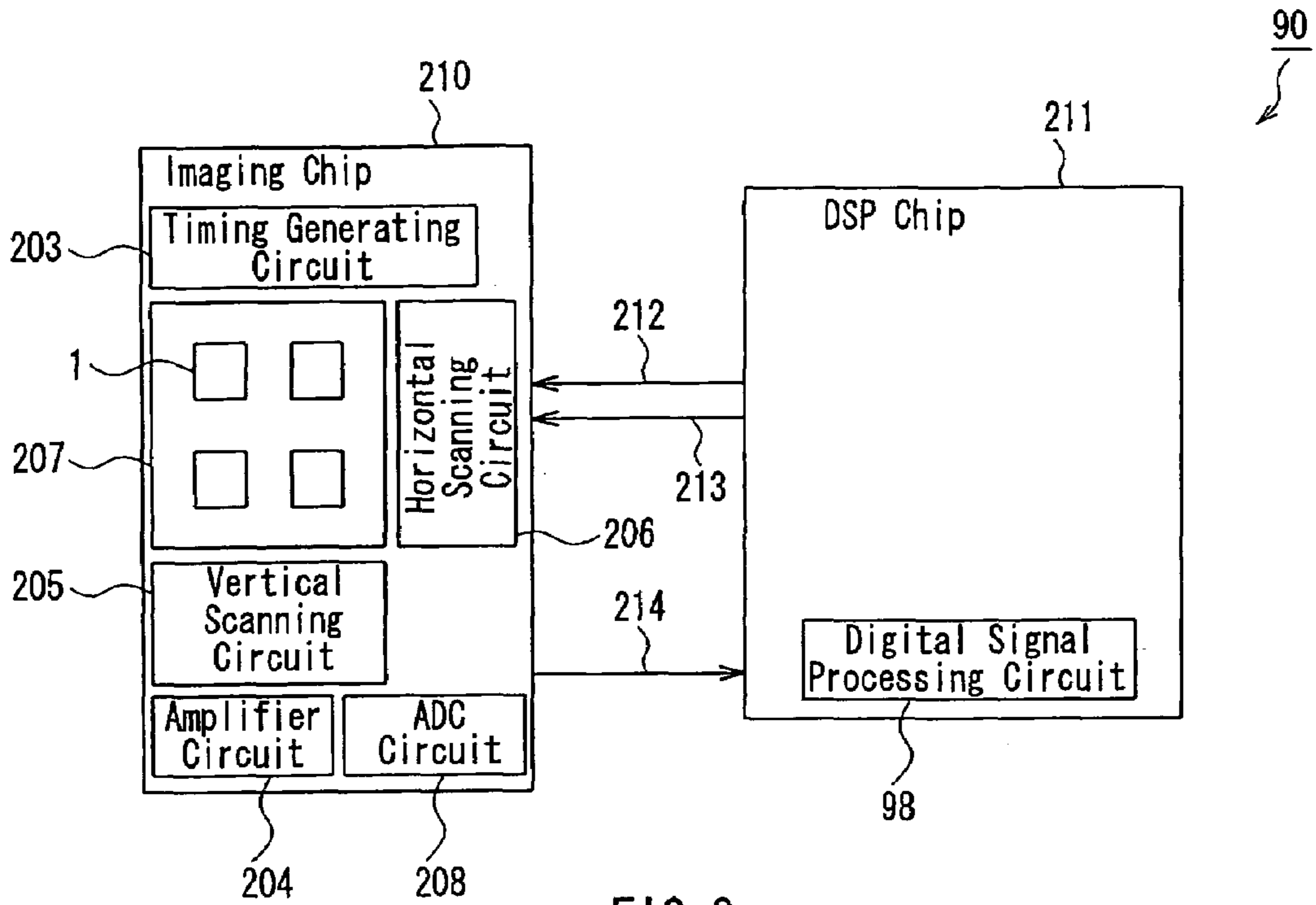
FIG. 8 PRIOR ART
