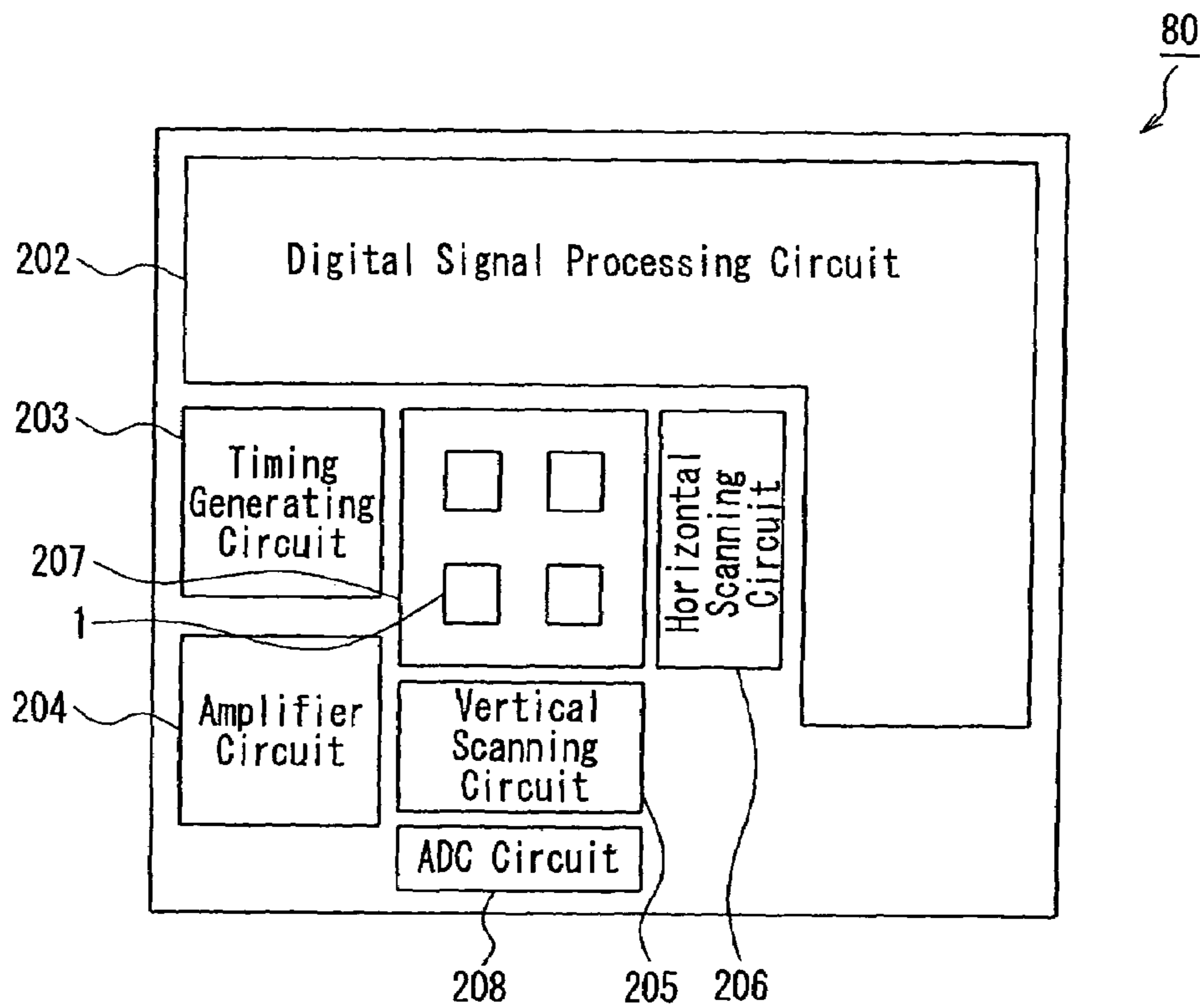
FIG. 7 PRIOR ART
