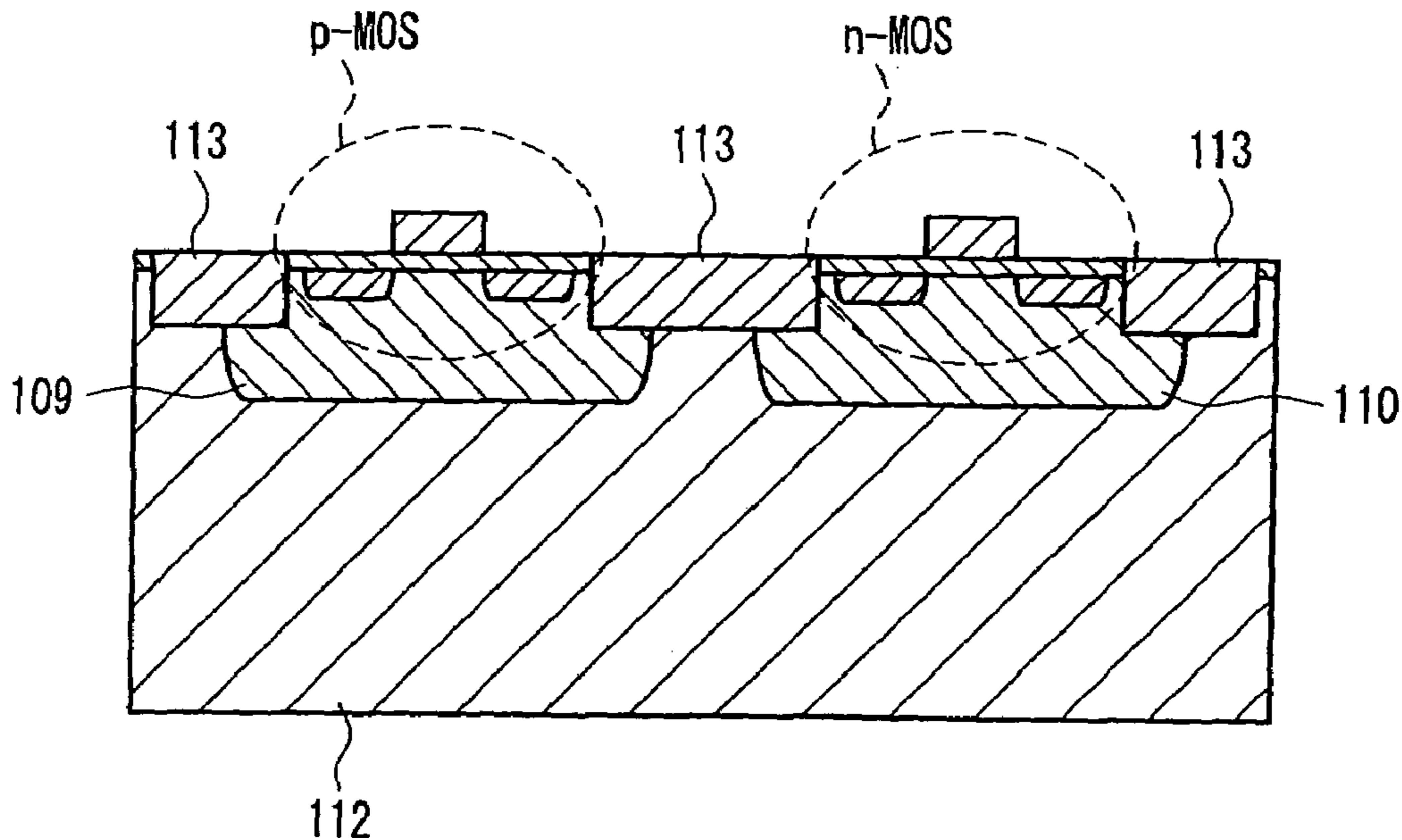
FIG. 11 PRIOR ART
