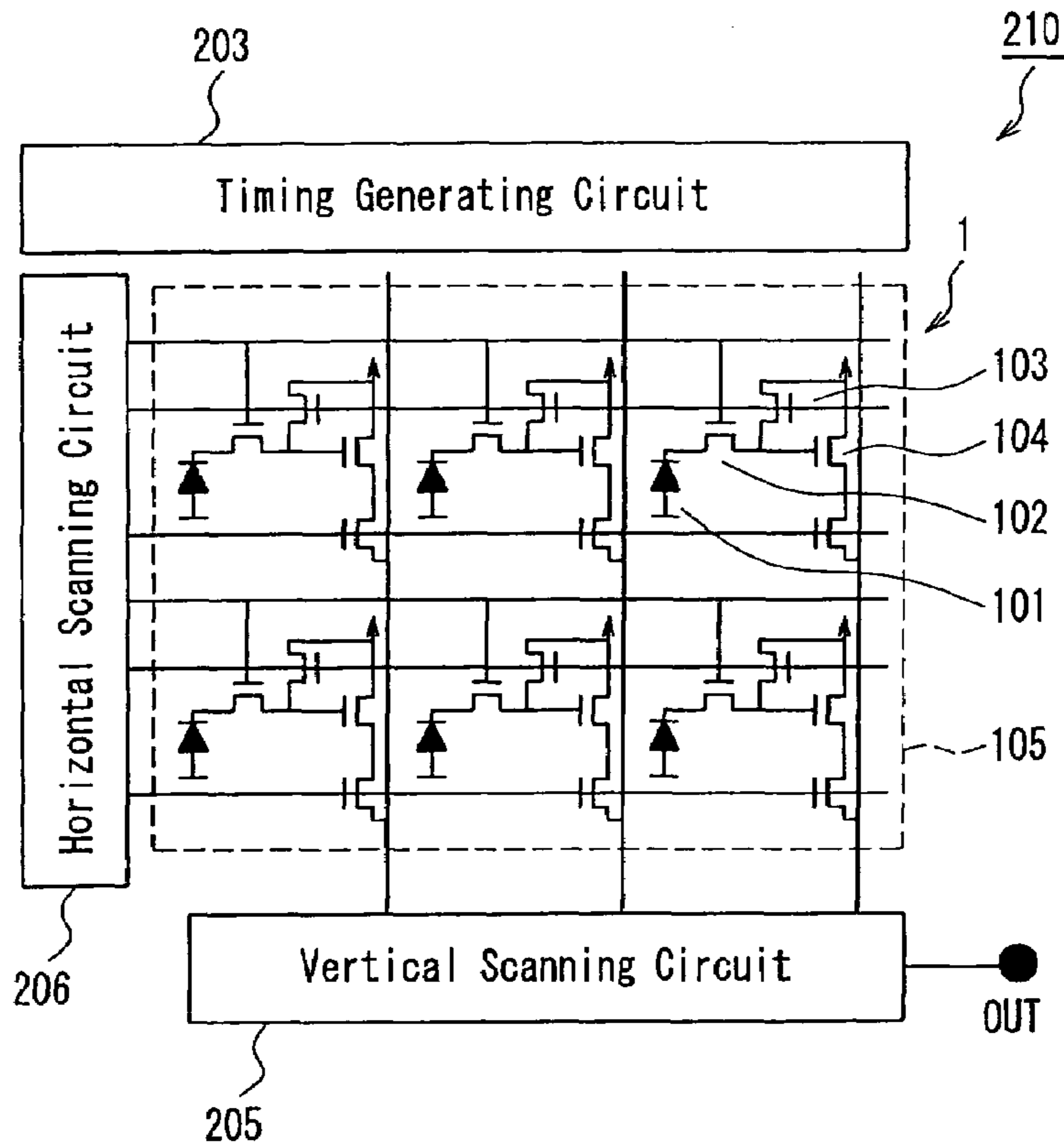
FIG. 9 PRIOR ART
