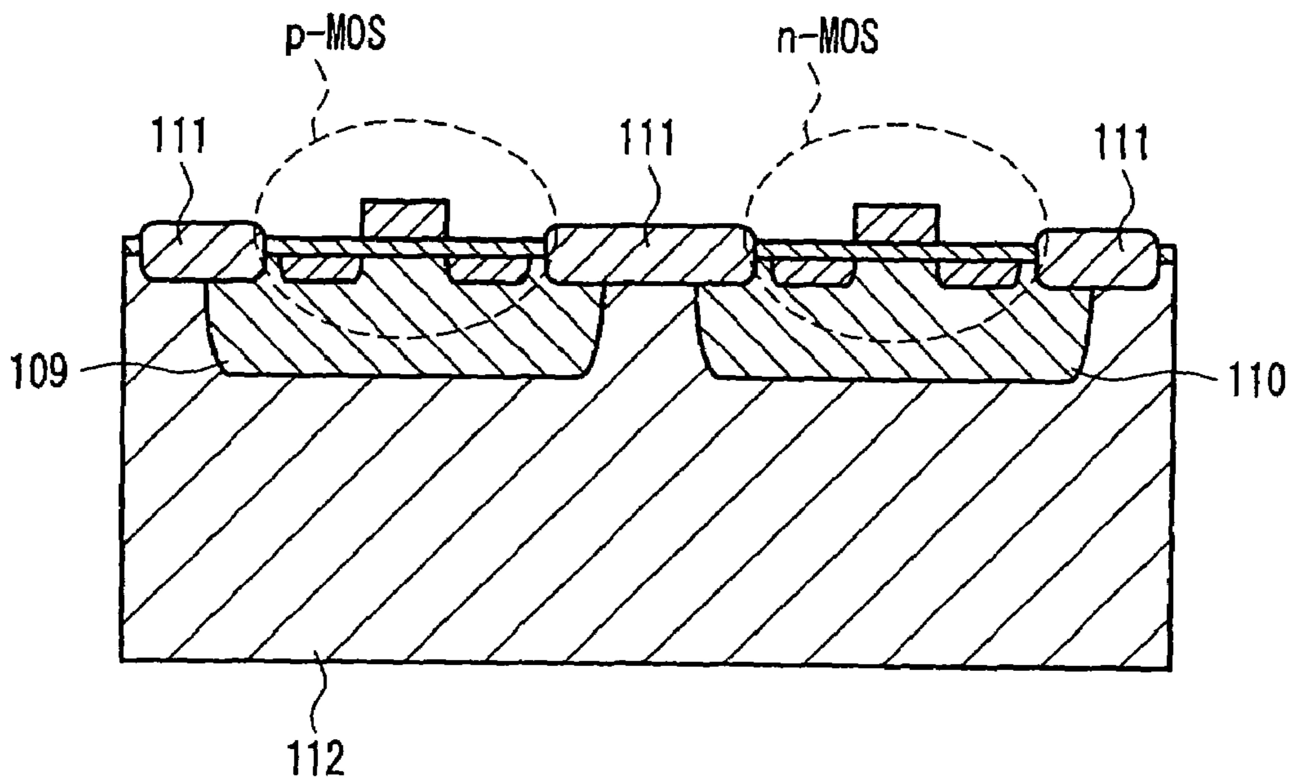
FIG. 10 PRIOR ART
