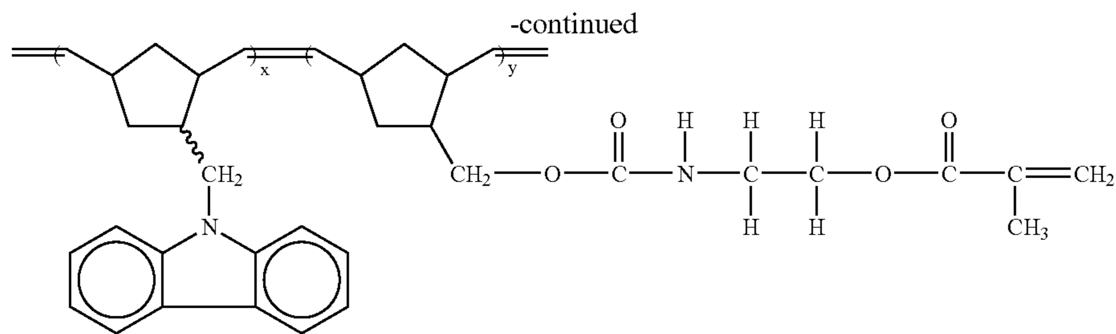
Poly(CbzNB-b-NBMOAC)
