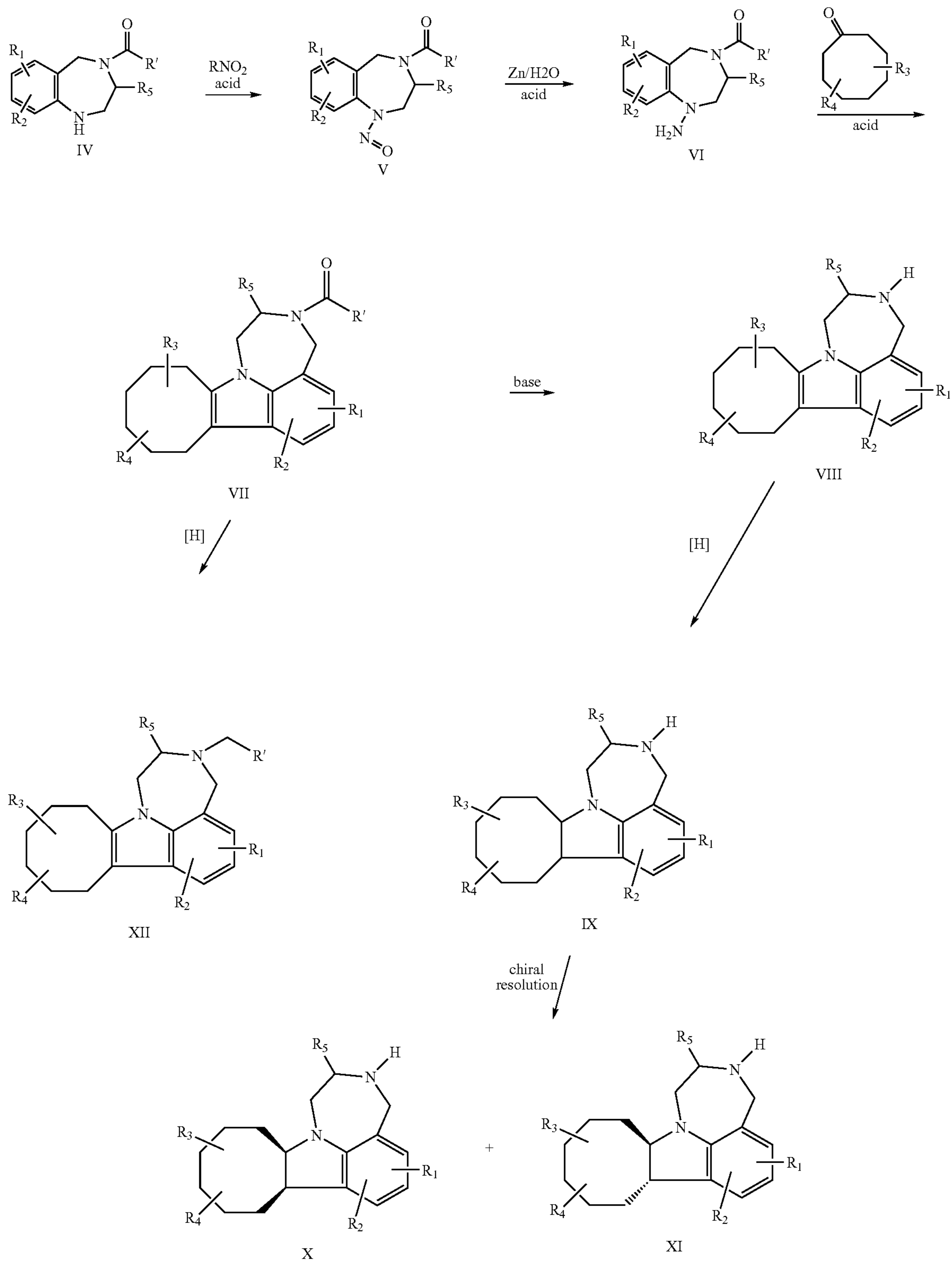
Scheme 2
