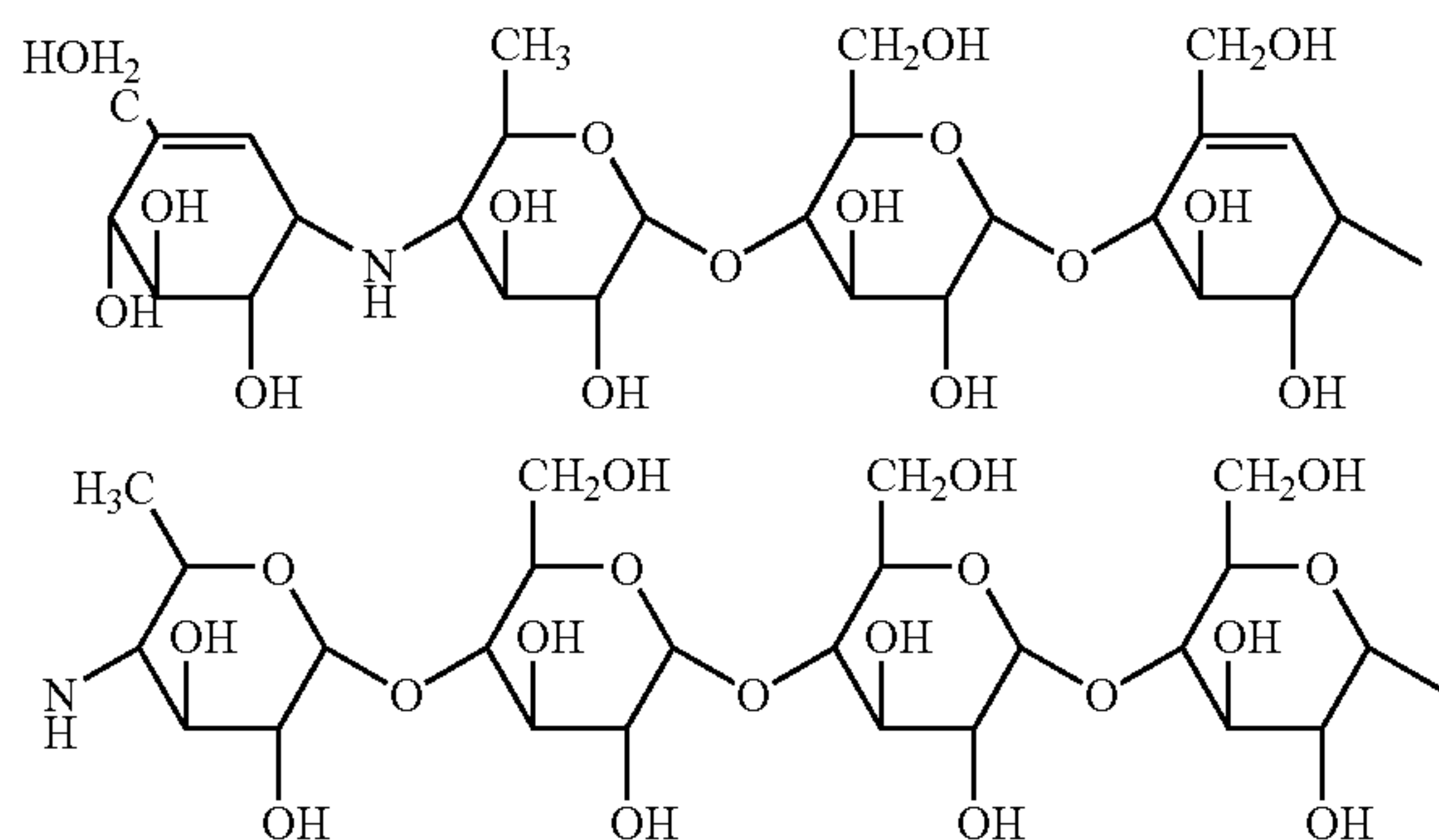
ACARBOSE
