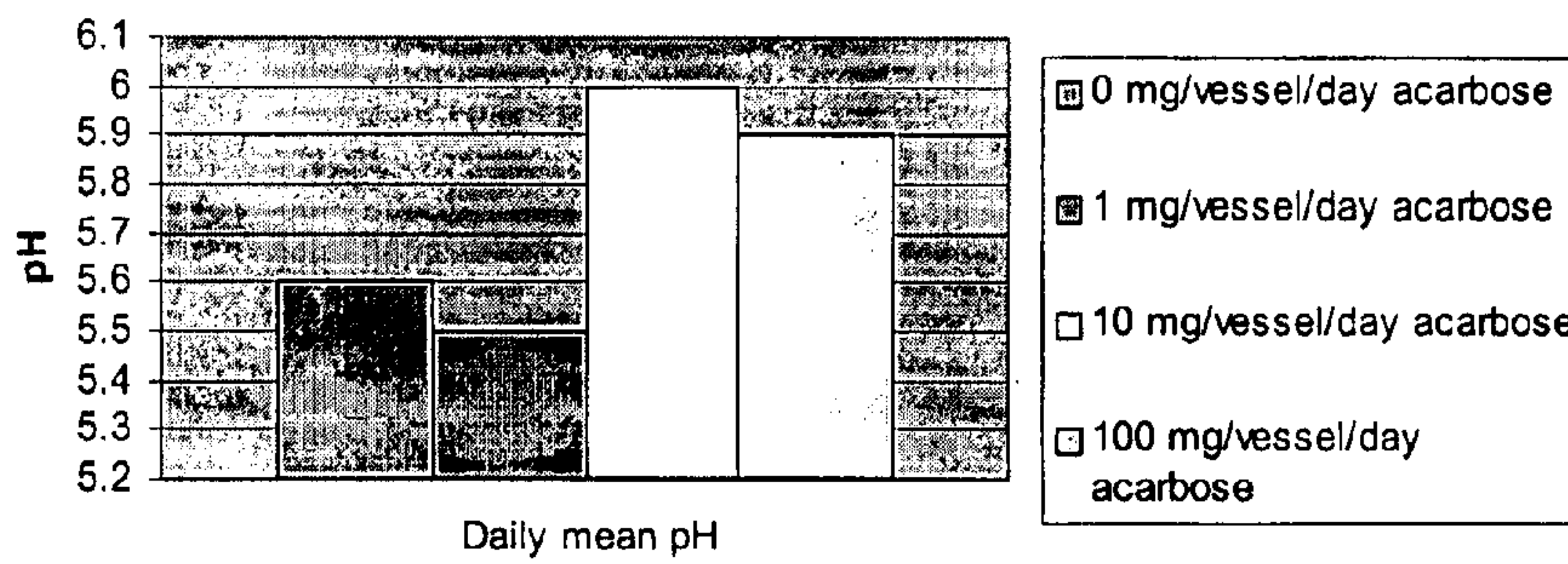
Daily mean pH in Rusitec chronic acidosis model treated with acarbose
