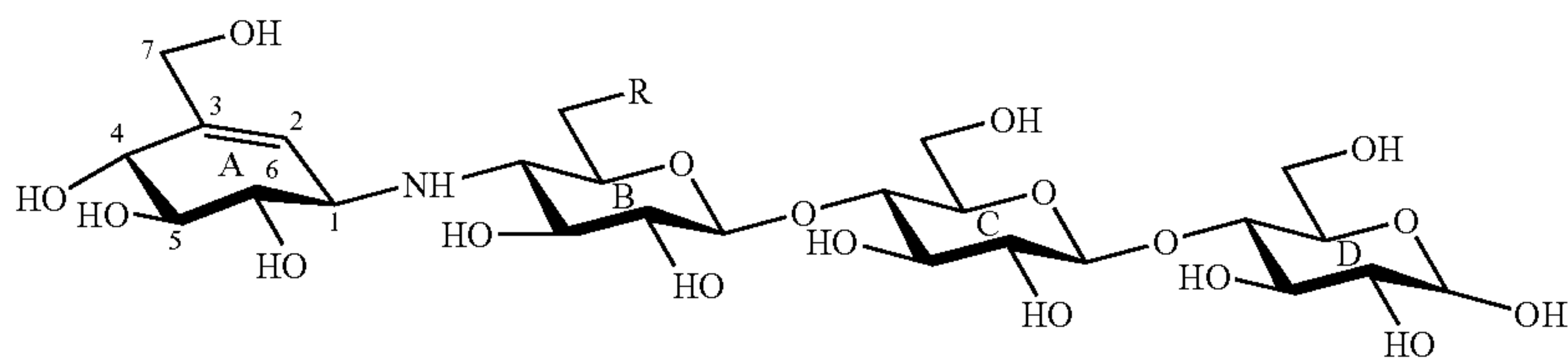
2a beta-acarbose
