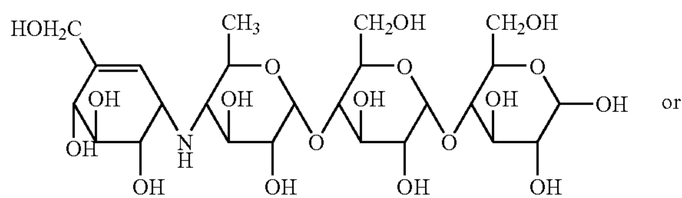
ACARBOSE
