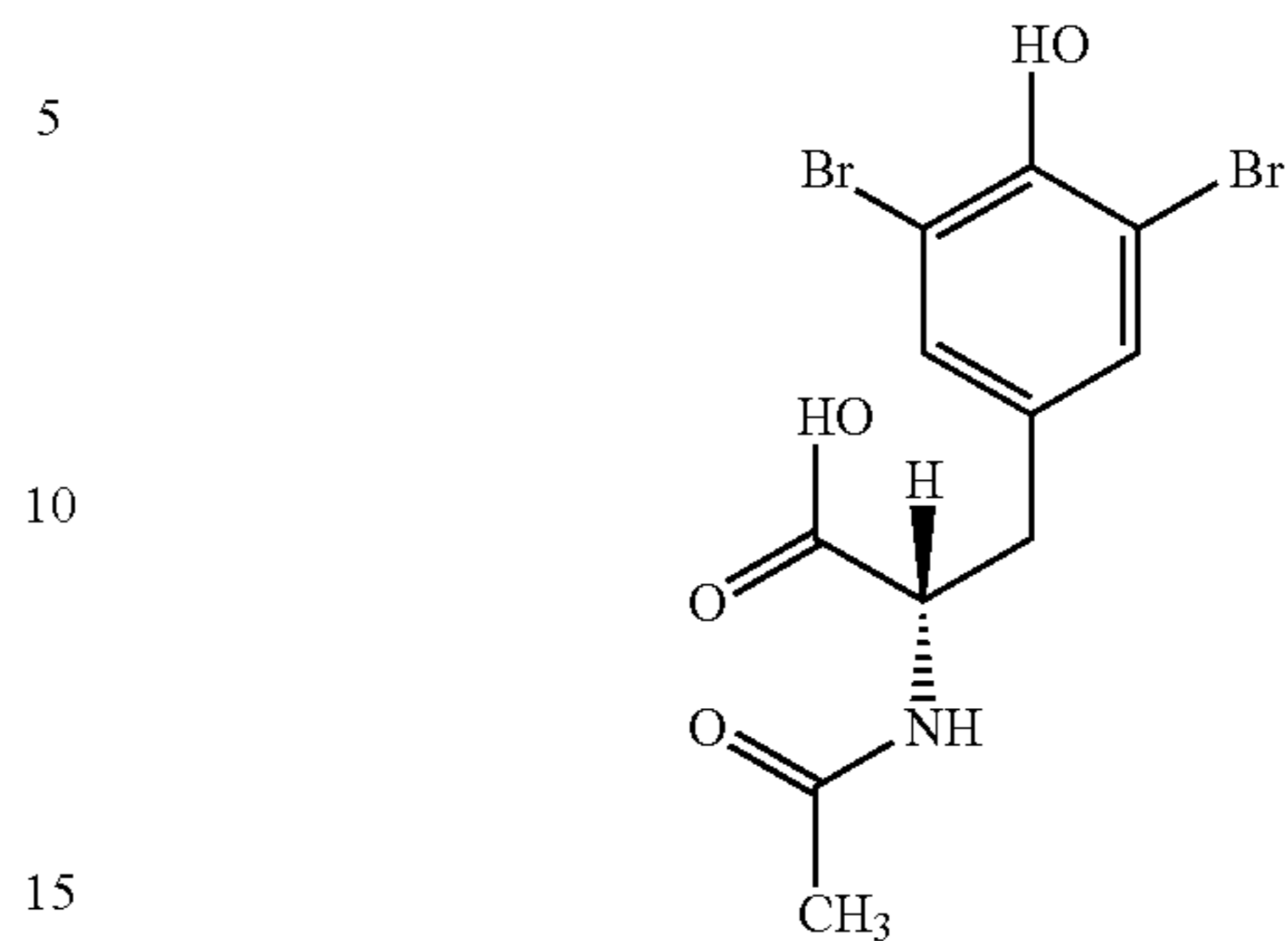
N-acetyl-3,5-dibromo-L-tyrosine
