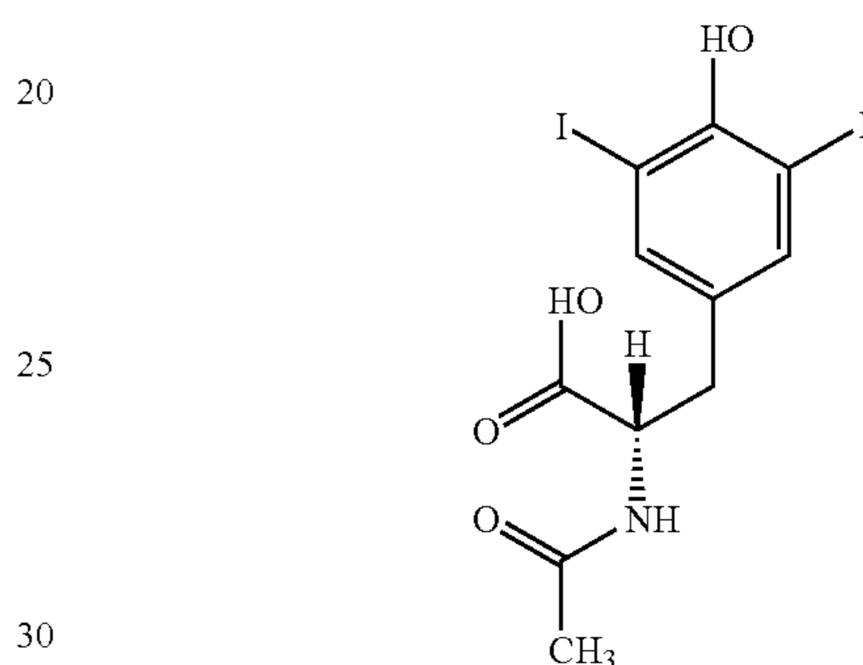
N-acetyl-3,5-diiodo-L-tyrosine
