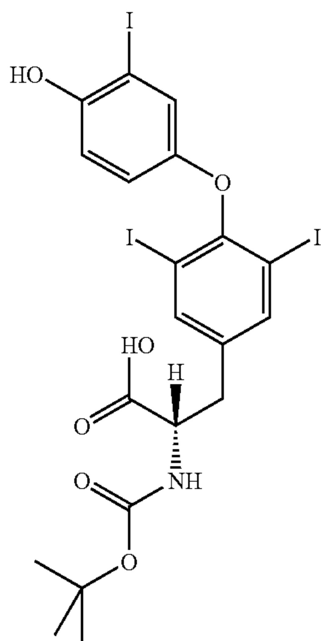
N-tert-butylloxycarbonyl-3',3,5-triiodo-L-thyronine
