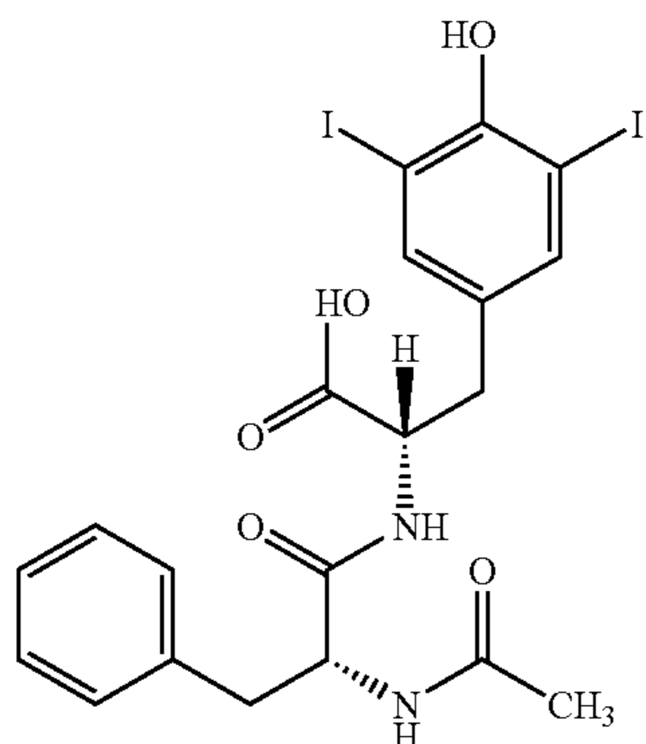
N-acetylphenylalanyl-3,5-diiodo-L-tyrosine
