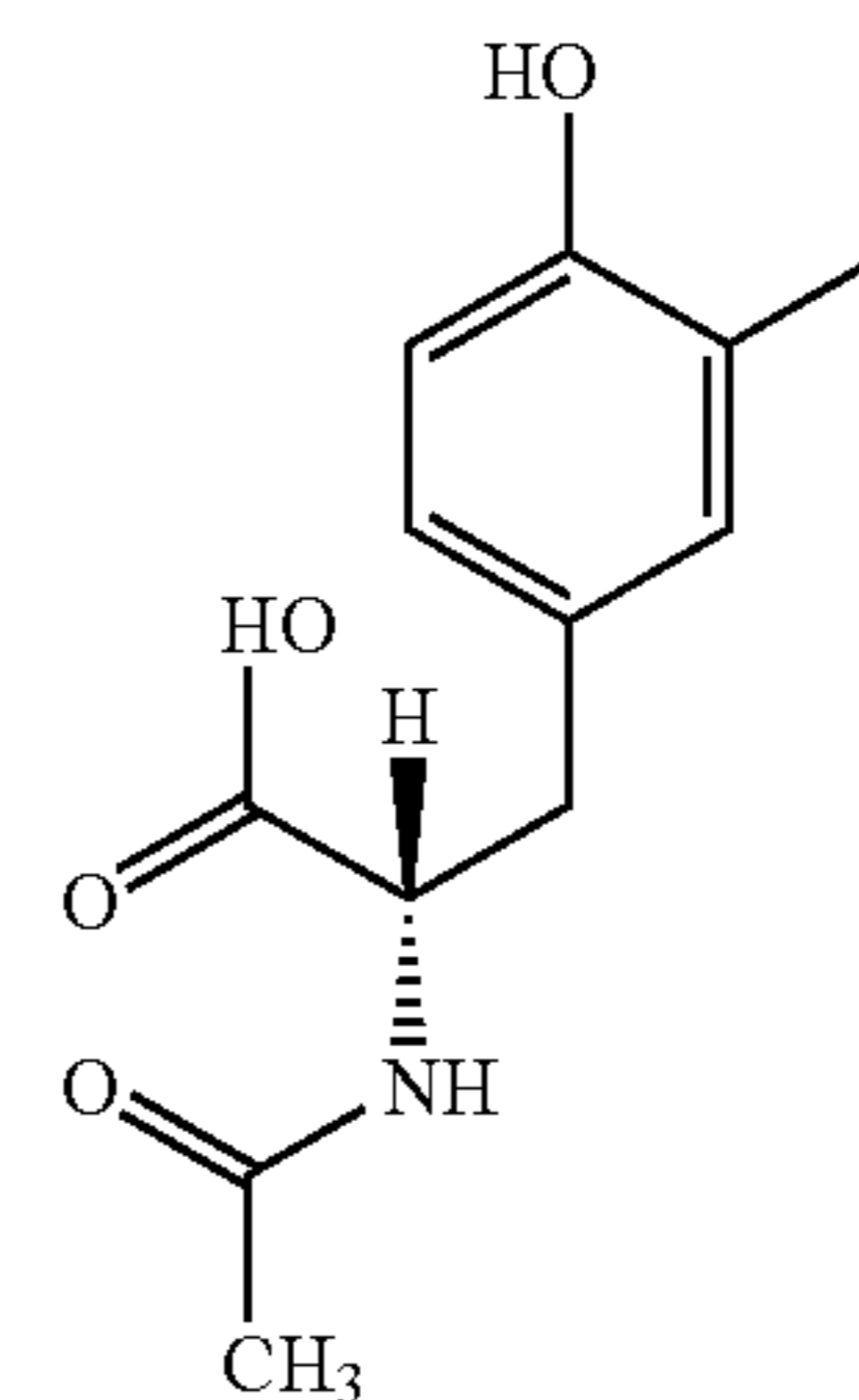
N-acetyl-3-iodo-L-tyrosine
