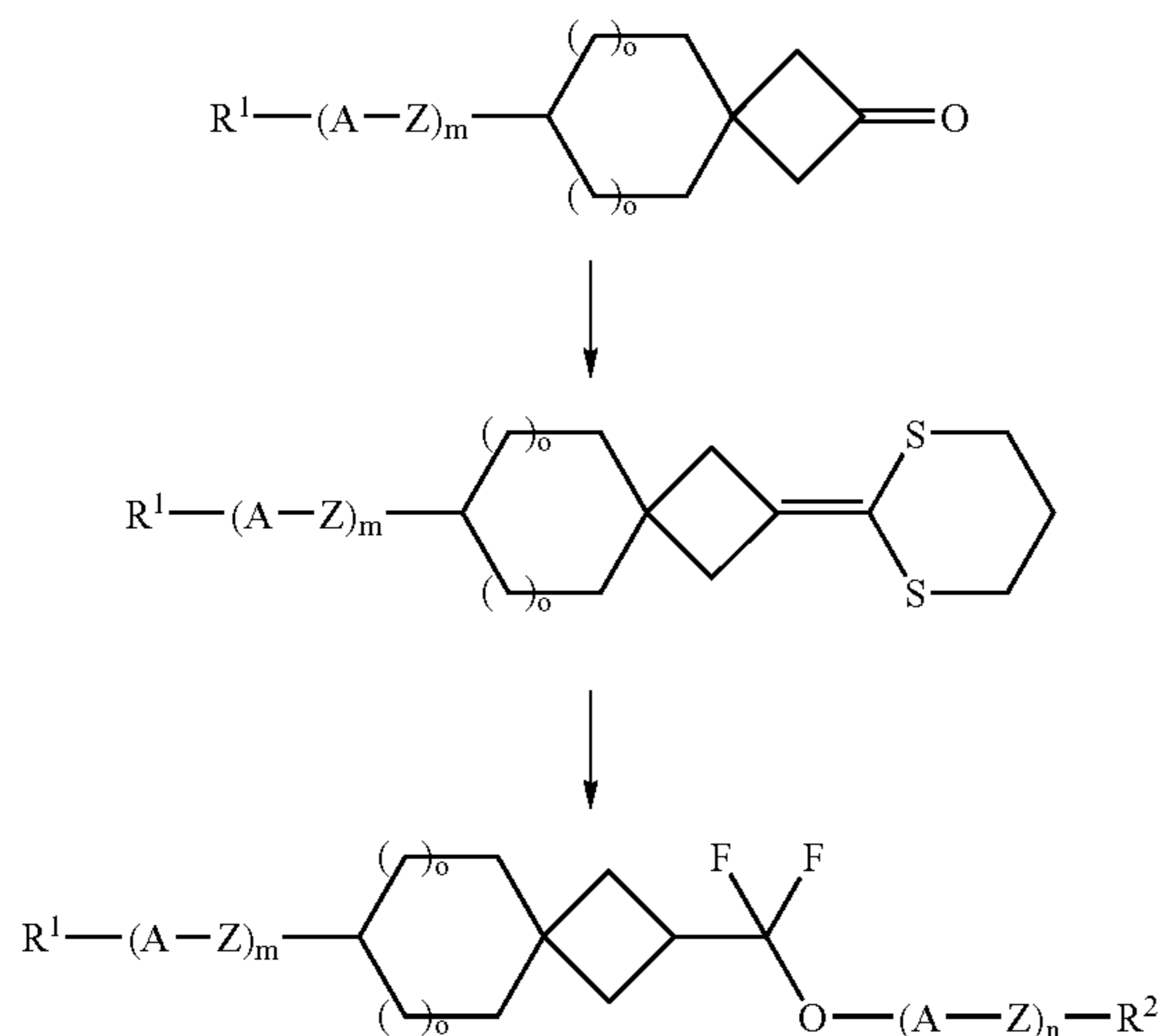
Scheme 1:
