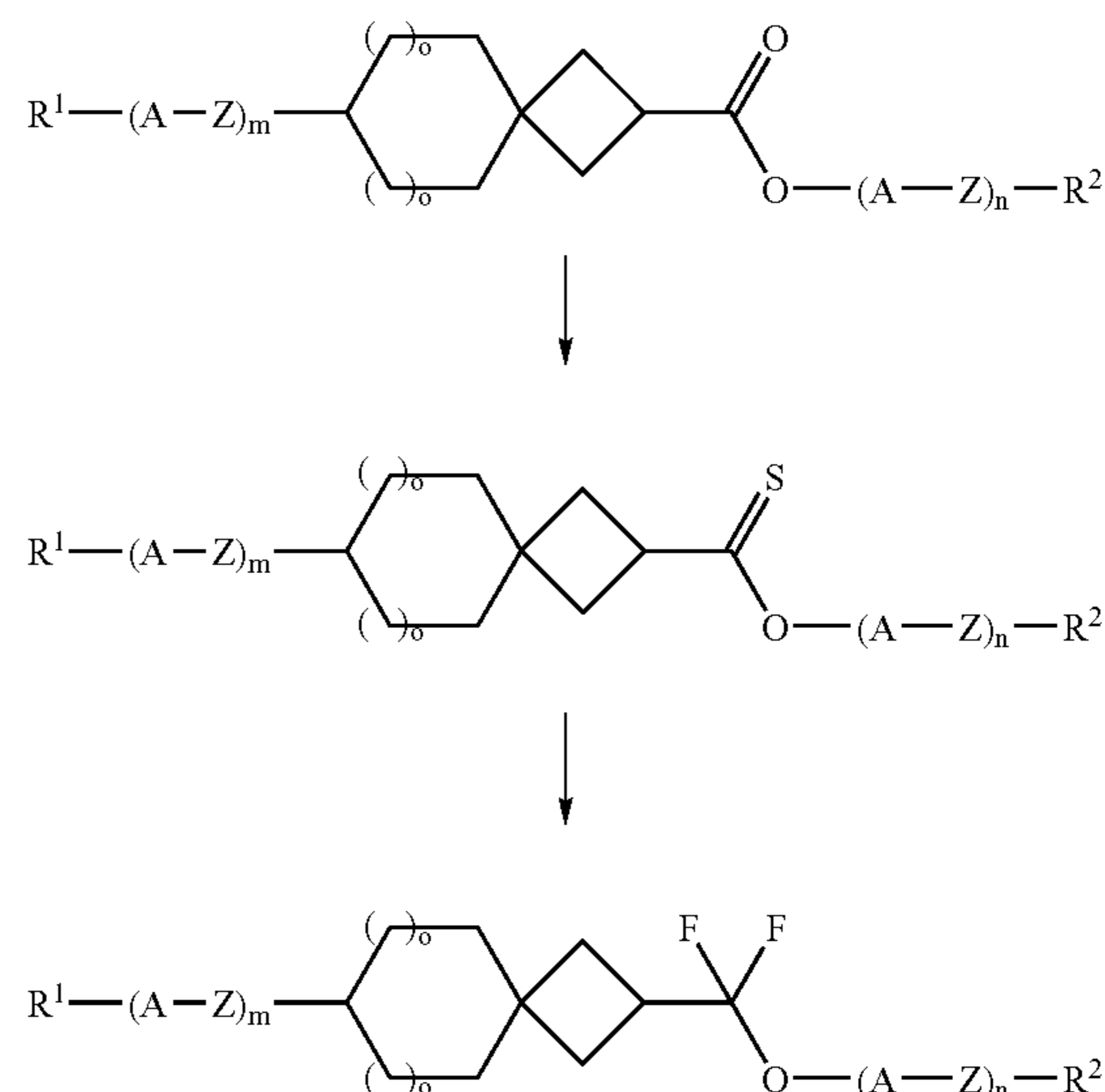
Scheme 4:
