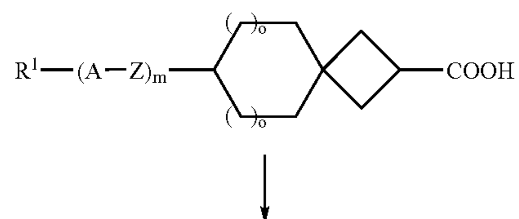
Scheme 2:
