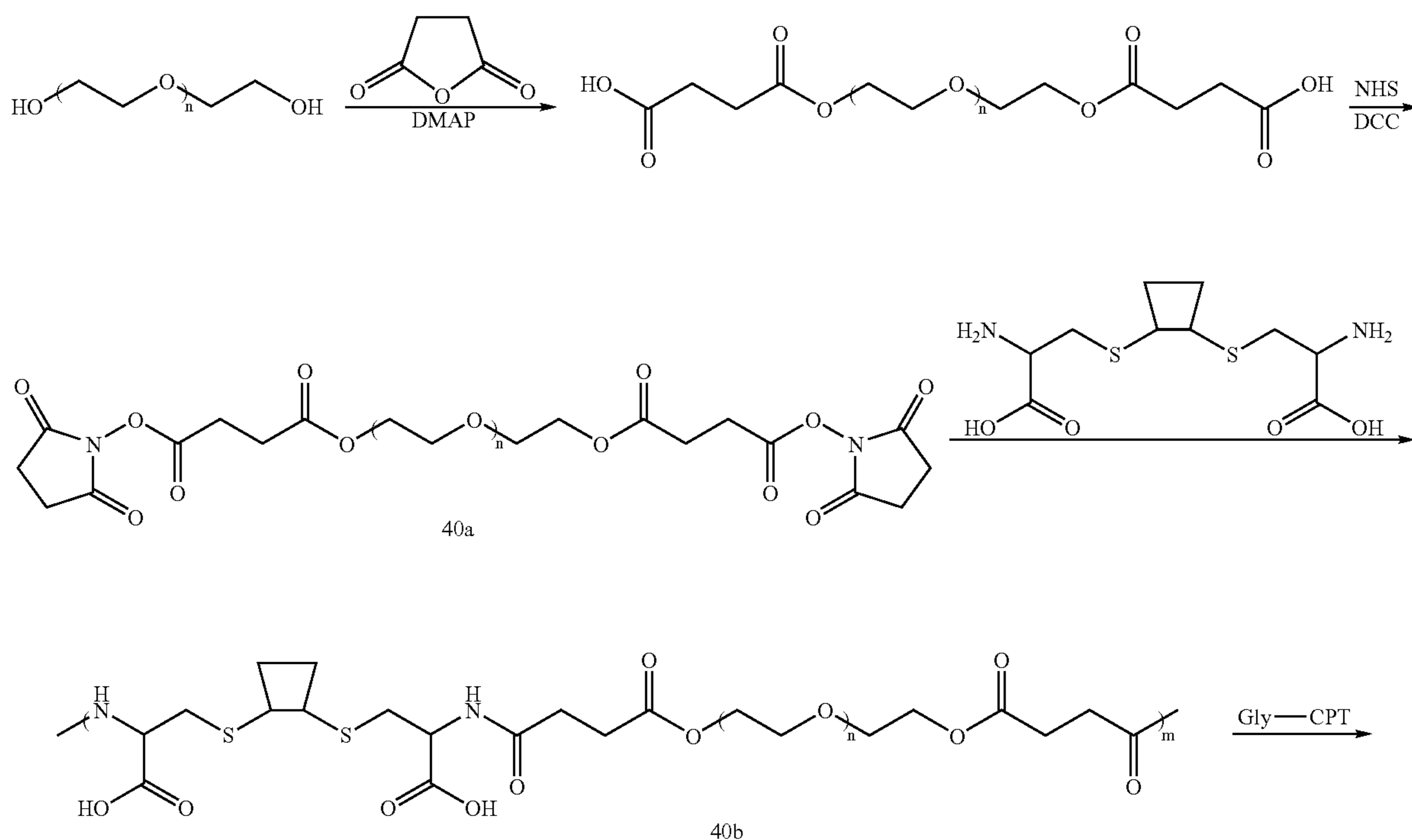
Scheme XXXXI
