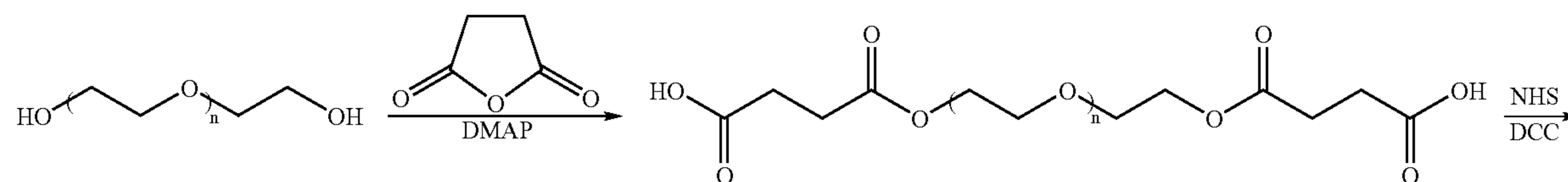
Scheme XIV
