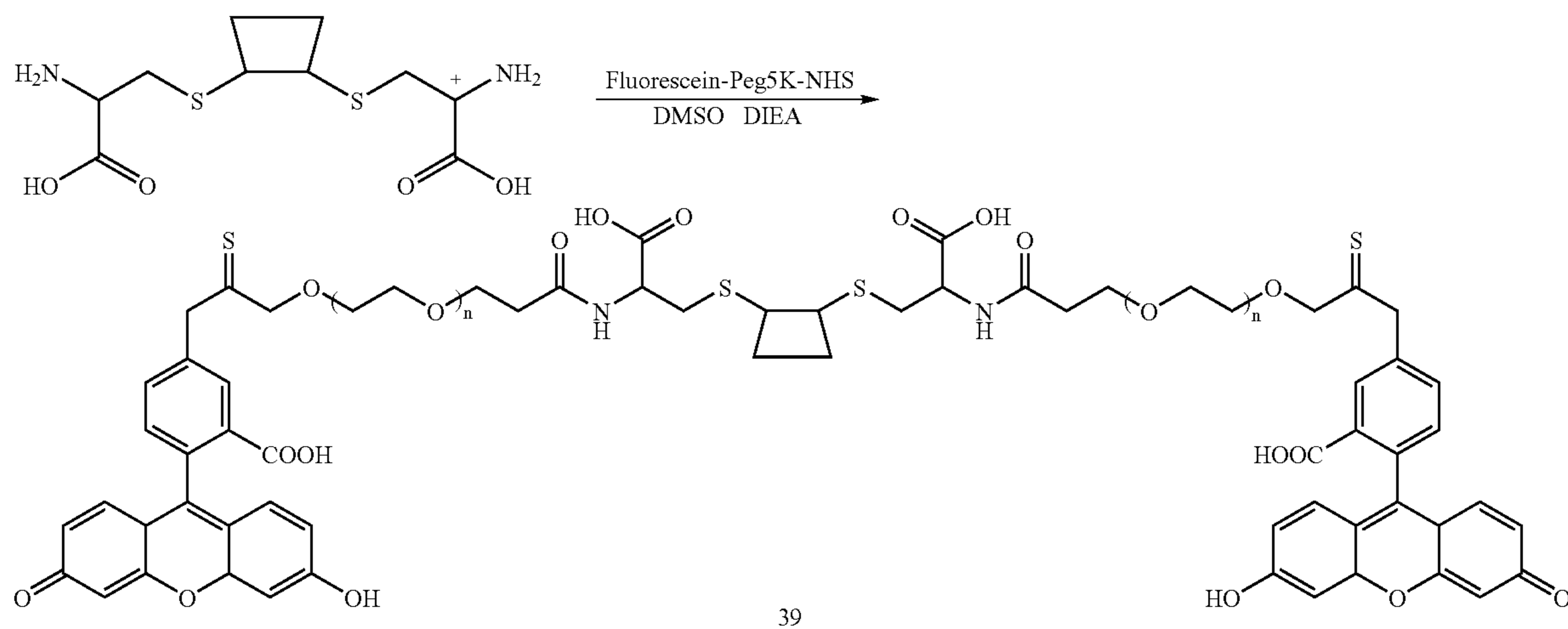
Scheme XXXX
