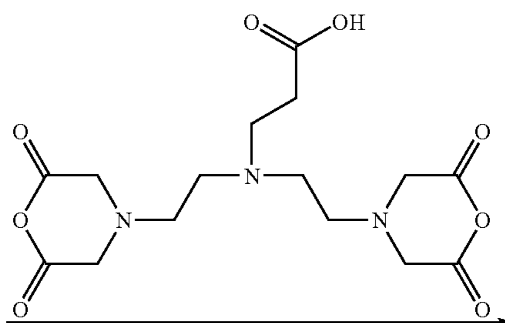
Scheme XXIX
