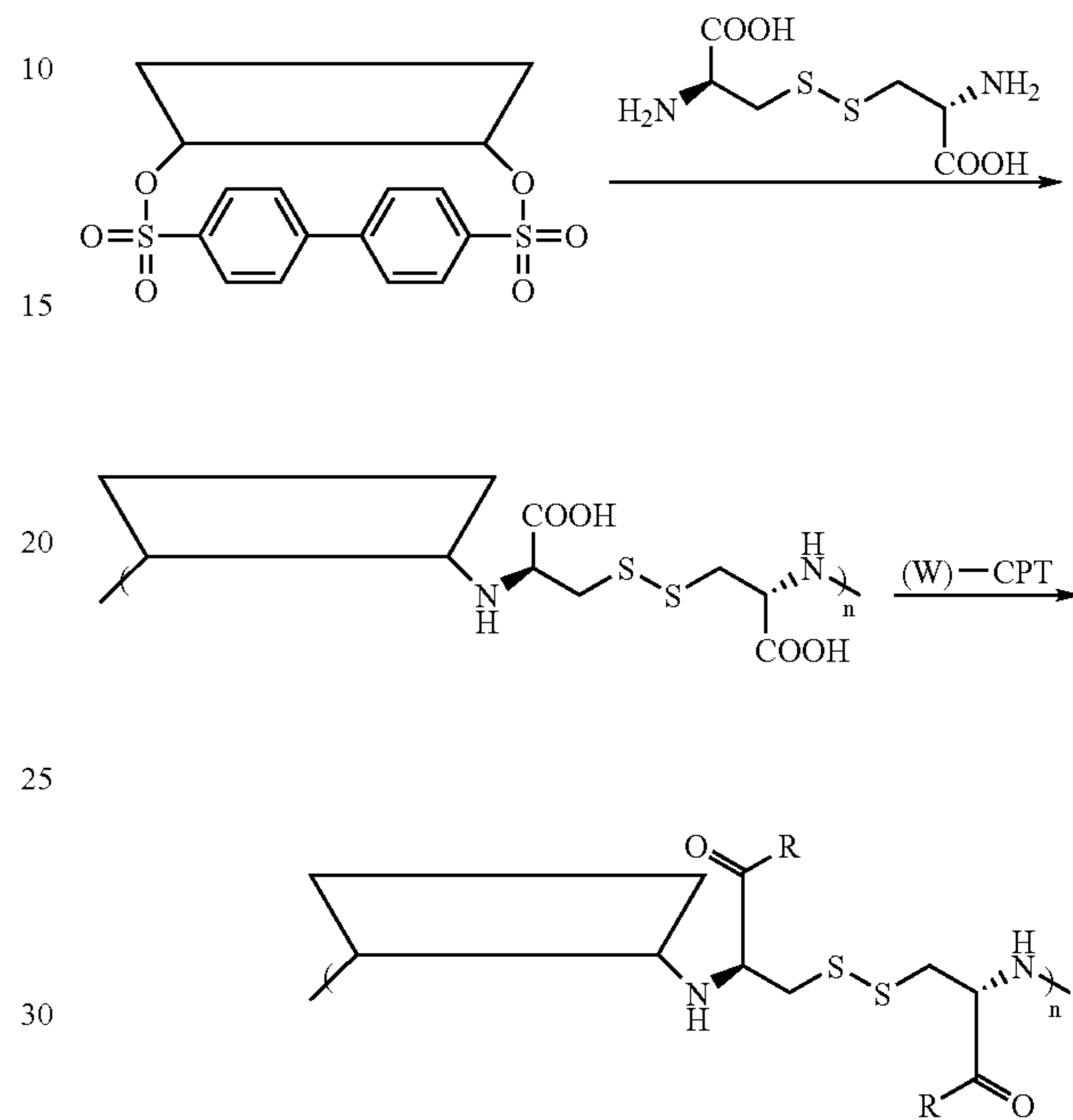
Scheme III
