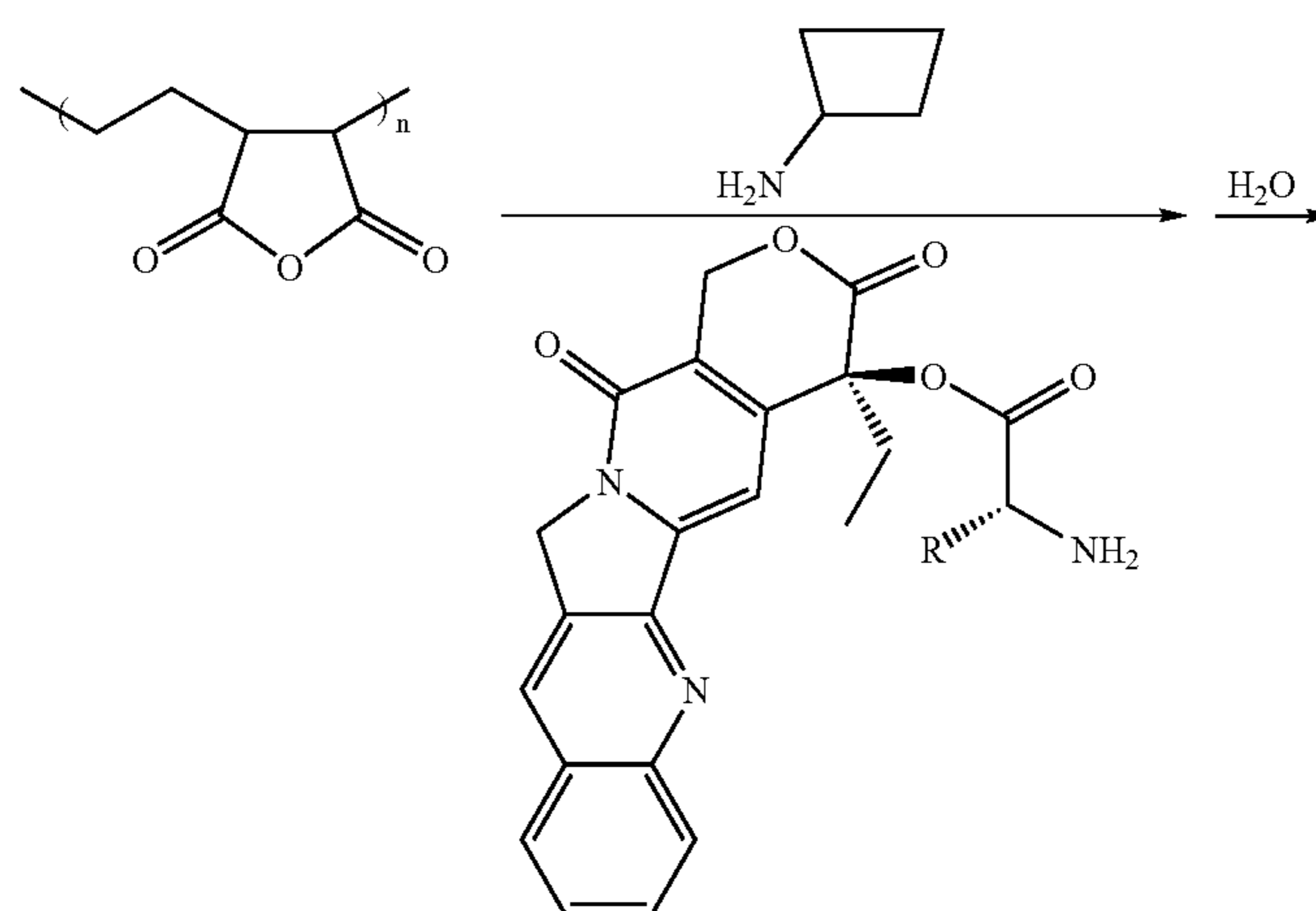
Scheme XI
