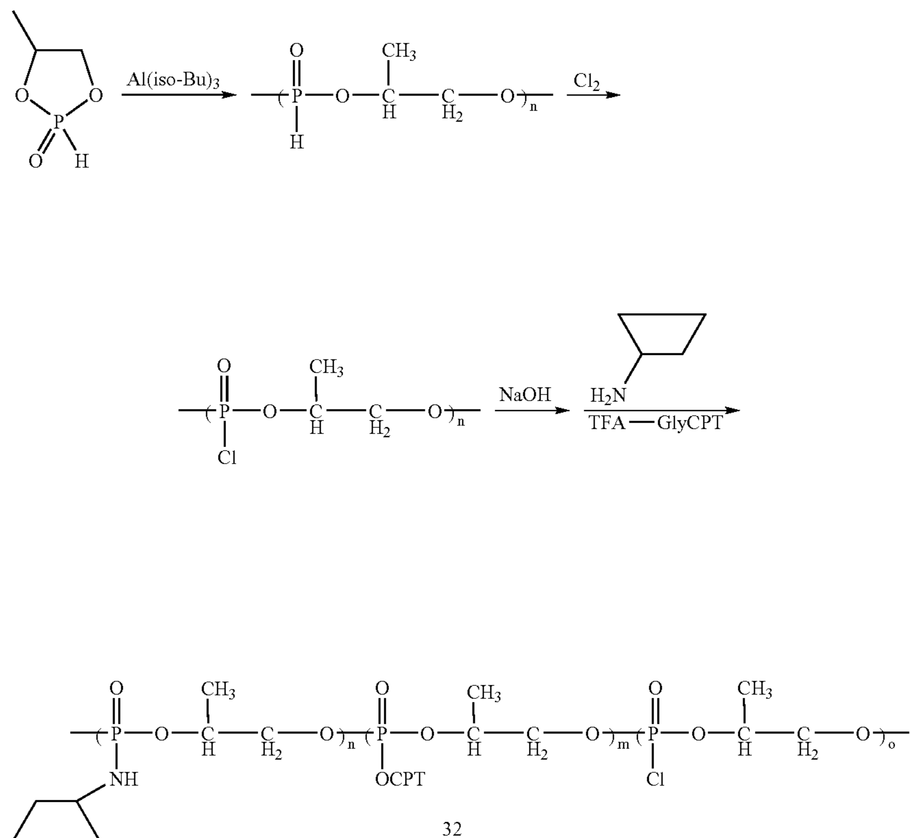
Scheme XXXIV
