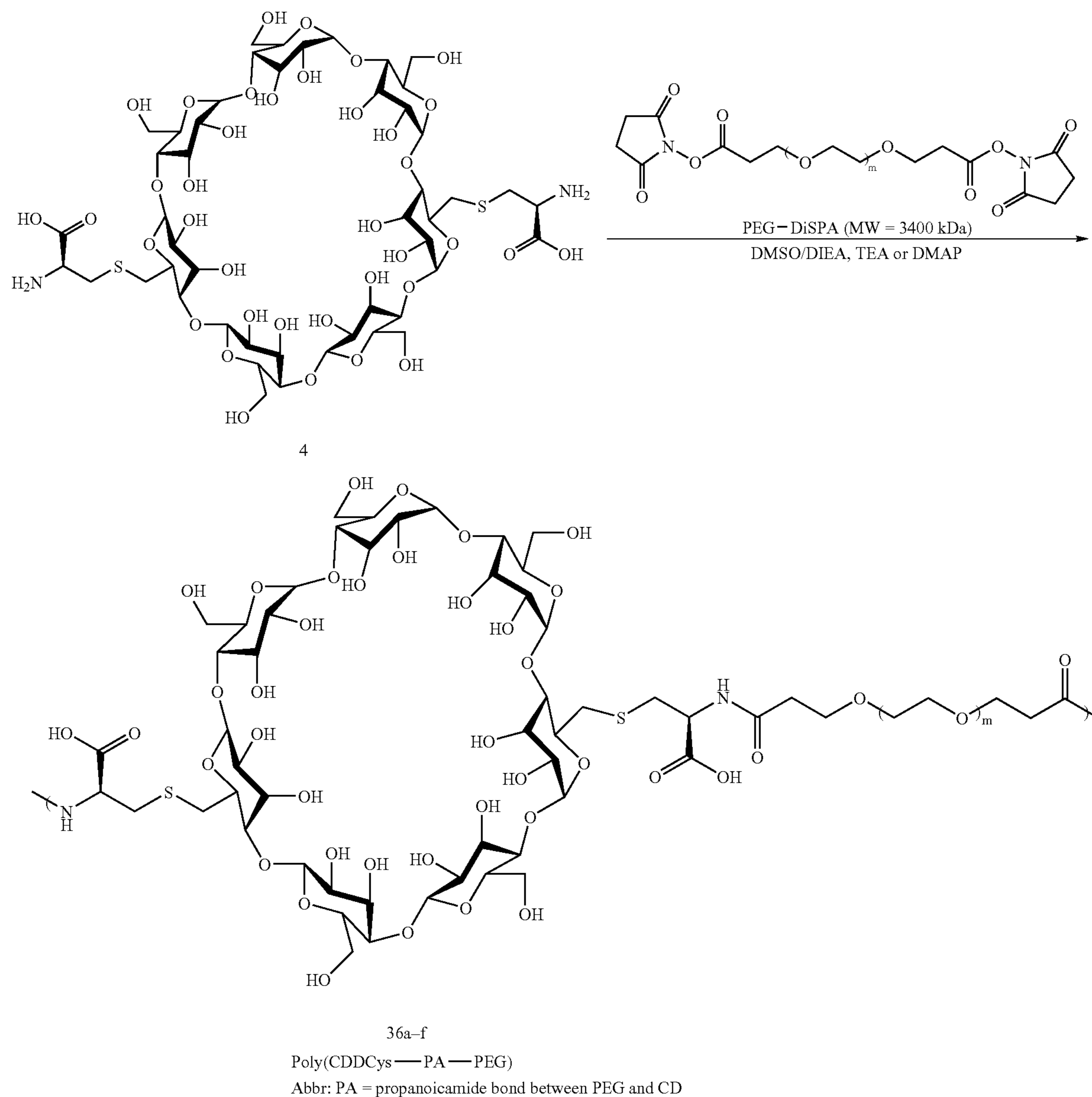
Scheme XXXVIIIa
