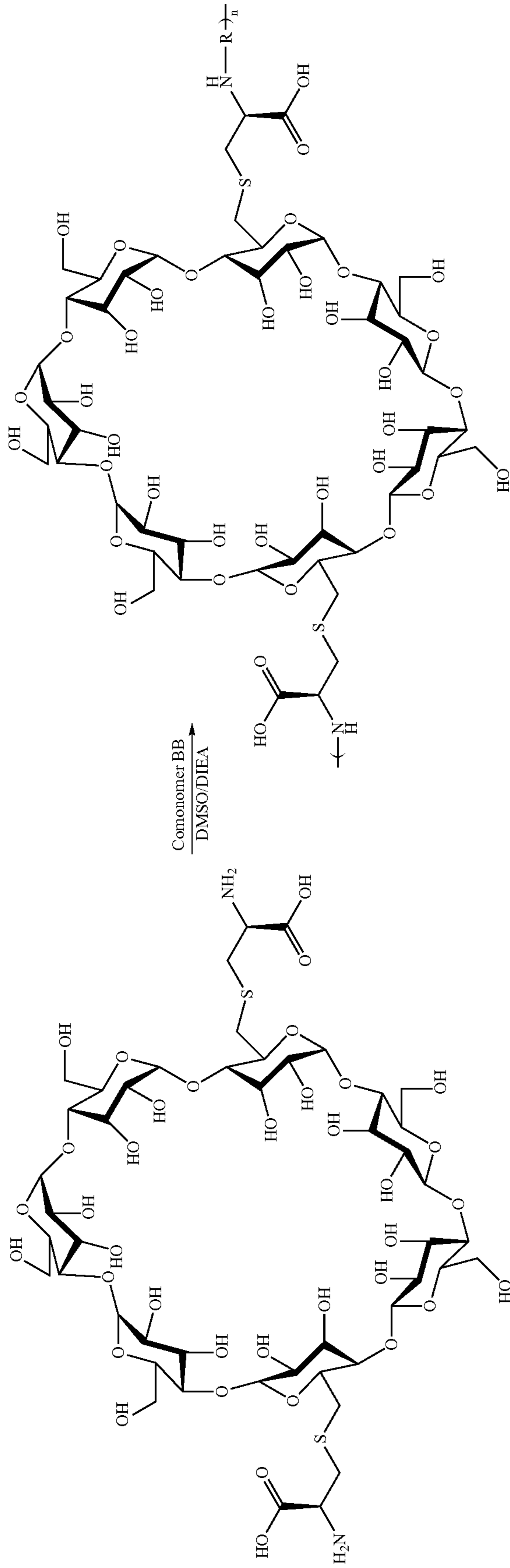
Scheme XXXVIIIb
