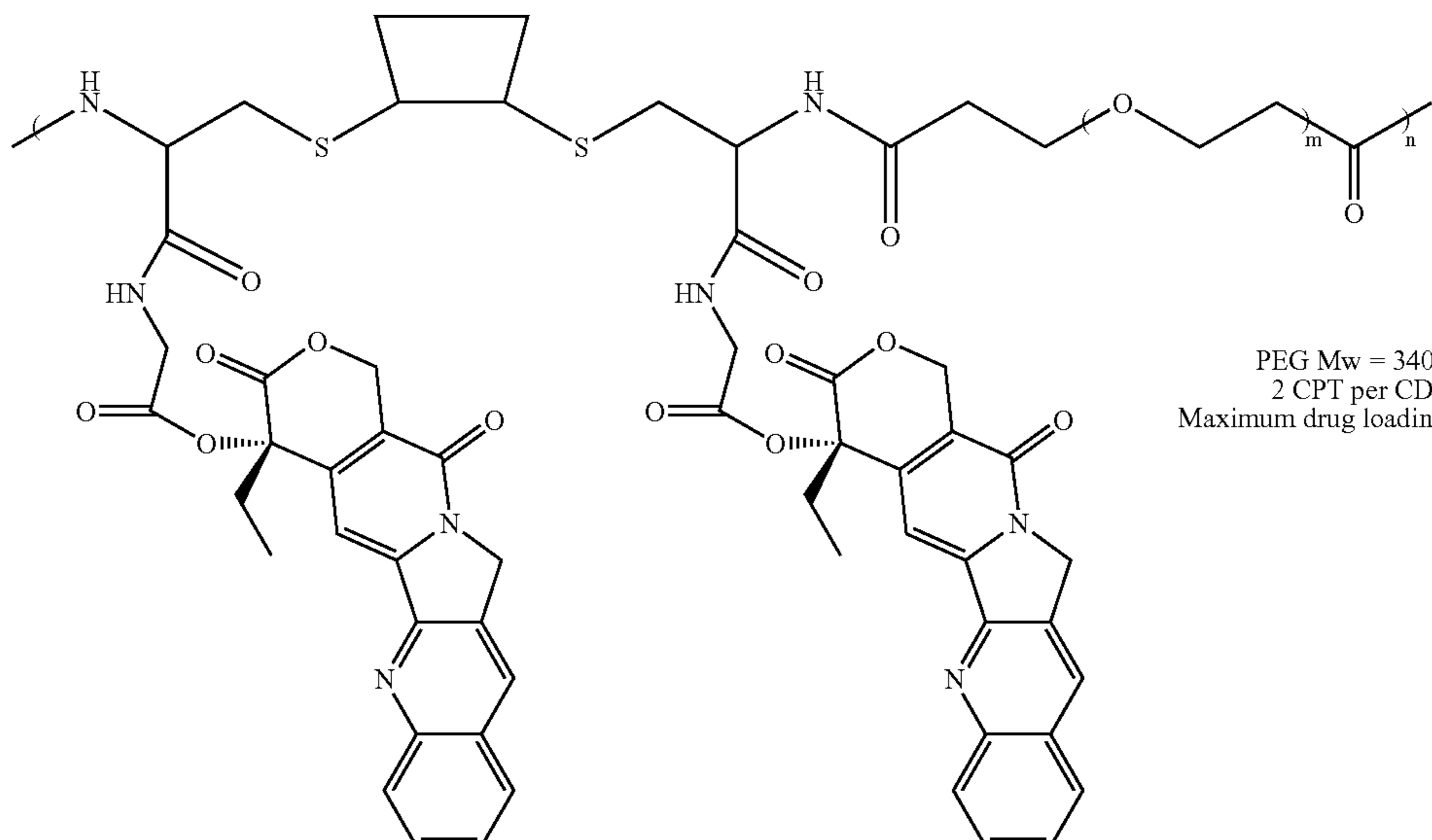
Scheme XXXXIII
