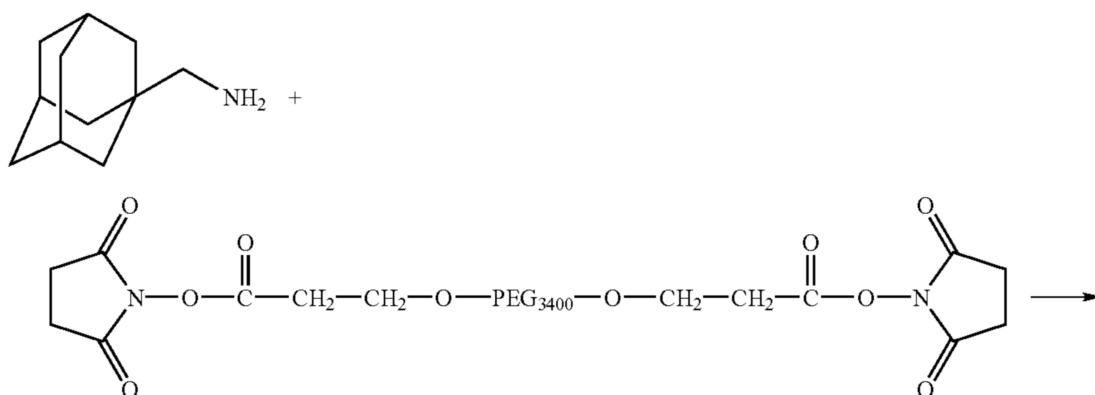
Scheme XXXXVI
