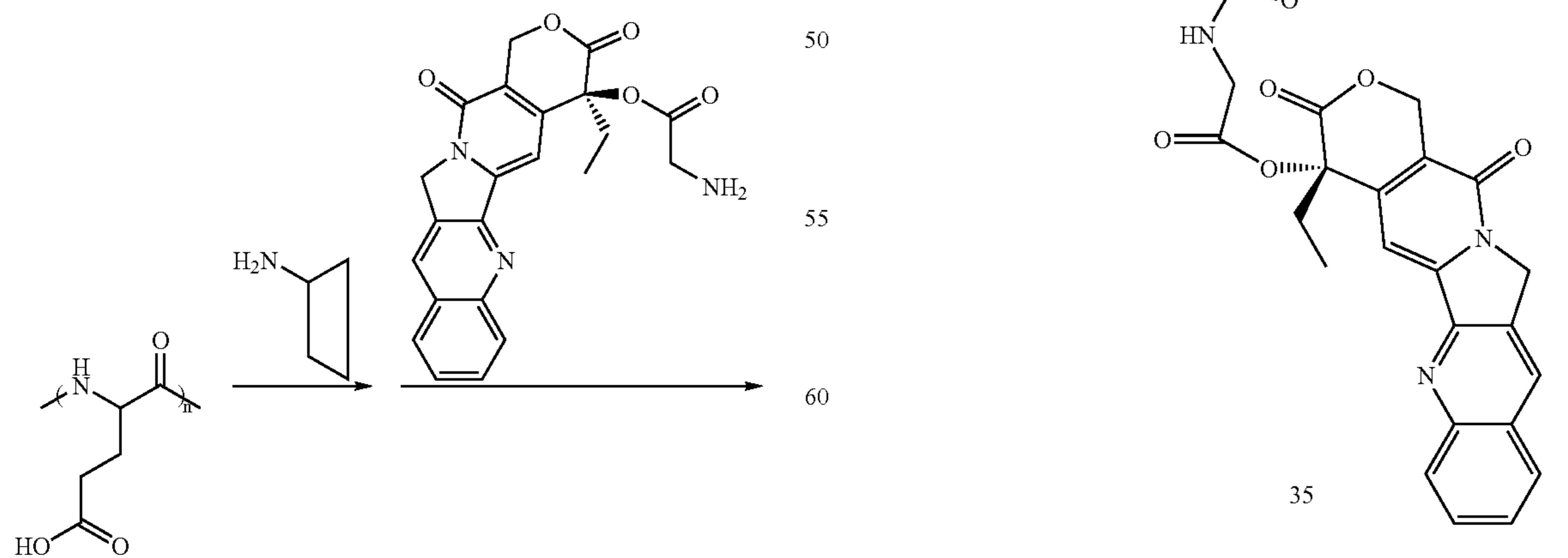
Scheme XXXVII
