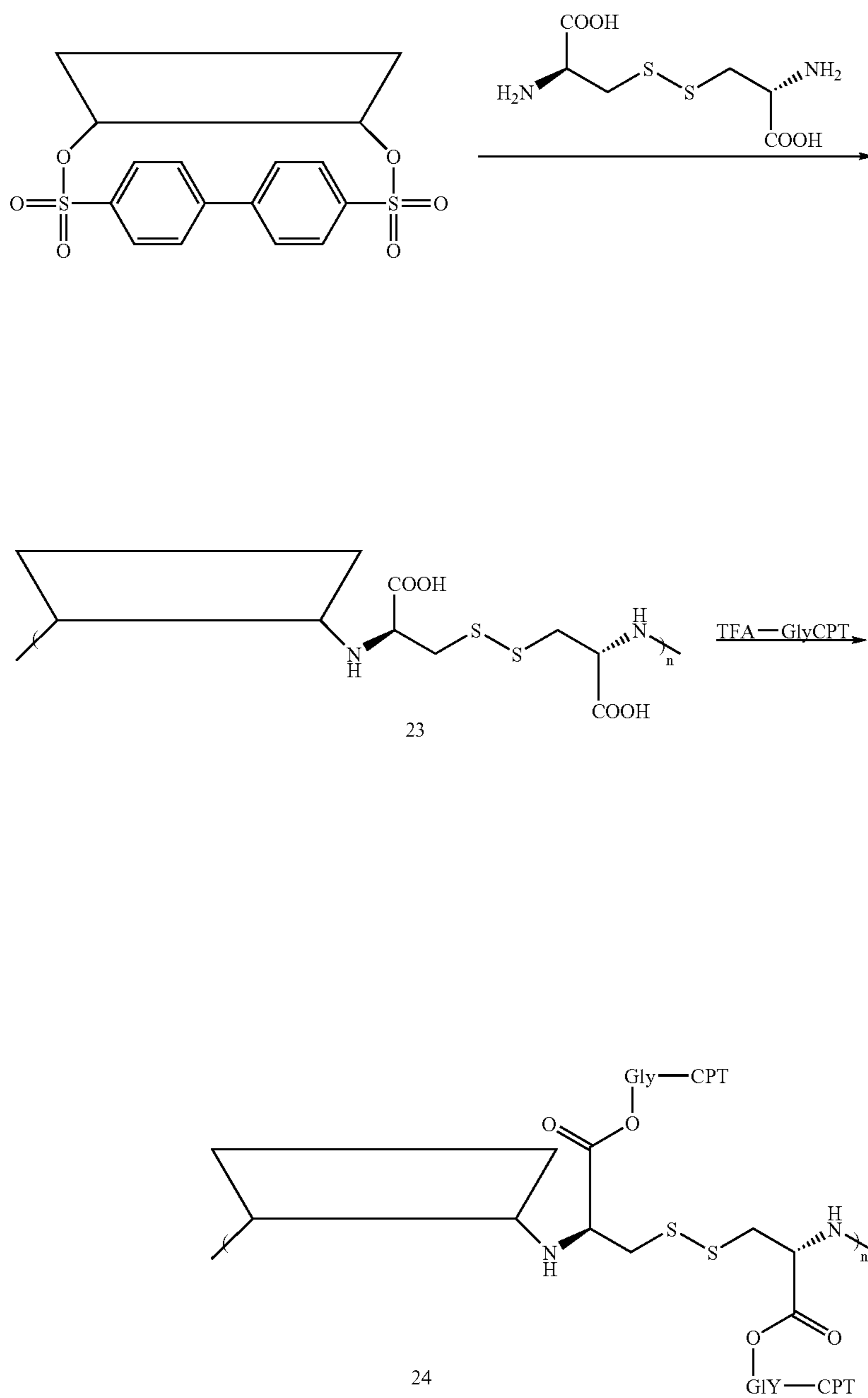
Scheme XXX
