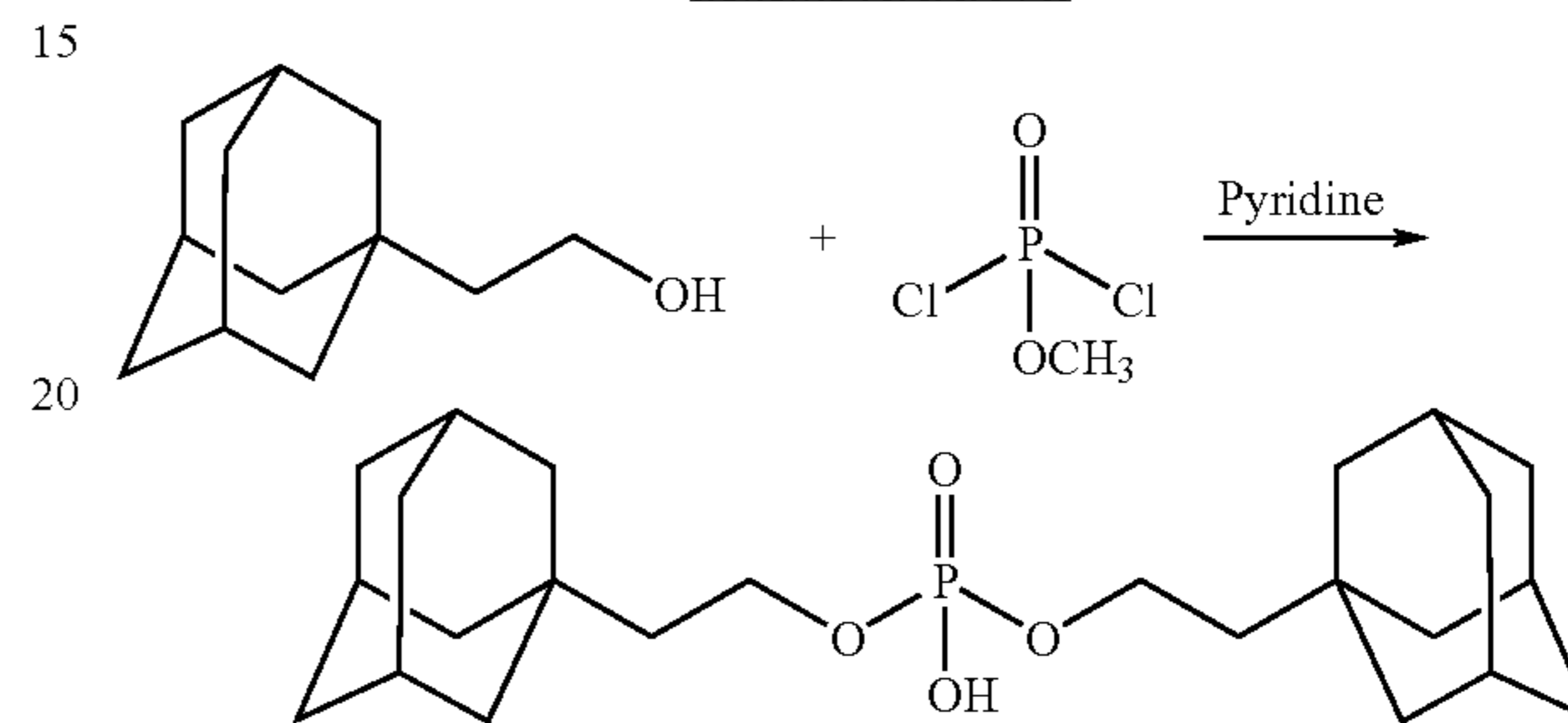
Scheme XXXXVII
