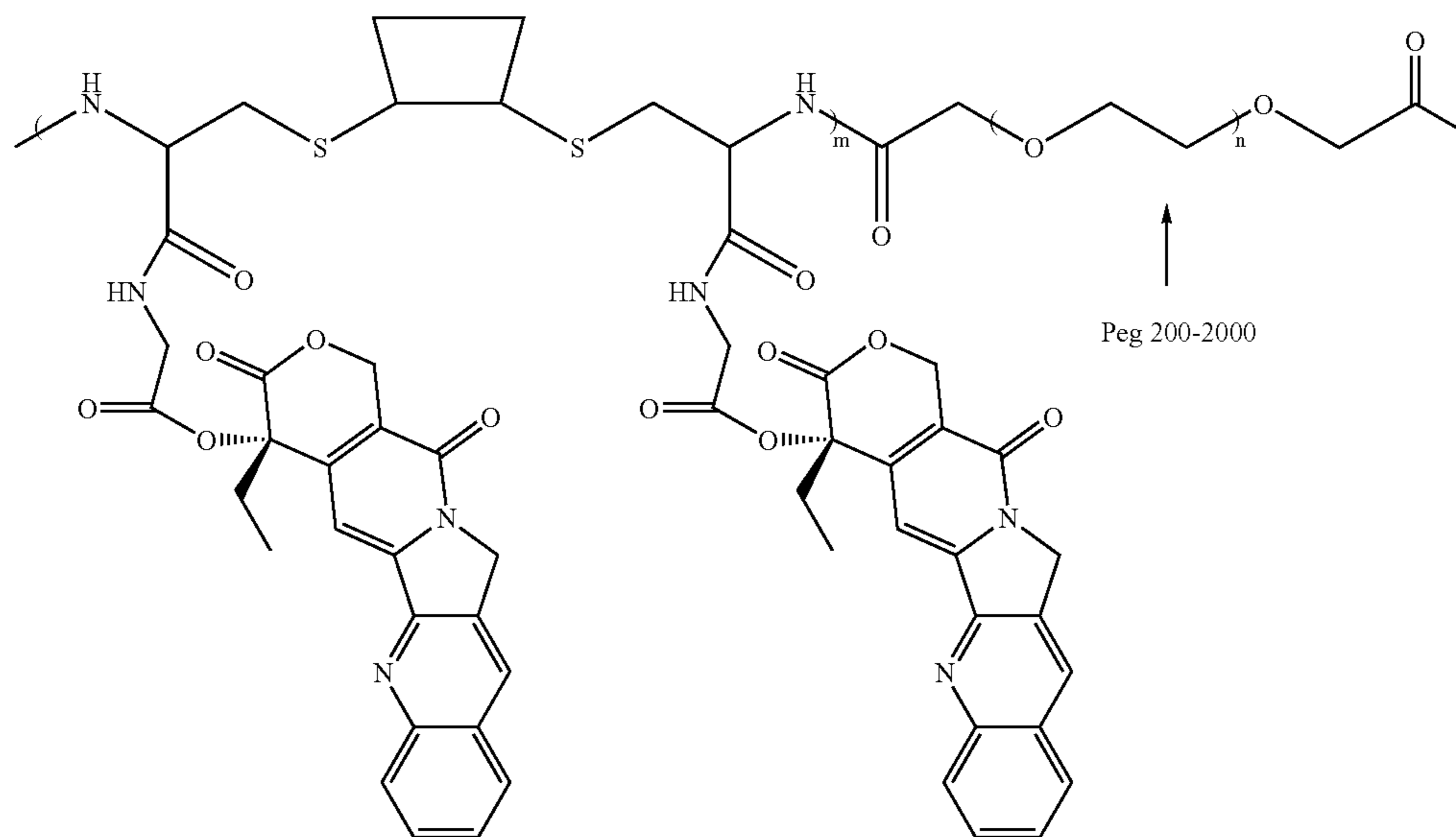
Scheme XXXXII
