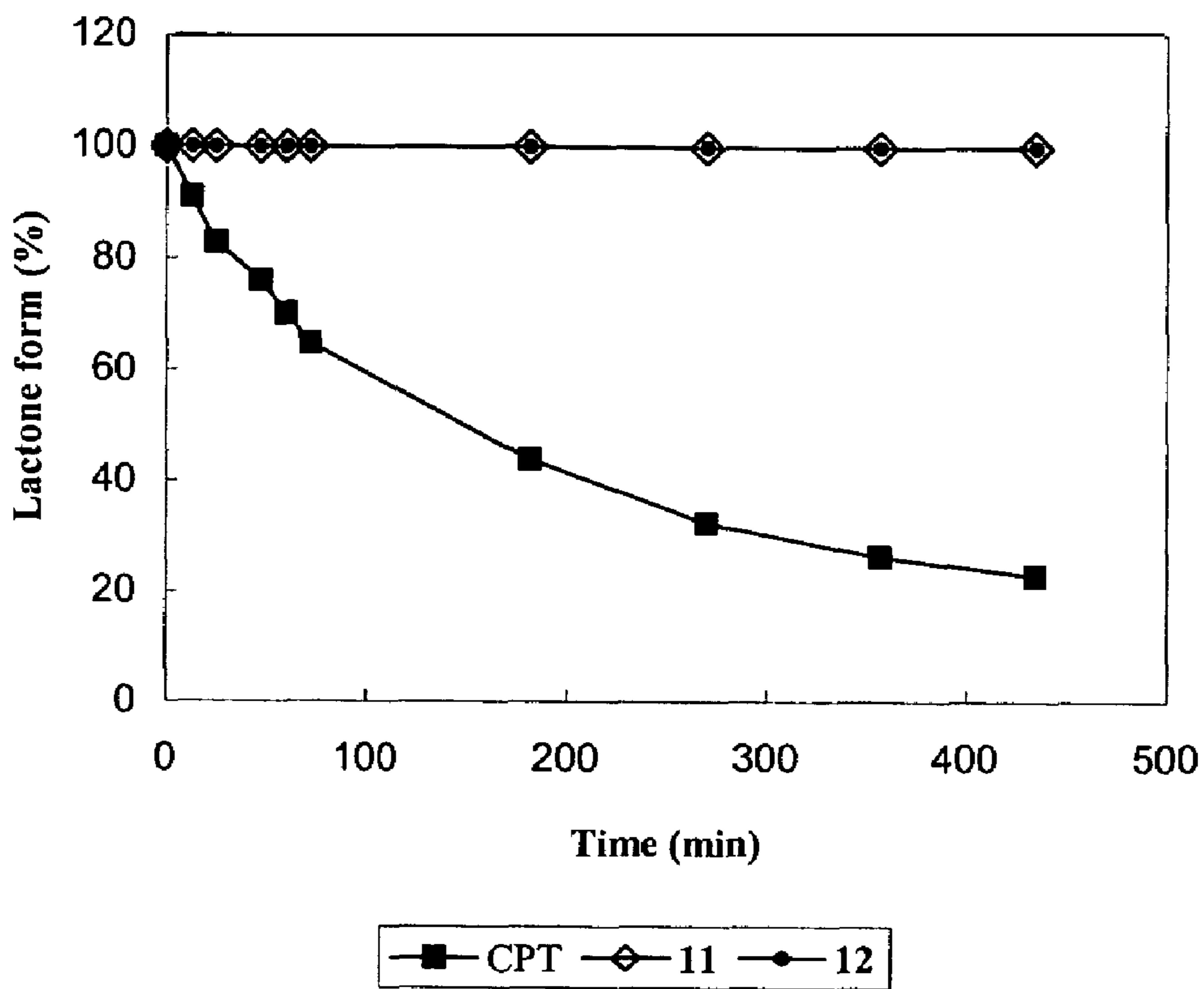
Figure 3 Lactone Ring Stability of CPT, 11 and 12 in PBS (pH 7.4)
