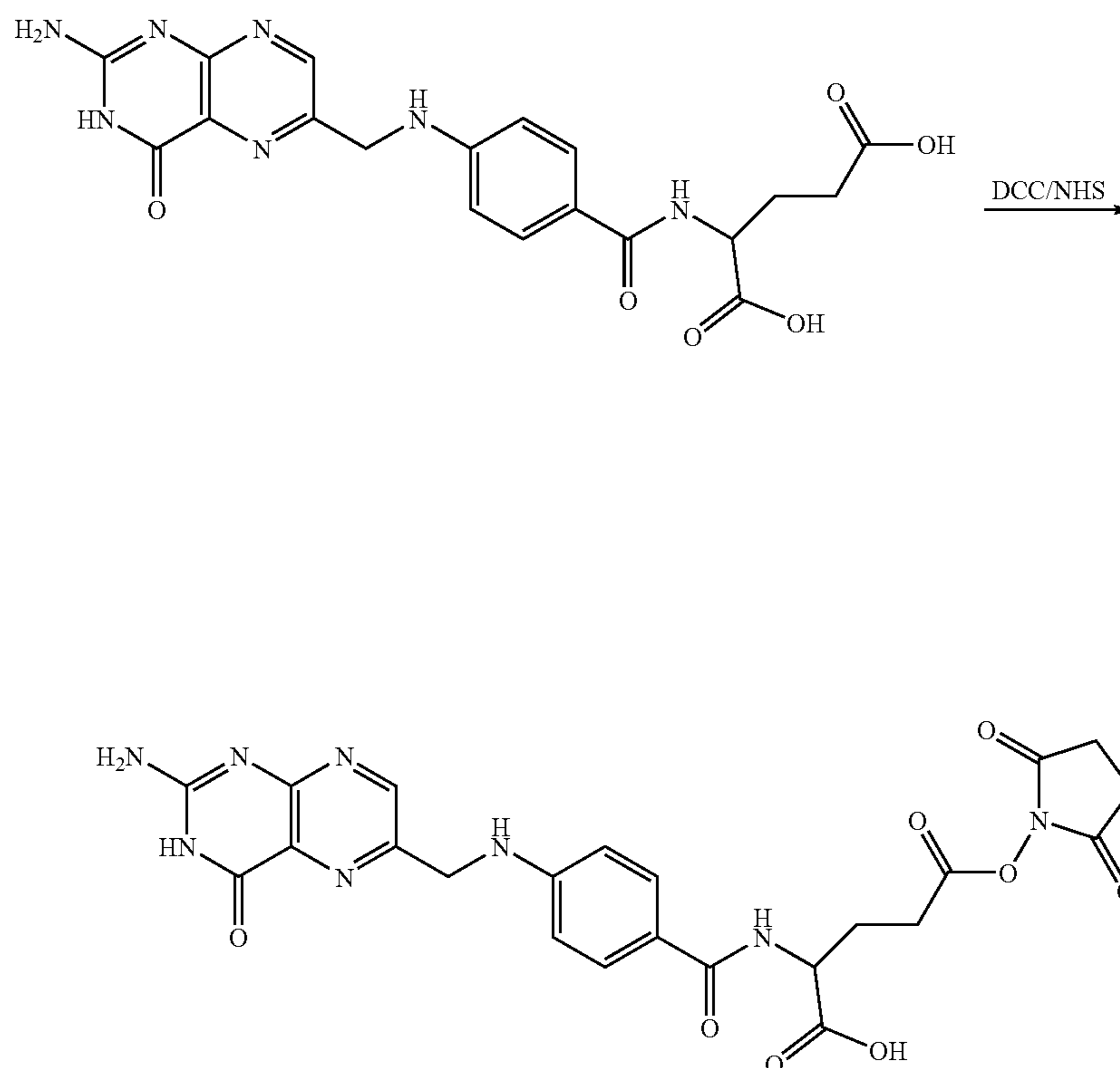
Scheme XXXXIX
