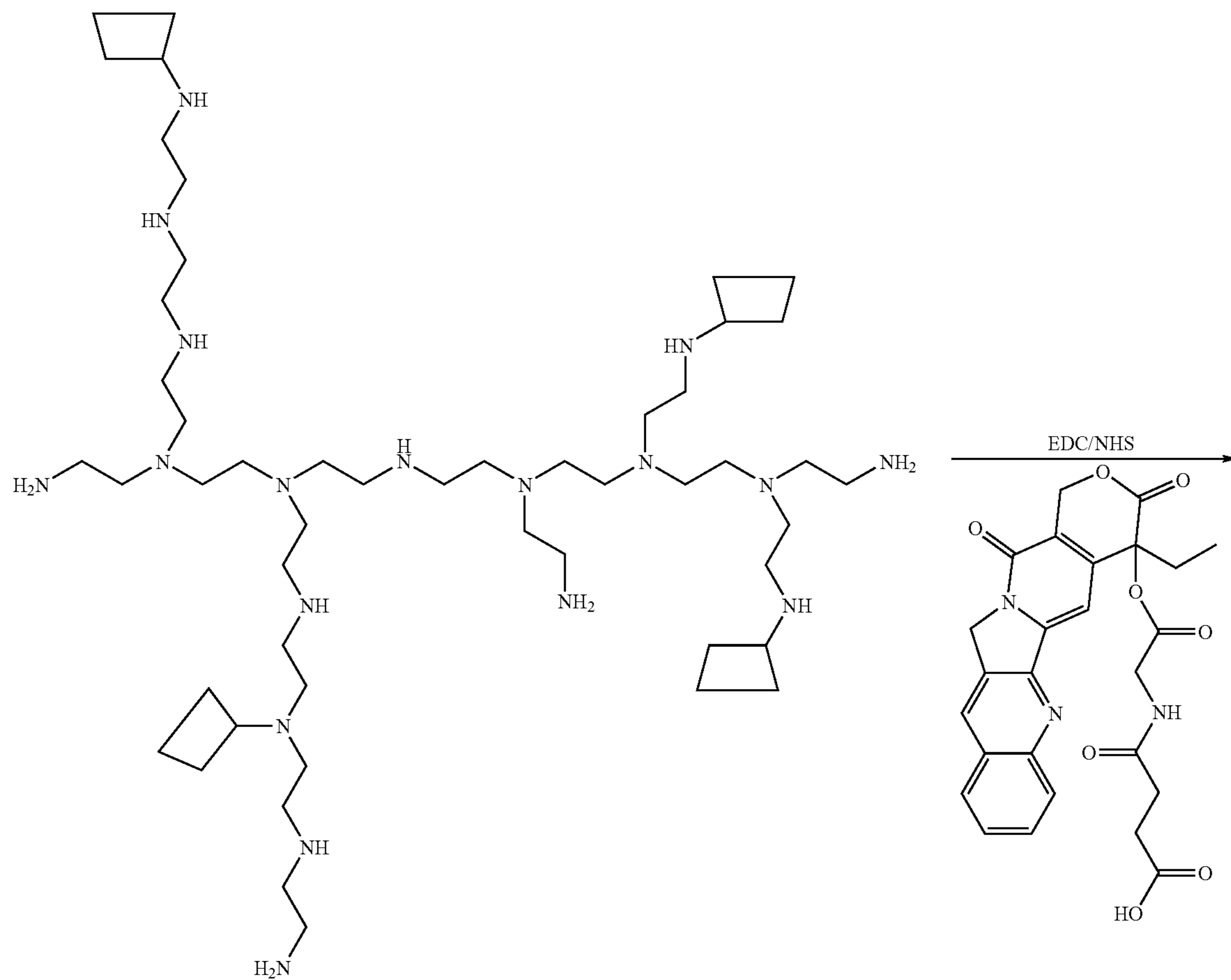
Scheme XXXXV
