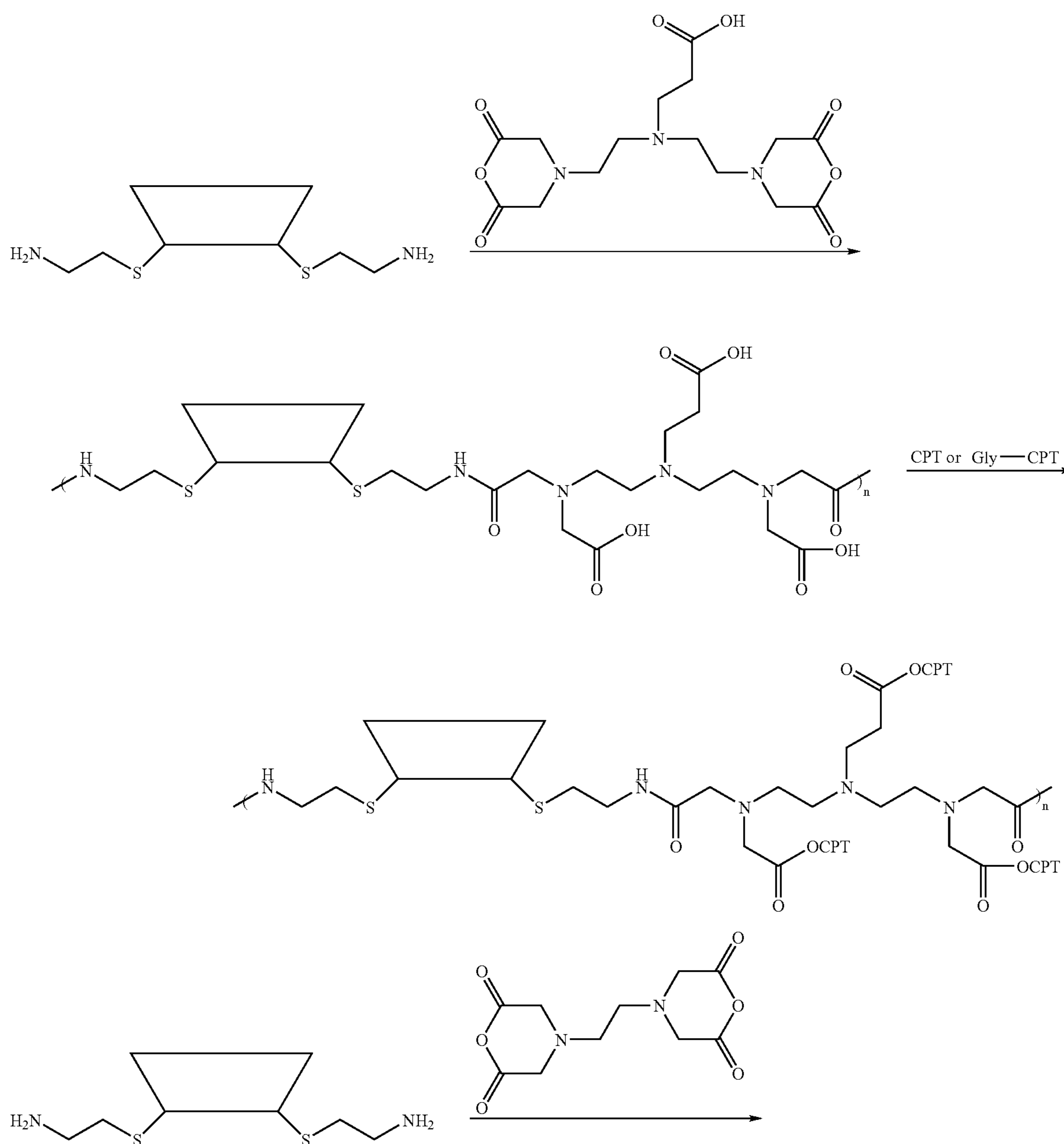
Scheme V
