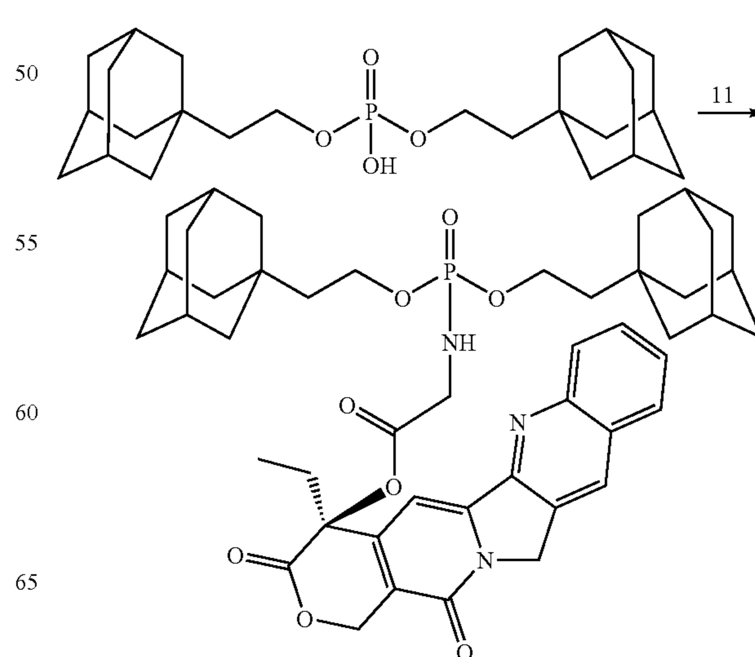
Scheme XXXXVIII
