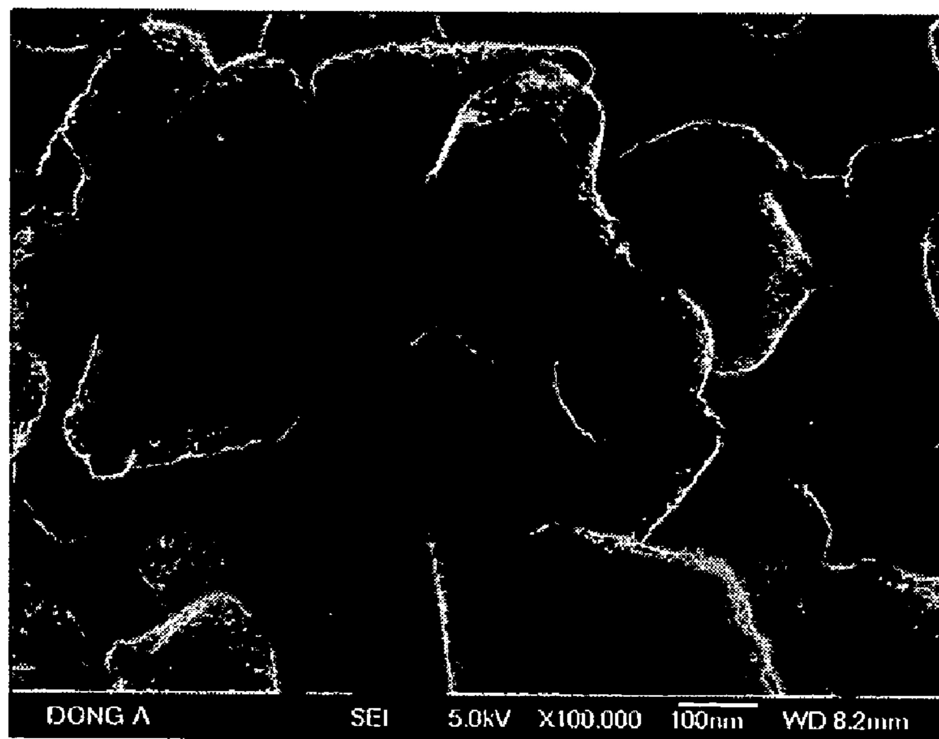
Fig. 2. Ag particles formed from the conditions mentioned in example 2.
