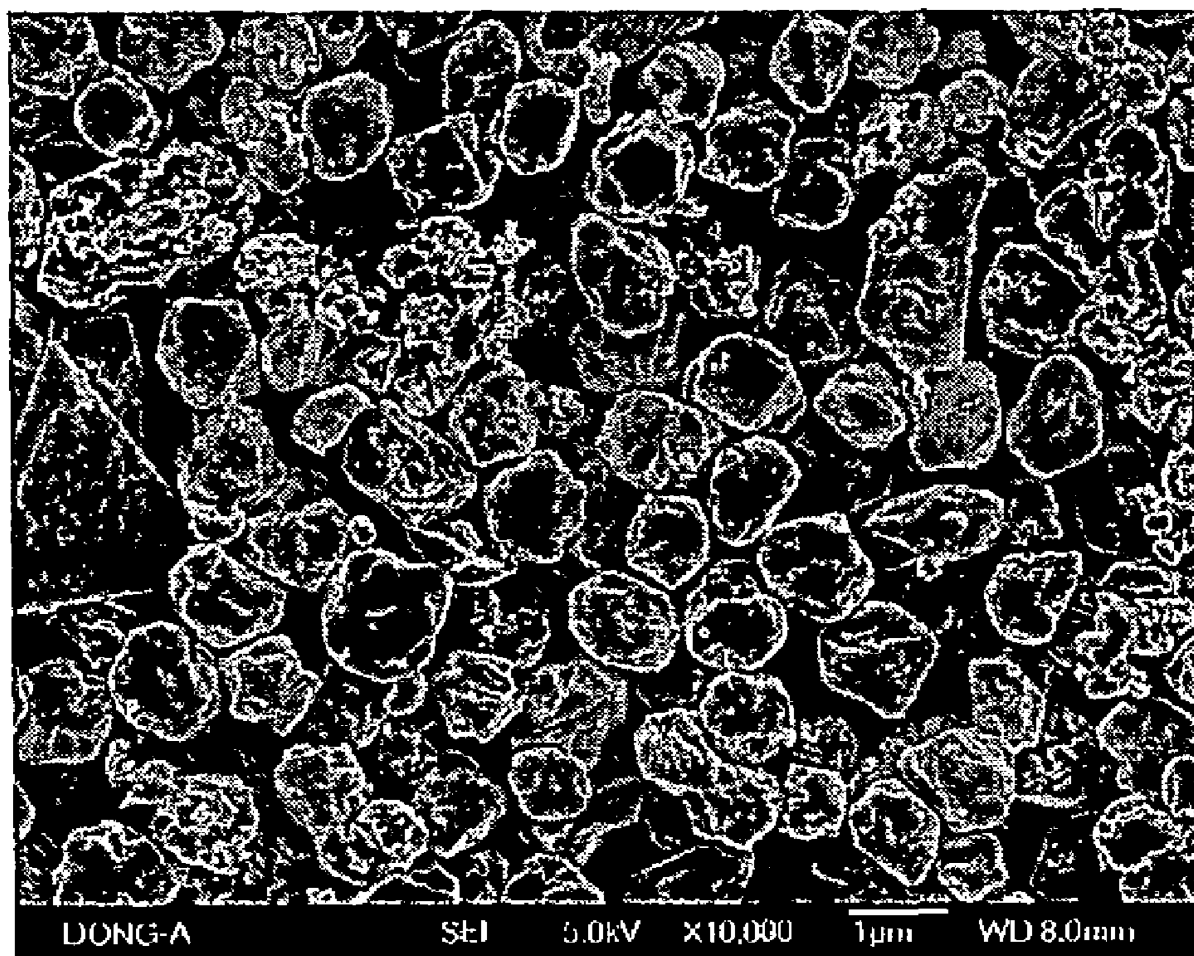
Micron-sized Ag particles formed from direct reaction between silver carbonate and hydrogen peroxide
