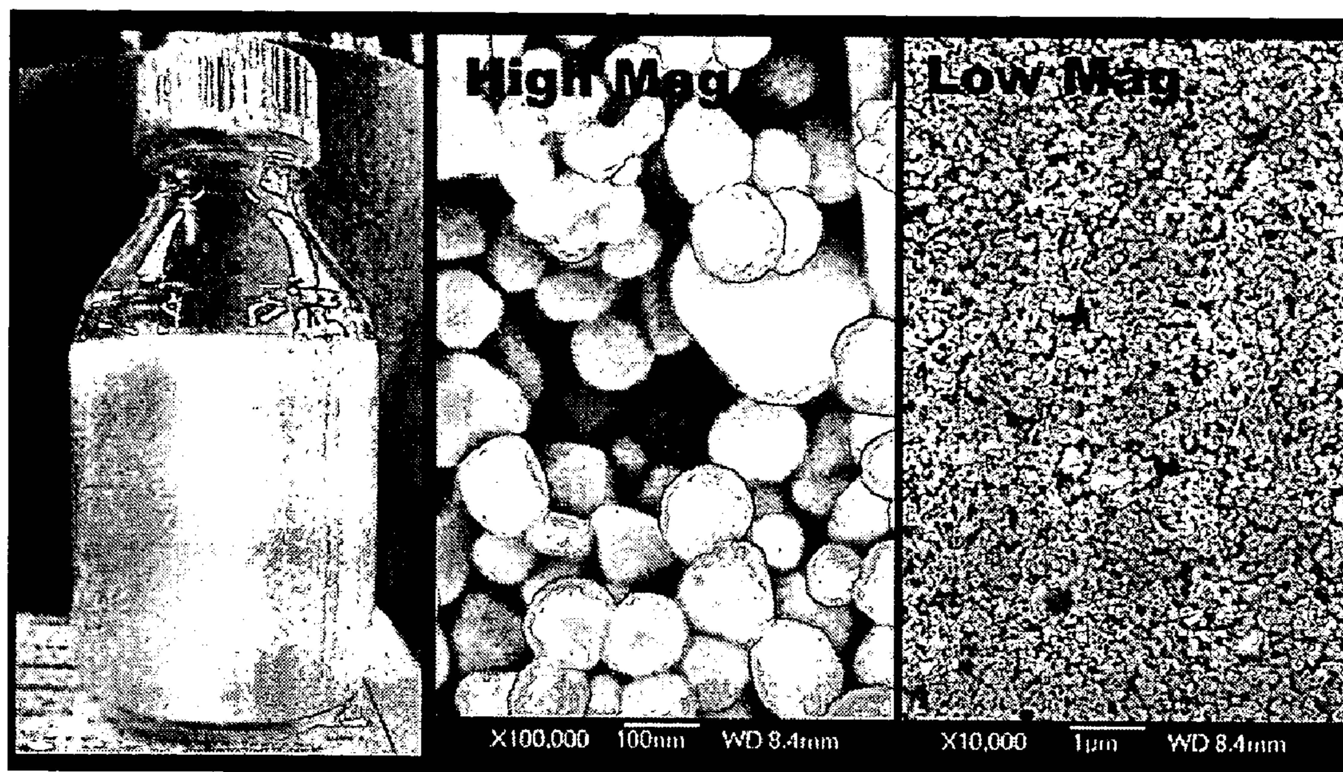
Fig. 1. Ag particles obtained by centrifuge operating to 17,000rpm for 10 min
