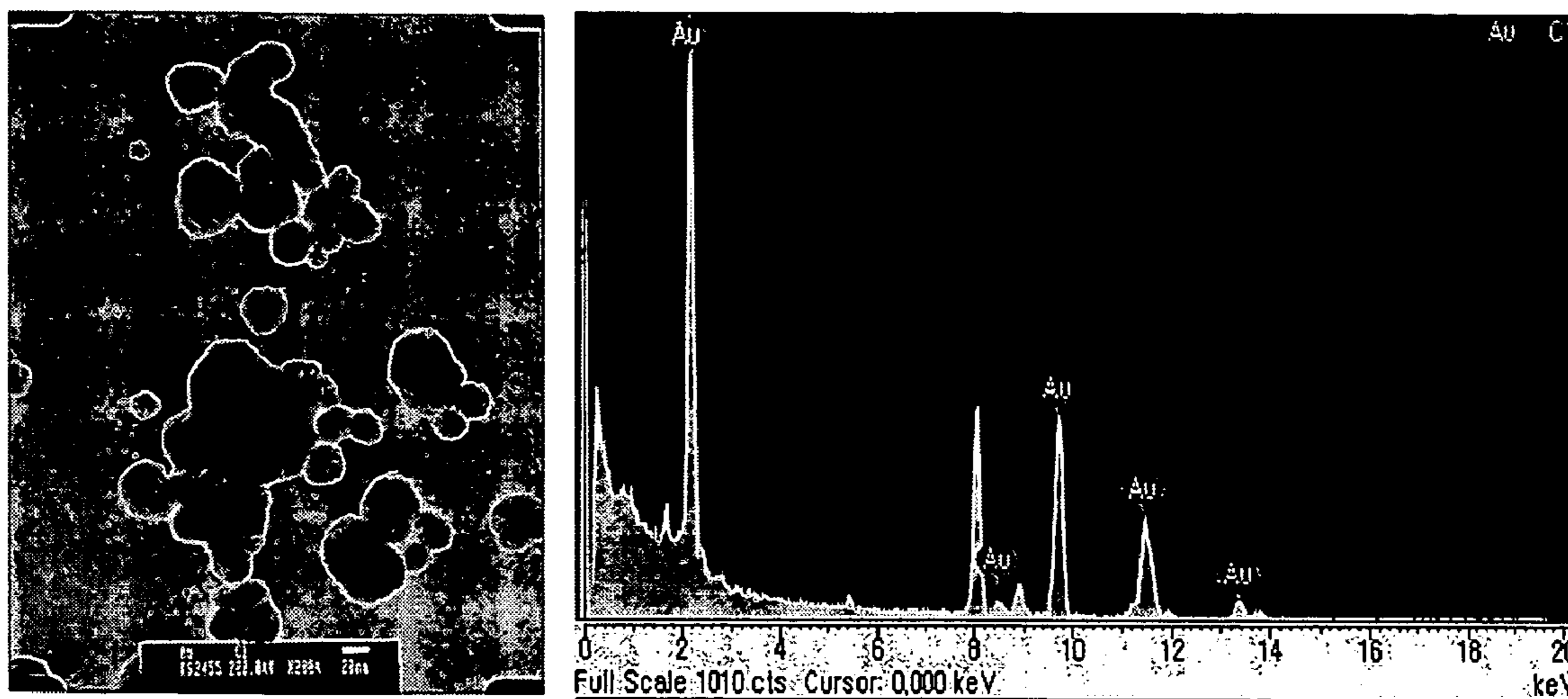
Fig. 4. Nano-sized Au particles formed from the conditions mentioned in example 4.
