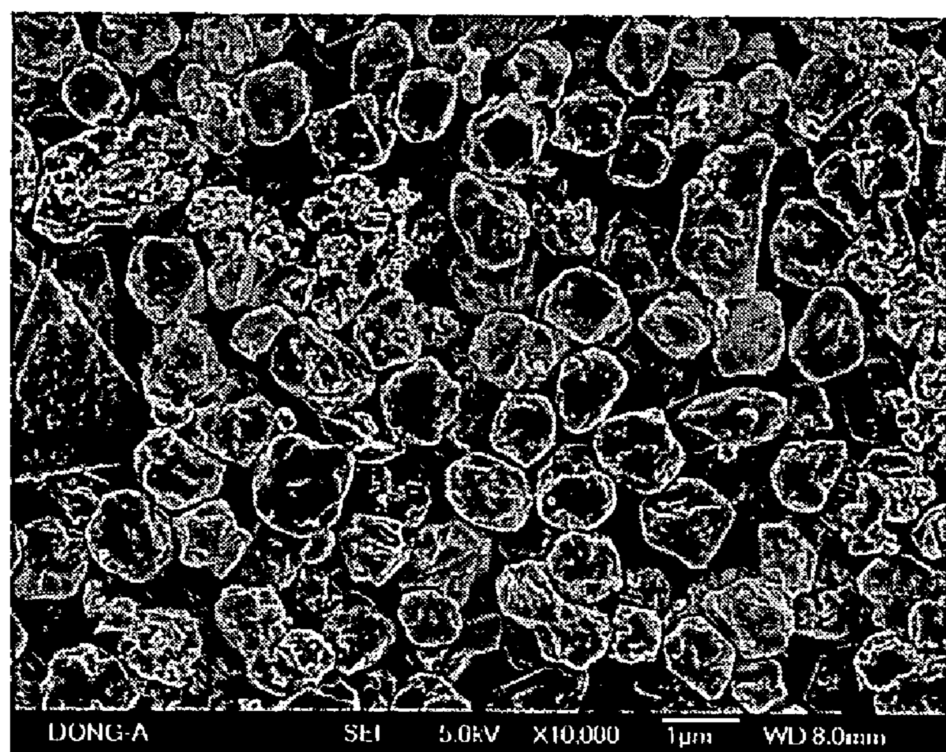
Fig. 3. Micron-sized Ag particles formed from direct reaction between silver carbonate and hydrogen peroxide
