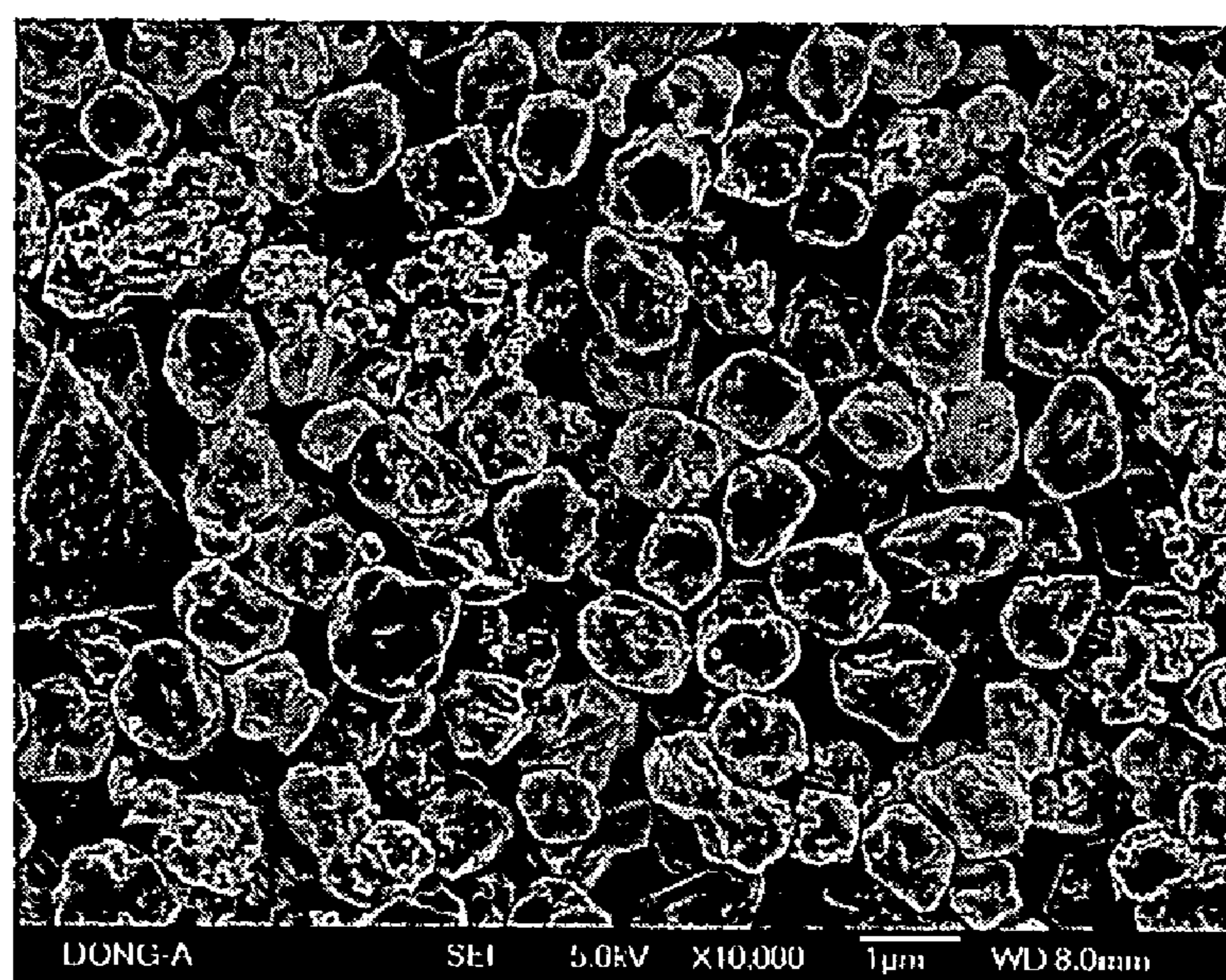
Fig. 3. Micron-sized Ag particles formed from direct reaction between silver carbonate and hydrogen peroxide
