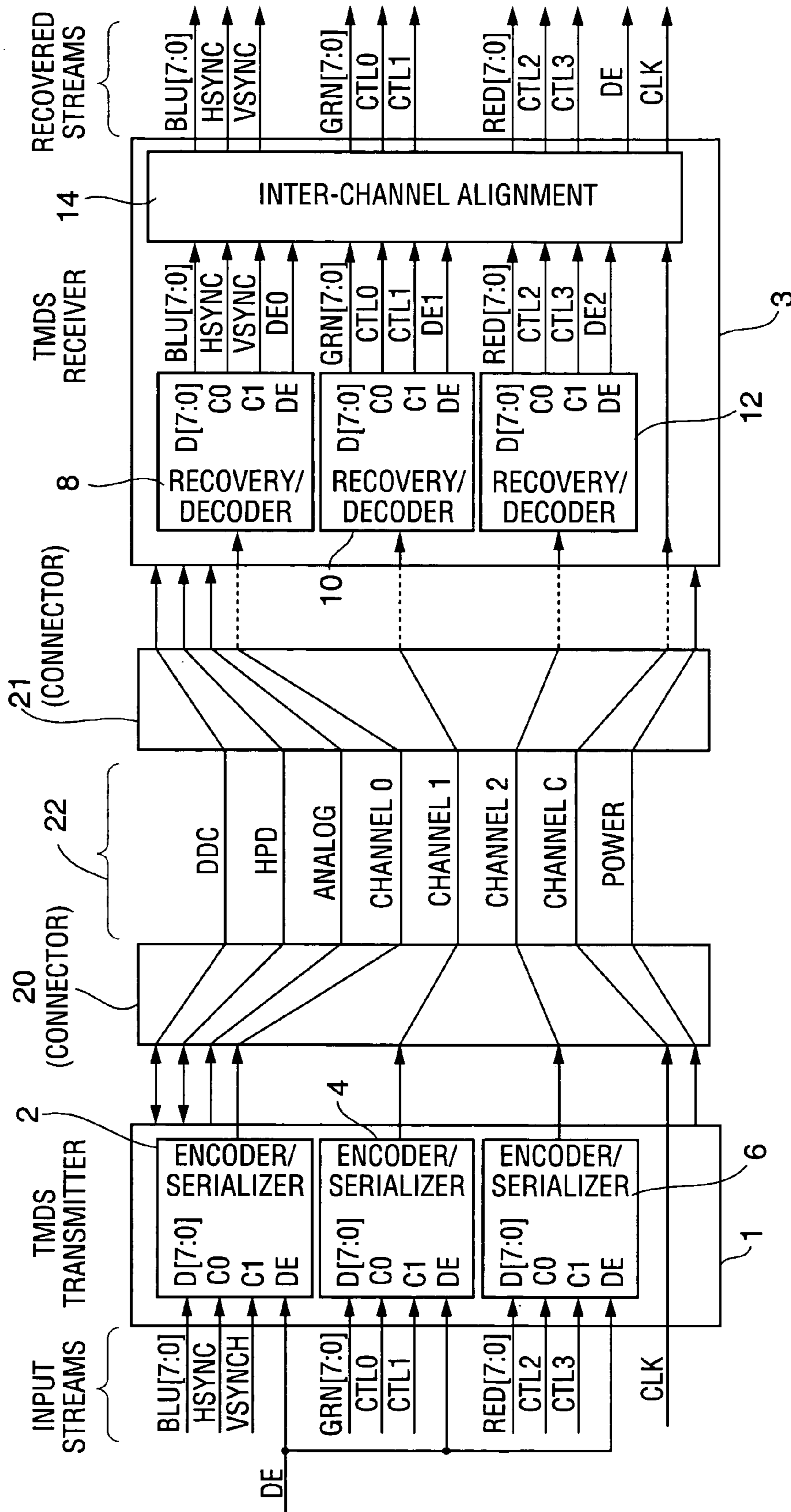
FIG. 1 (PRIOR ART)
