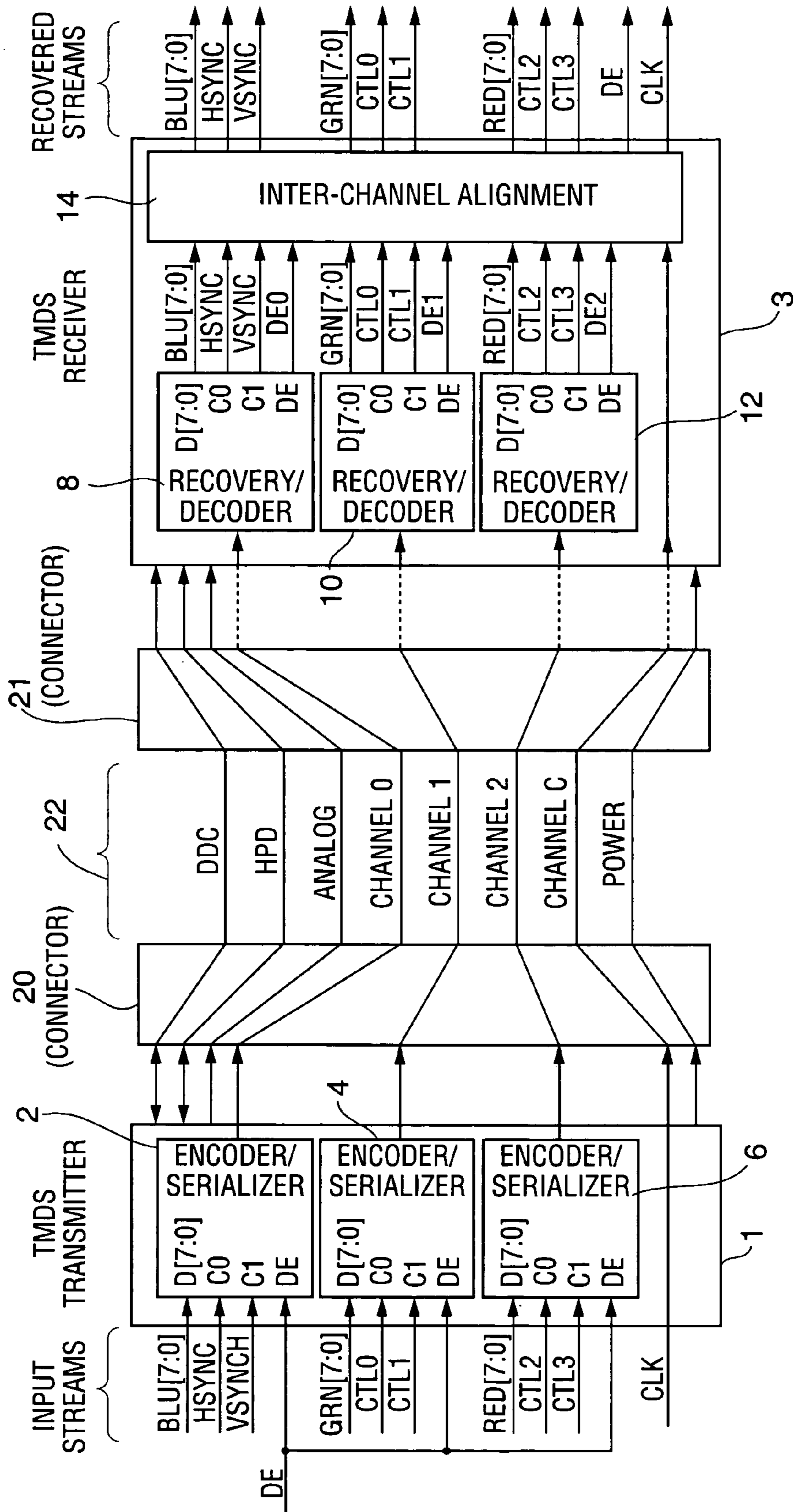
FIG. 1 (PRIOR ART)
