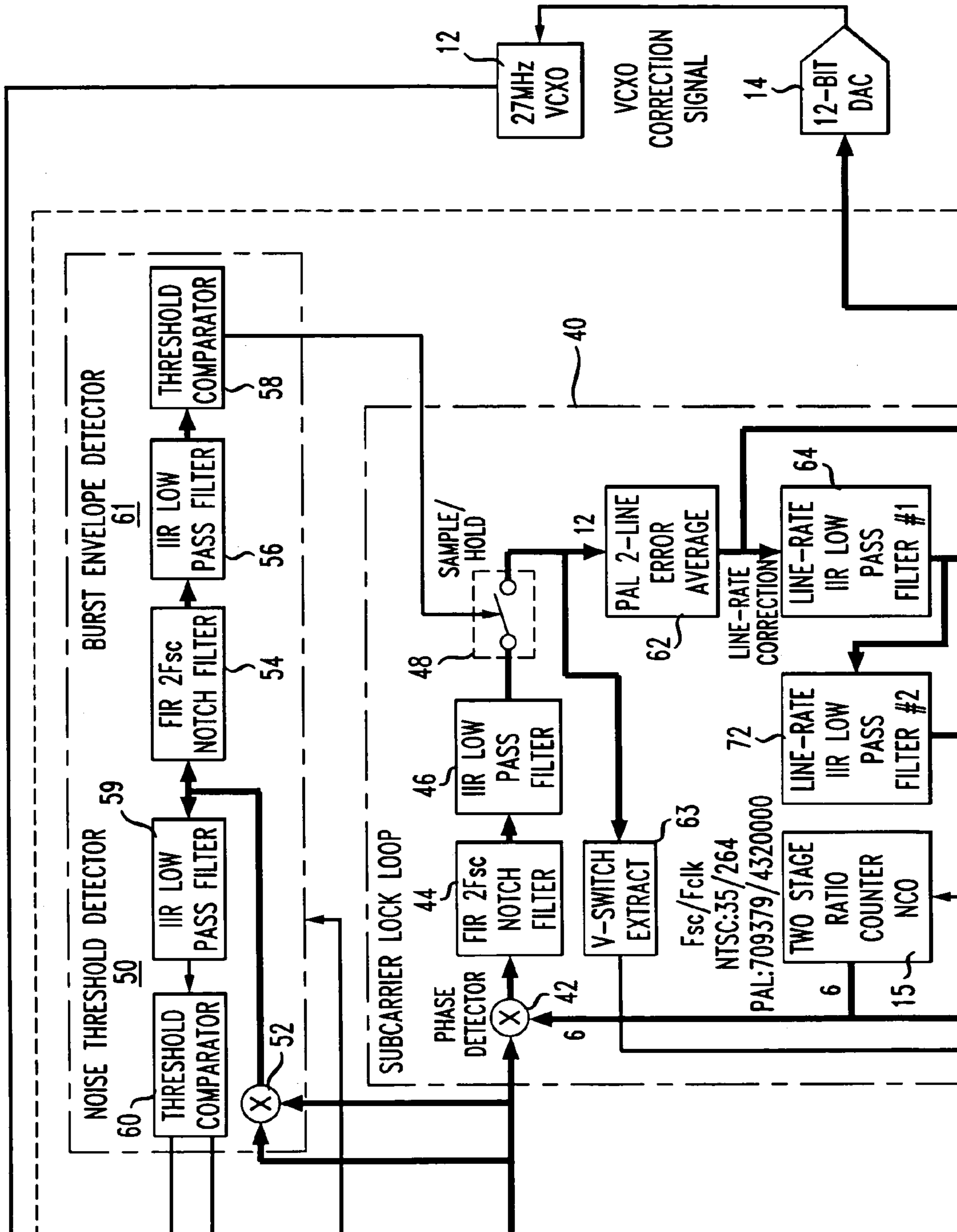
DIGITAL GENLOCK BLOCK DIAGRAM 10
