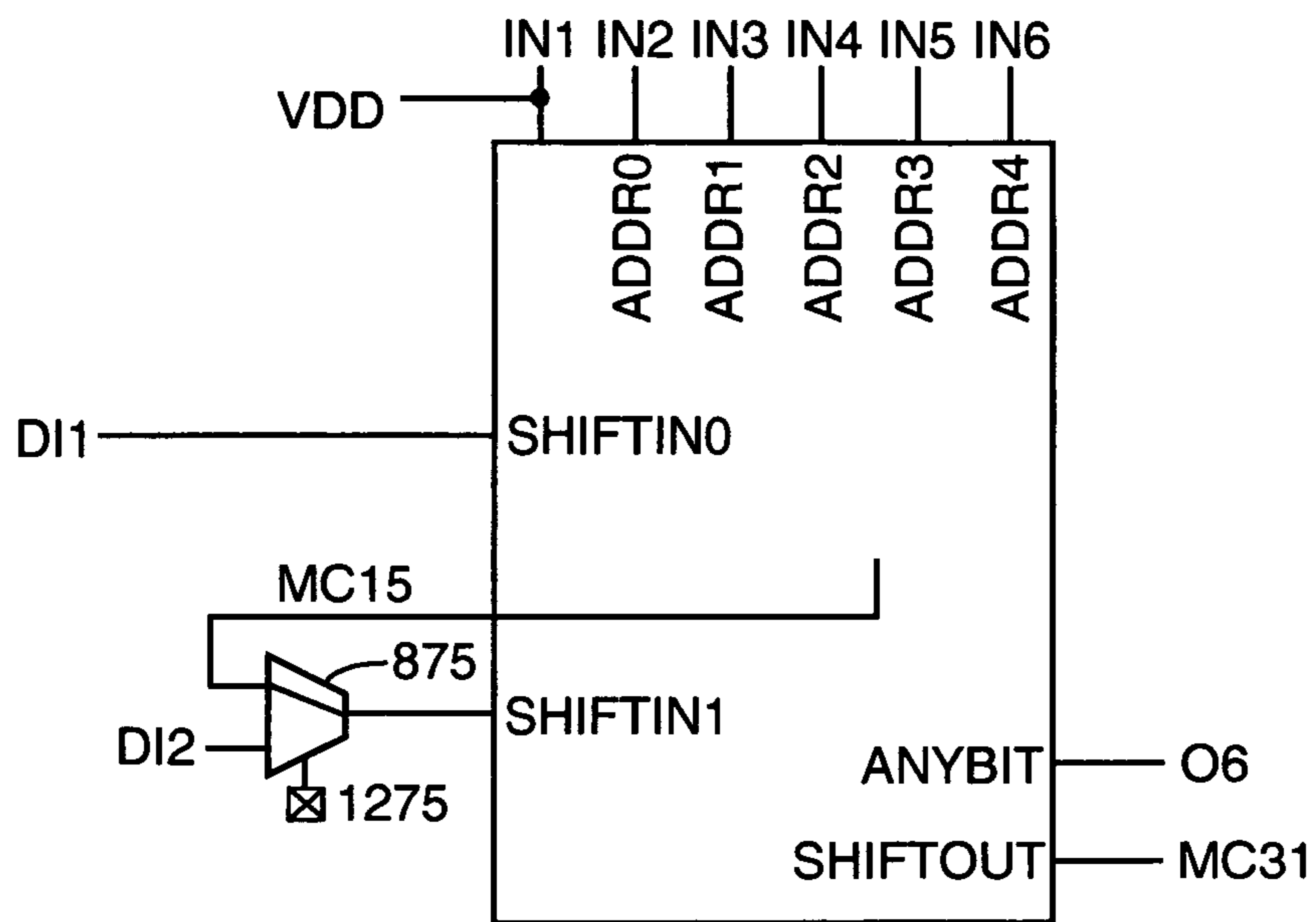
FIG. 12 (32x1 SRL)
